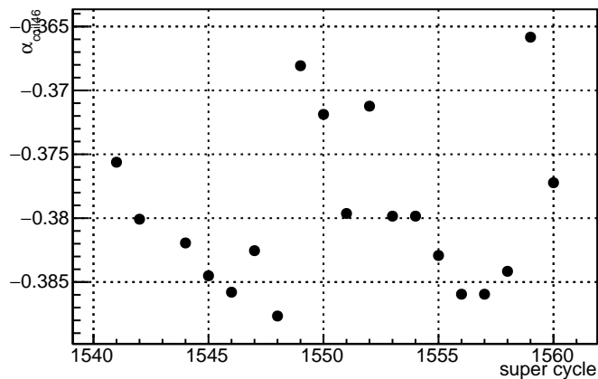
\alpha_{\text{coil46}}\text{-slug31}
