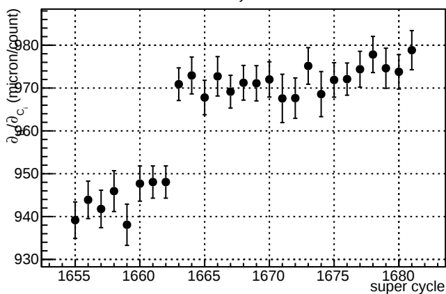
\partial B_{4ay}/\partial C_6
