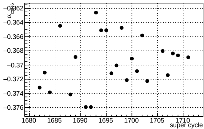
\alpha_{\text{coil46}} —slug35
