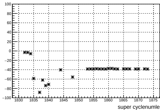
usr_11X12X : slug 39
