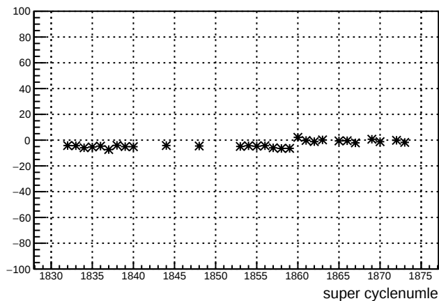
usr_11X12X : slug 39
