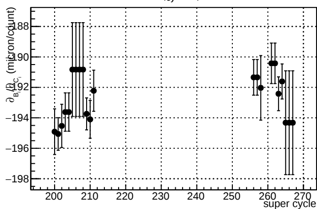
\partial B_{4ey}/\partial C_4
