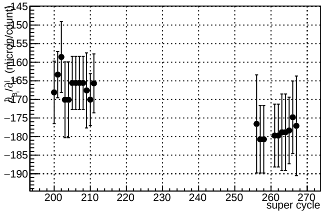
\partial B_{4ex}/\partial C_7
