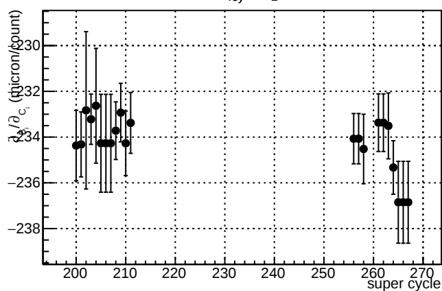
\partial B_{4ey}/\partial C_2
