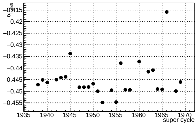
\alpha_{\text{coil46}} - \text{slug42}
