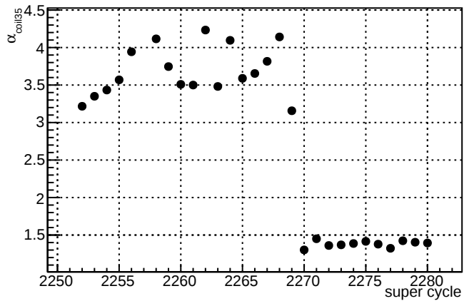
\alpha_{\text{coil35}} slug47
