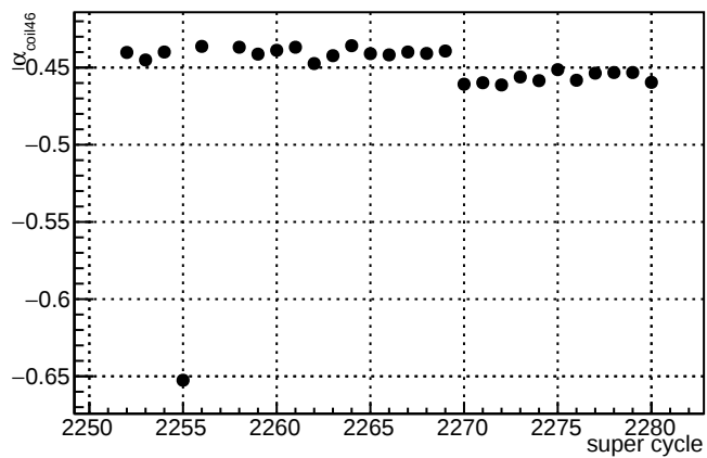
\alpha_{\text{coil46}} - \text{slug47}
