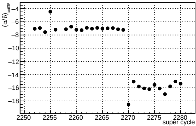
(\delta/\alpha)_{\text{coil35}}
