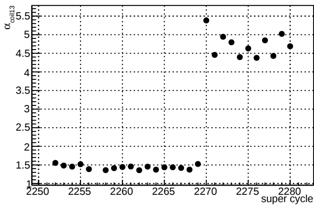
\alpha_{\text{coil13}} - \text{slug47}
