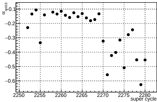
\alpha_{\text{coil15}} - \text{slug47}
