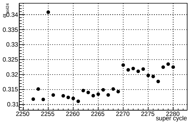
\alpha_{\text{coil24}} slug47
