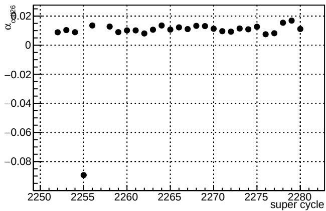
\alpha_{\text{coil26}} - \text{slug47}
