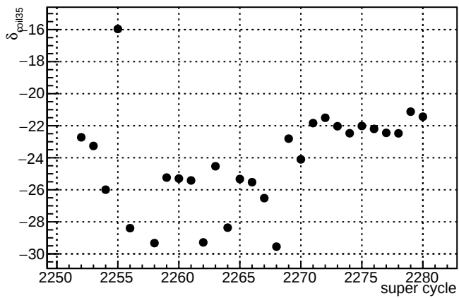
\delta_{\text{coil35}}
