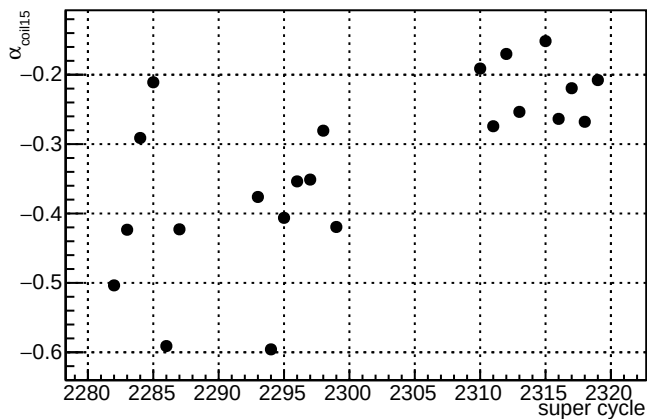
\alpha_{\text{coil15}} slug48
