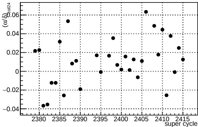
(\delta/\alpha)_{\text{coil24}}
