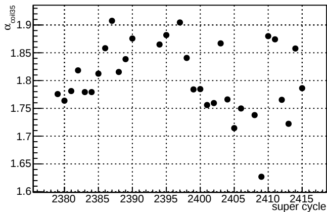
\alpha_{\text{coil35}} - \text{slug50}
