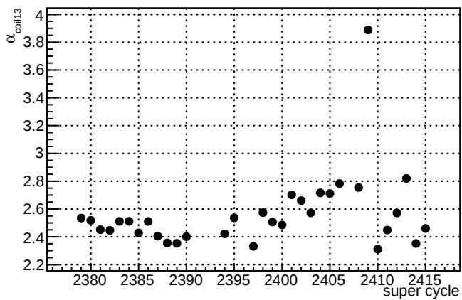
\alpha_{\text{coil13}} - \text{slug50}
