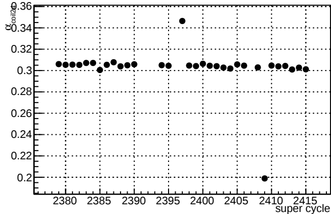
\alpha_{\text{coil24}} - \text{slug50}
