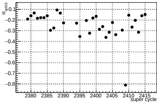
\alpha_{\text{coil15}} - \text{slug50}
