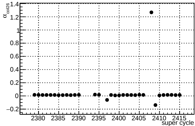
\alpha_{\text{coil26}} - \text{slug50}
