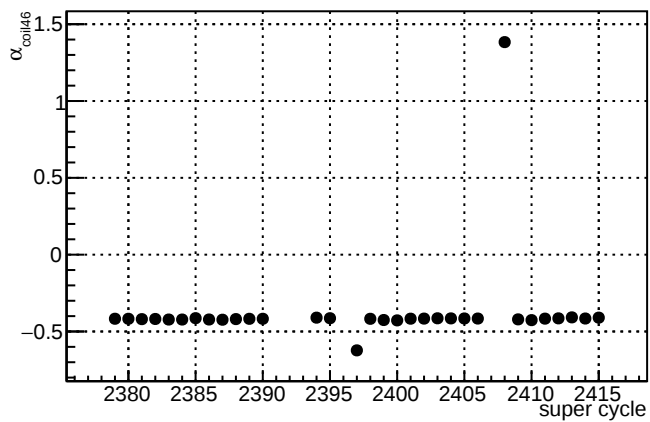
\alpha_{\text{coil46}} - \text{slug50}
