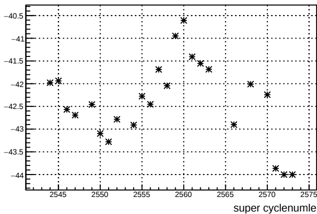
avg_ds_11X12X : slug 55
