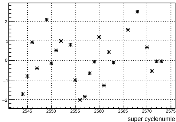
avg_us_11X12X : slug 55
