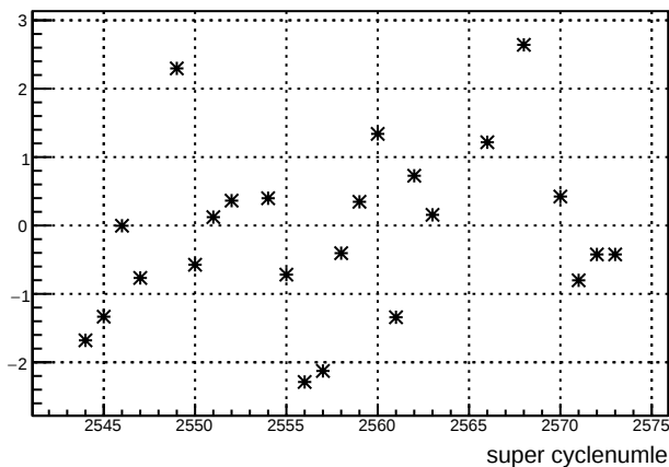
avg_ds_11X12X : slug 55
