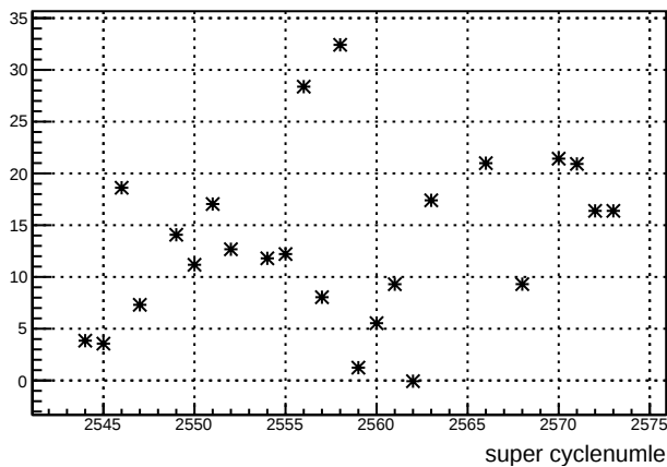
avg_ds_4ay : slug 55
