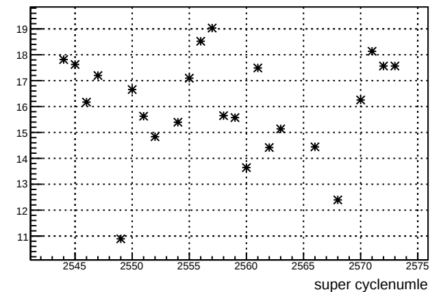
avg_ds_4ey : slug 55
