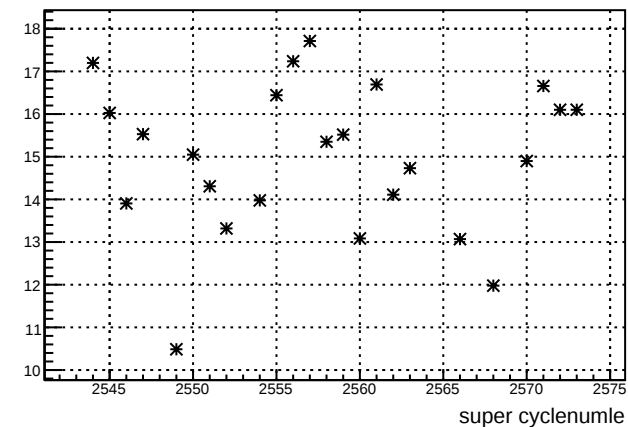
avg_us_4ey : slug 55
