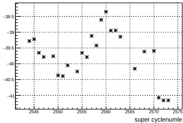
avg_us_11X12X : slug 55
