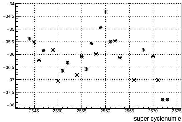
dsl_11X12X
