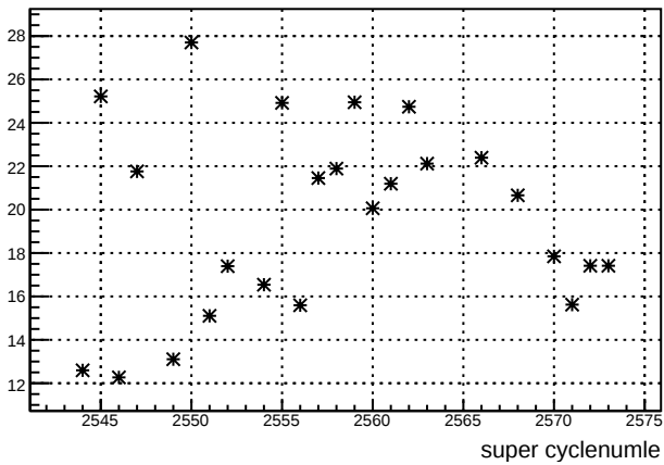
dd_ds_4ay : slug 55
