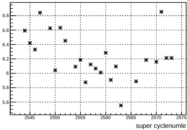
dd_ds_11X12X : slug 55
