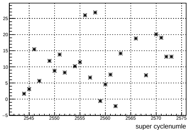
avg_us_4ay : slug 55
