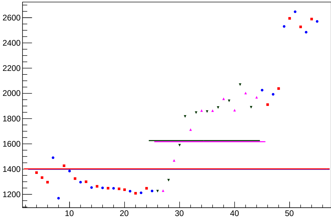
diff_bpm0l07Y_rms vs slug
