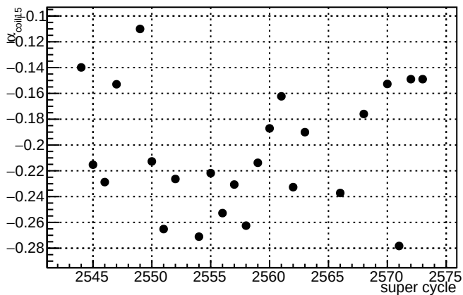
\alpha_{\text{coil15}} slug55
