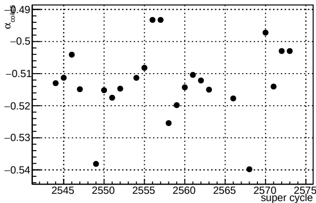
\alpha_{\text{coil46}} slug55
