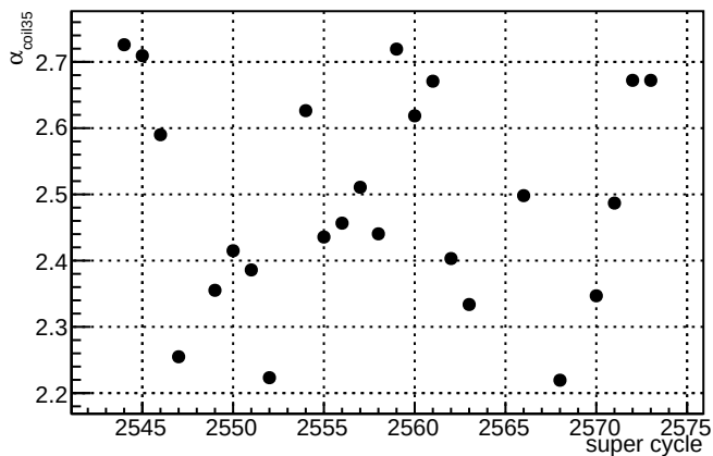
\alpha_{\text{coil35}} - \text{slug55}
