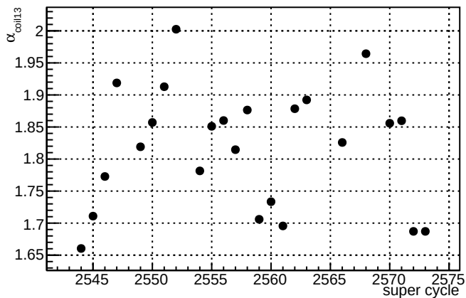
\alpha_{\text{coil13}} slug55
