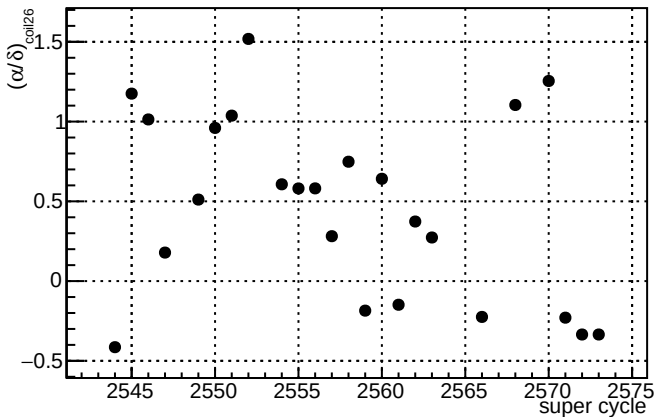
(\delta/\alpha)_{\text{coil26}}
