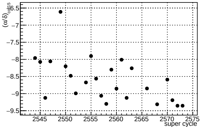
(\delta/\alpha)_{\text{coil15}}
