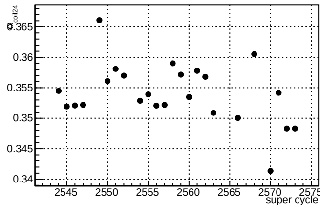
\alpha_{\text{coil24}} - \text{slug55}
