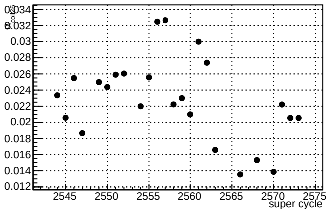
\alpha_{\text{coil26}} slug55
