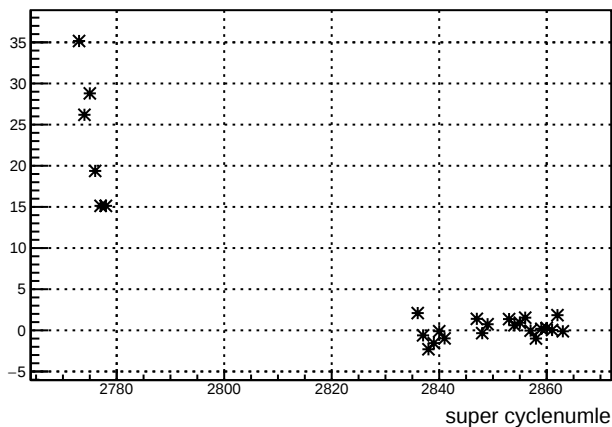
avg_ds_11X12X : slug 60
