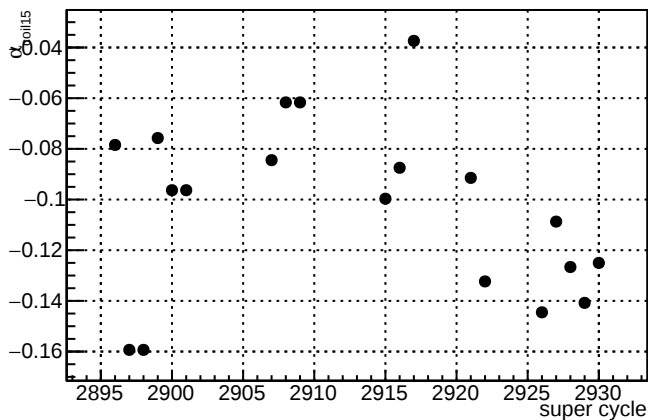
\alpha_{\text{coil15}} slug62
