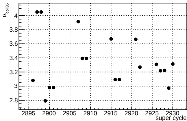
\alpha_{\text{coil35}} - \text{slug62}
