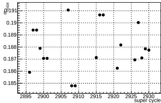
\alpha_{\text{coil24}} - \text{slug62}
