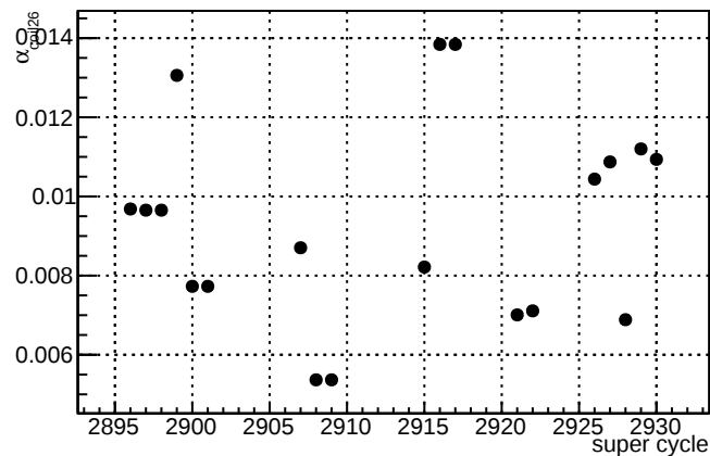
\alpha_{\text{coil26}} slug62
