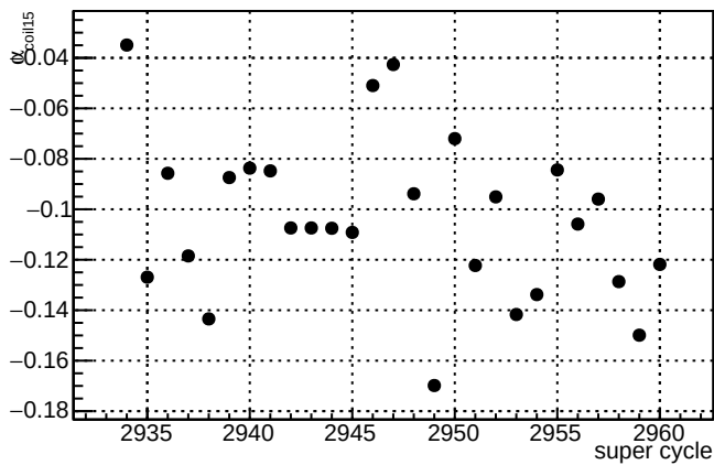
\alpha_{\text{coil15}} slug63
