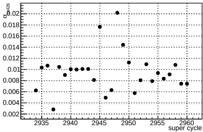
\alpha_{\text{coil26}} slug63
