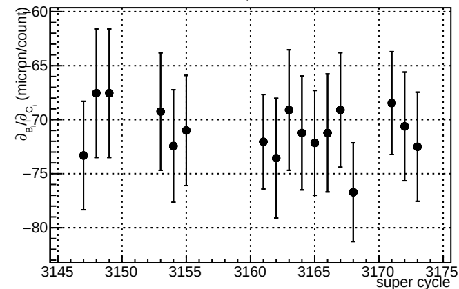
\partial B_{4ey}/\partial C_7
