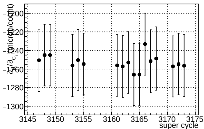
\partial B_{4ex}/\partial C_5
