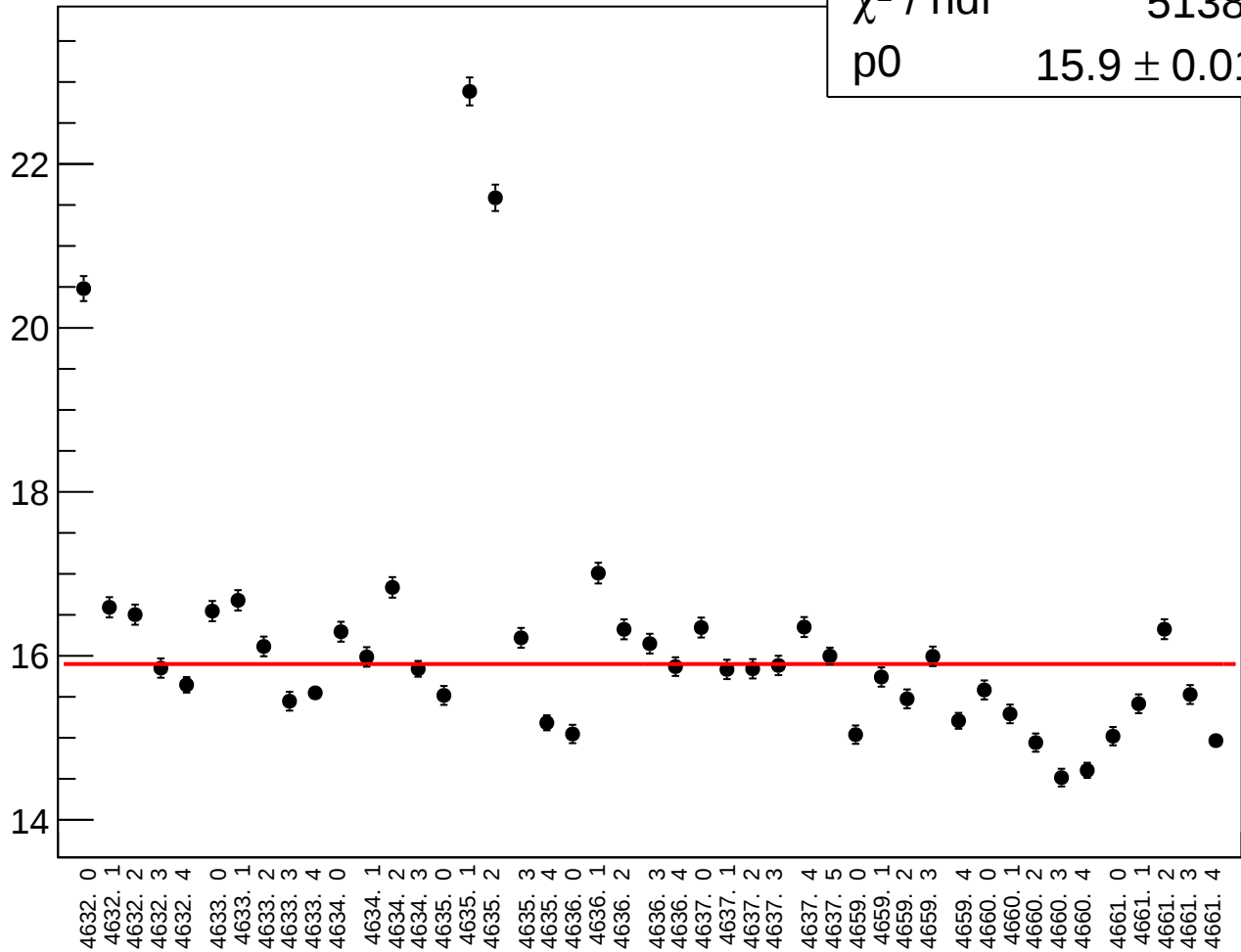
asym_bcm_dg_ds_bcm_an_us_agg_dd_rms vs run
