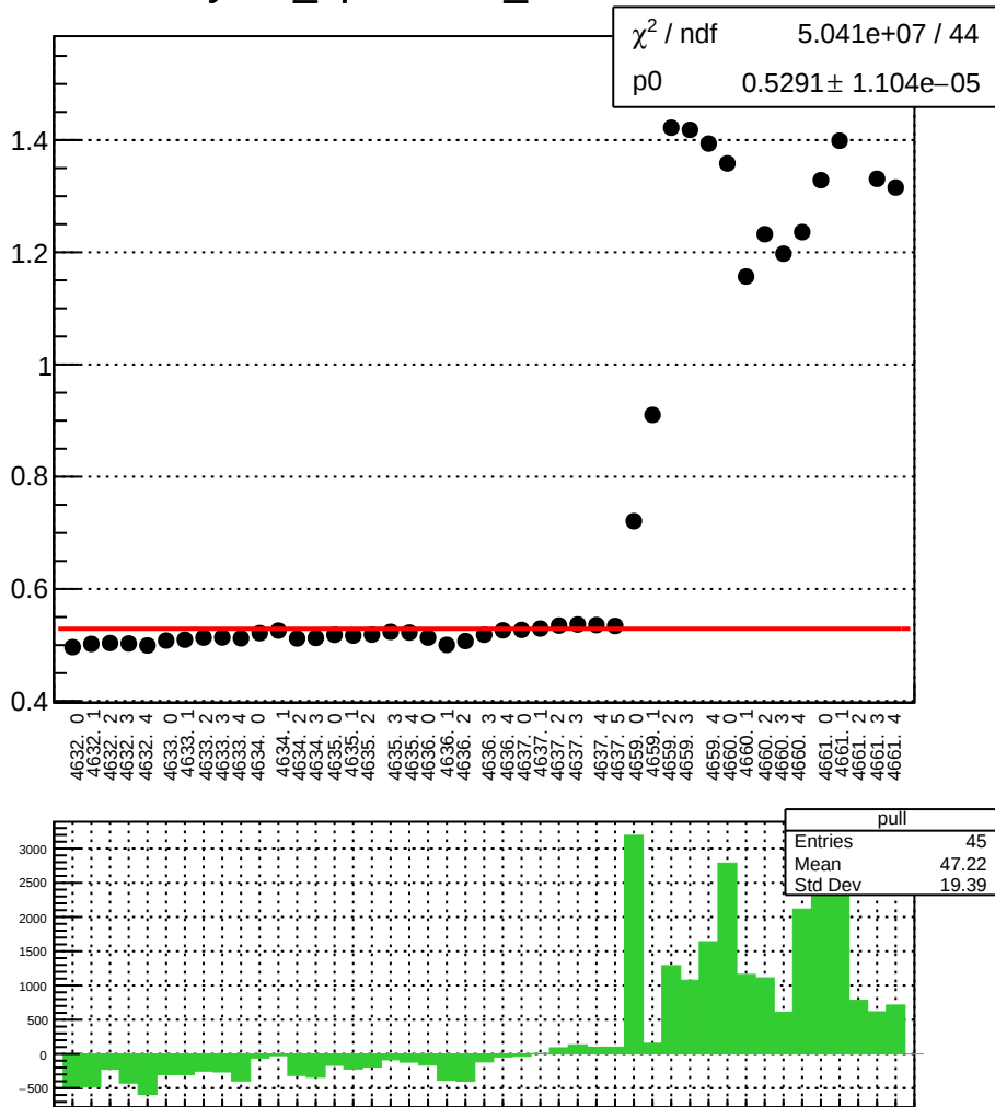
yield_bpm0l03Y_mean vs run
