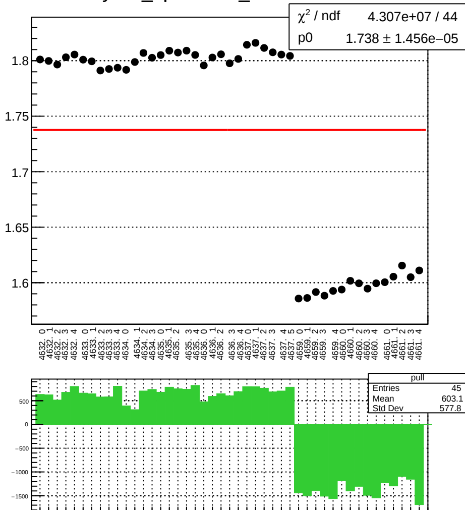
yield_bpm0l02Y_mean vs run
