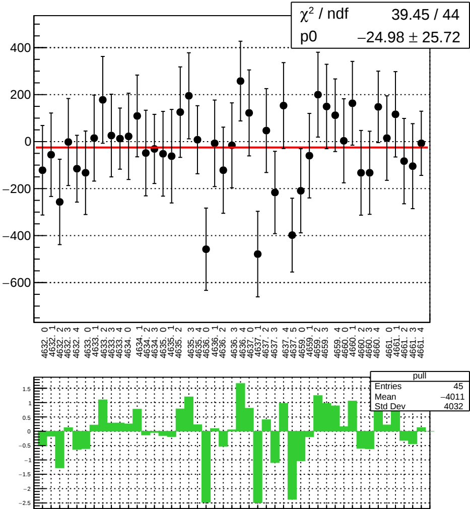
asym bcm an us ds3 avg bcm dg us agg dd mean vs run
