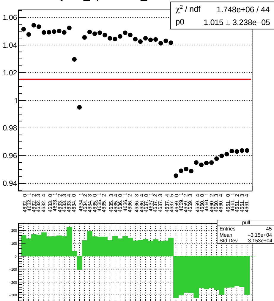
yield_bpm2i02X_mean vs run
