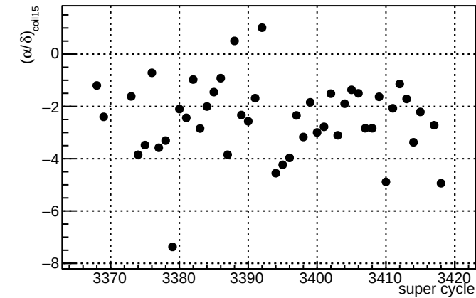
(\delta/\alpha)_{\text{coil15}}
