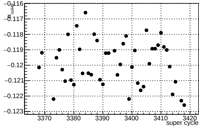
\alpha_{\text{coil46}} slug75
