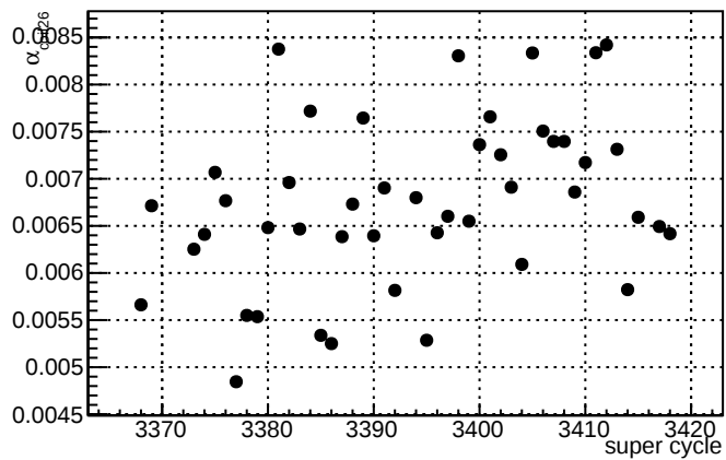
\alpha_{\text{coil26}} slug75
