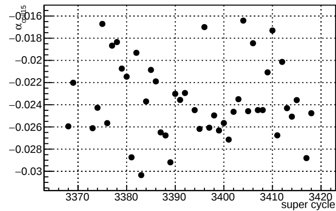
\alpha_{\text{coil15}} slug75
