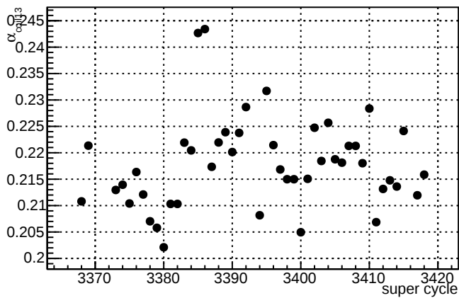
\alpha_{\text{coil13}} - \text{slug75}
