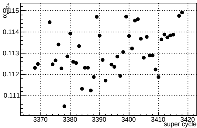
\alpha_{\text{coil24}} - \text{slug75}
