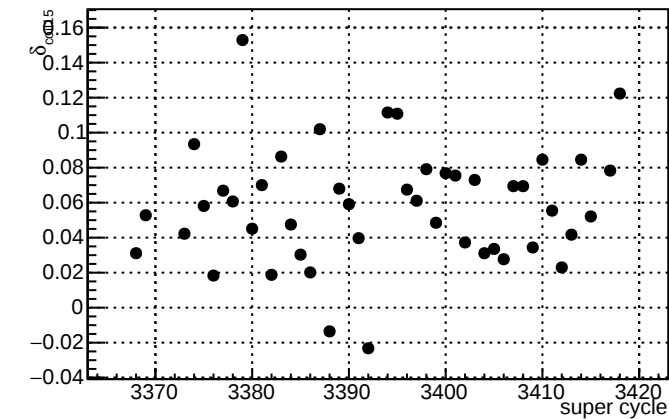
\delta_{\text{coil15}}
