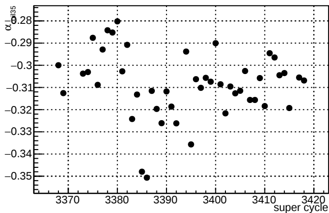
\alpha_{\text{coil35}} slug75
