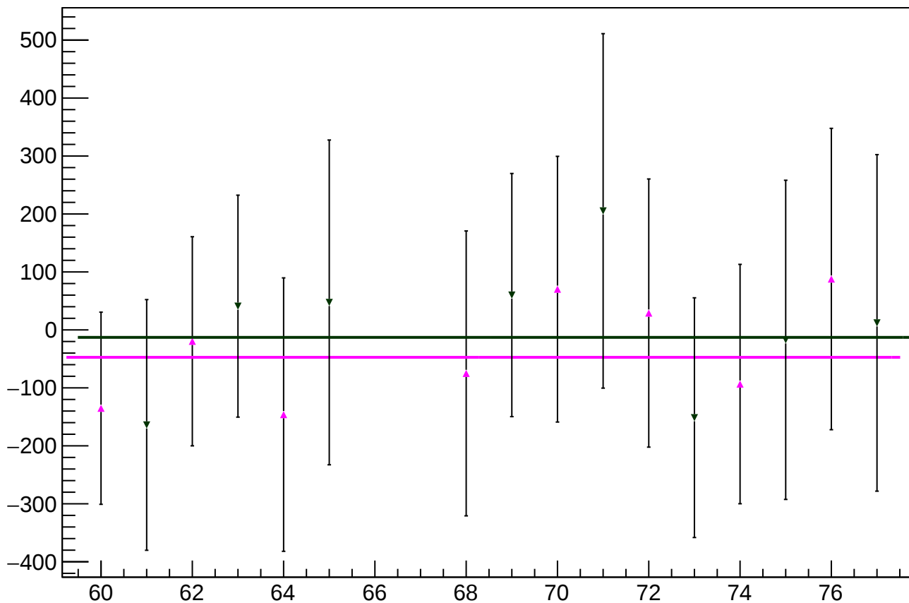
asym_bcm_dg_us_mean vs slug
