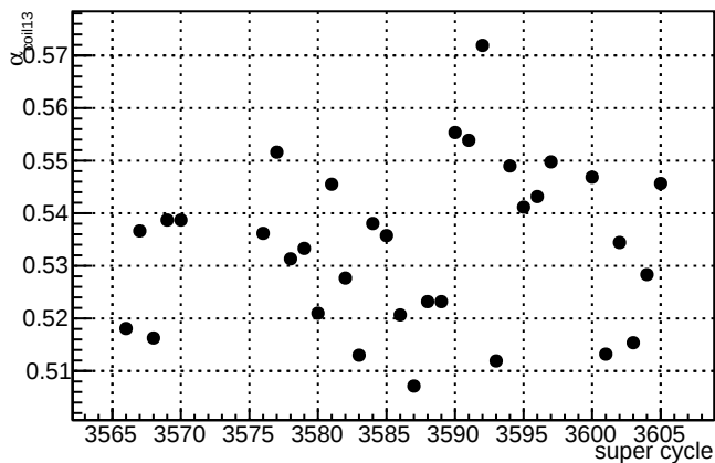
\alpha_{\text{coil13}} slug79
