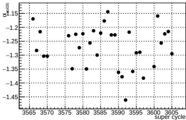
\alpha_{\text{coil35}} slug79
