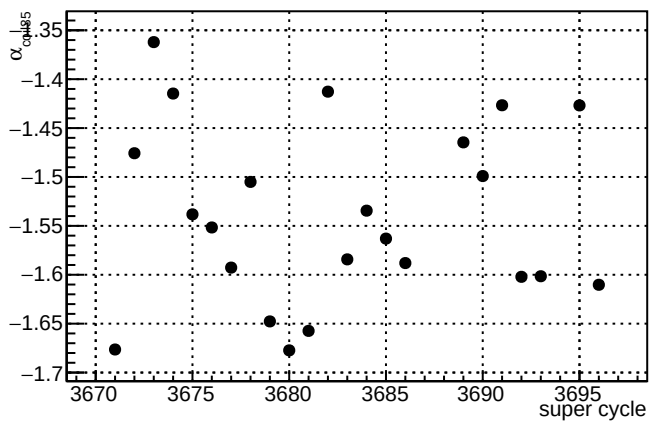
\alpha_{\text{coil35}} slug82
