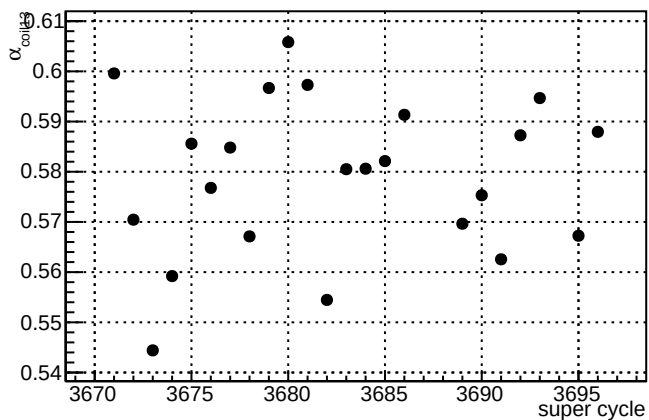
\alpha_{\text{coil13}} - \text{slug82}
