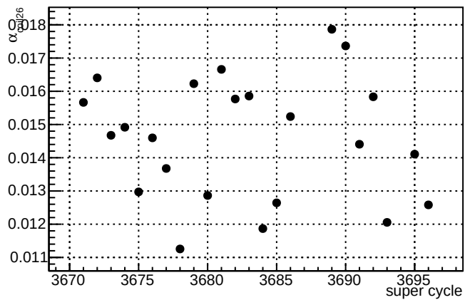
\alpha_{\text{coil26}} slug82
