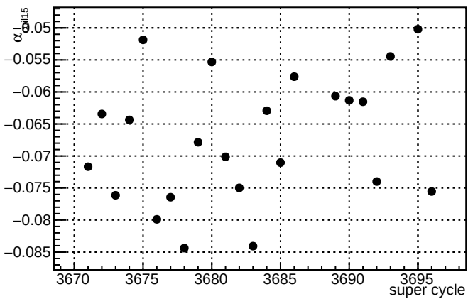
\alpha_{\text{coil15}} slug82
