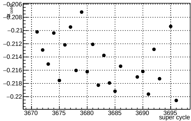
\alpha_{\text{coil46}} slug82
