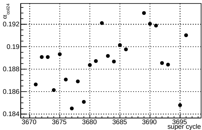
\alpha_{\text{coil24}} - \text{slug82}
