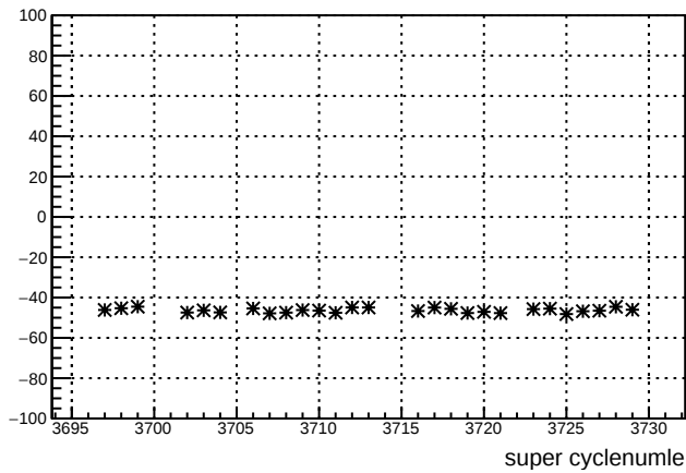
usr_11X12X : slug 83
