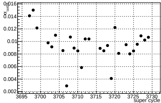
\alpha_{\text{coil26}} —slug83
