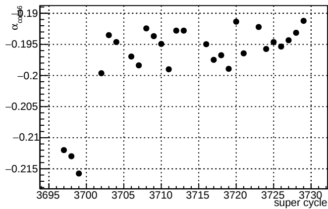
\alpha_{\text{coil46}} - \text{slug83}
