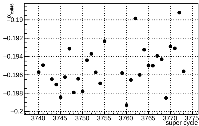
\alpha_{\text{coil46}} - \text{slug84}
