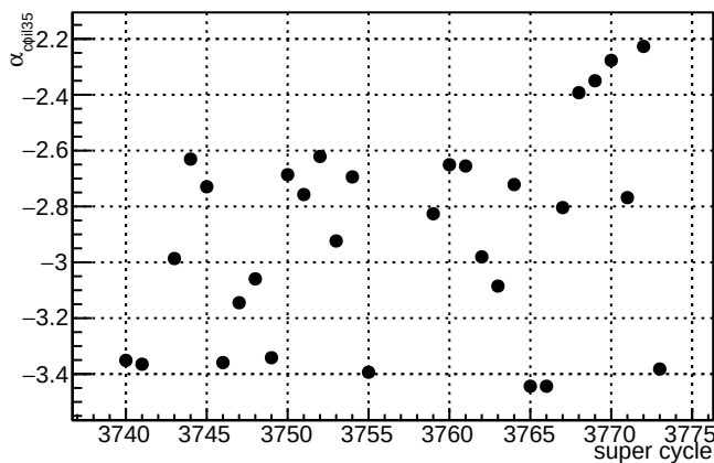
\alpha_{\text{coil35}} - \text{slug84}
