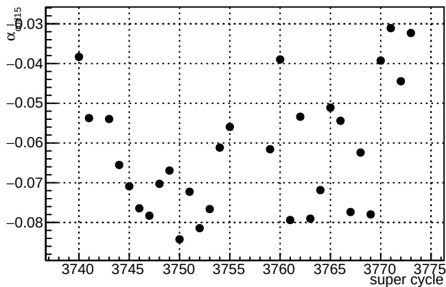
\alpha_{\text{coil15}} —slug84
