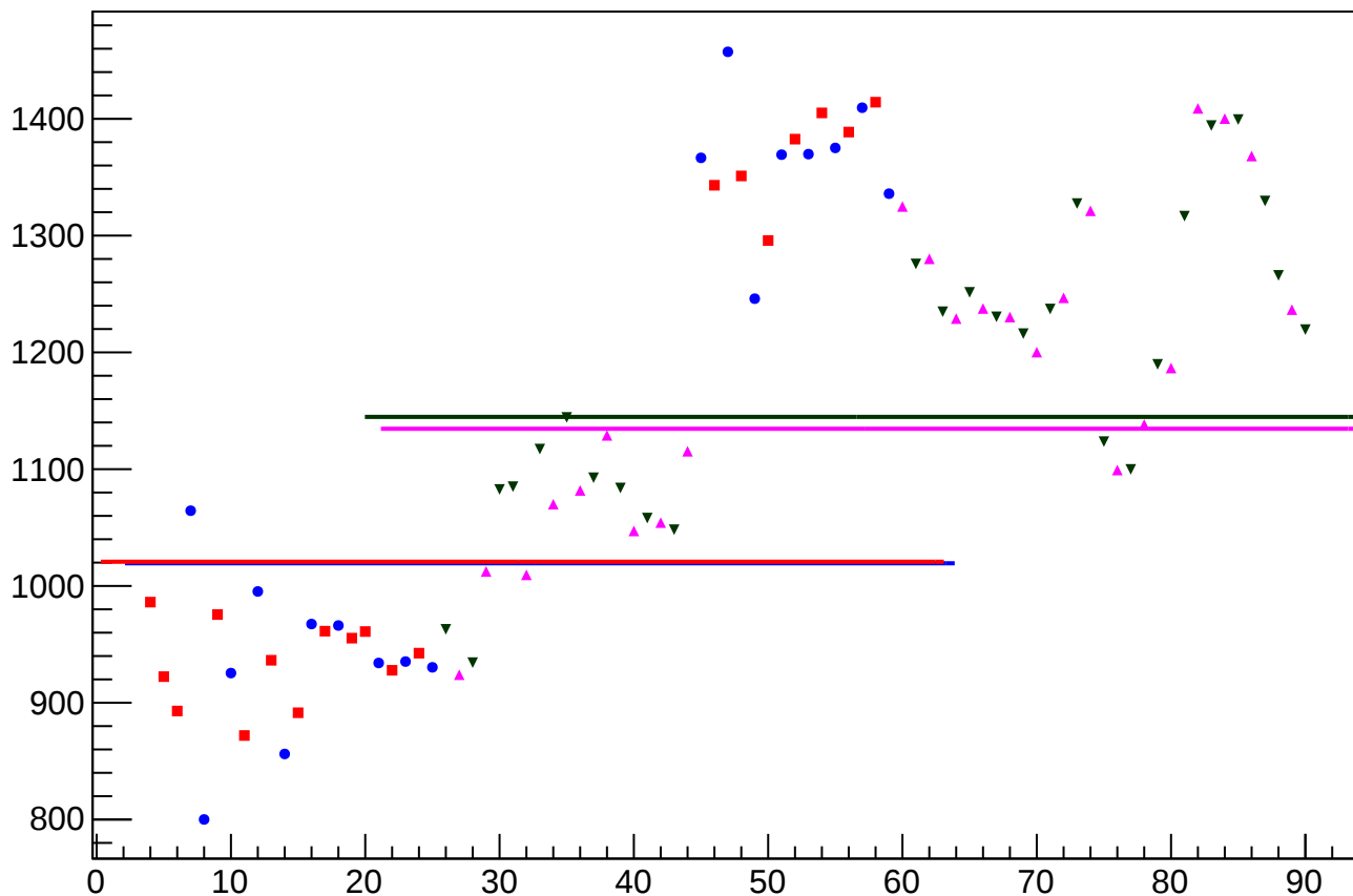
diff_bpm2i01X_rms vs slug
