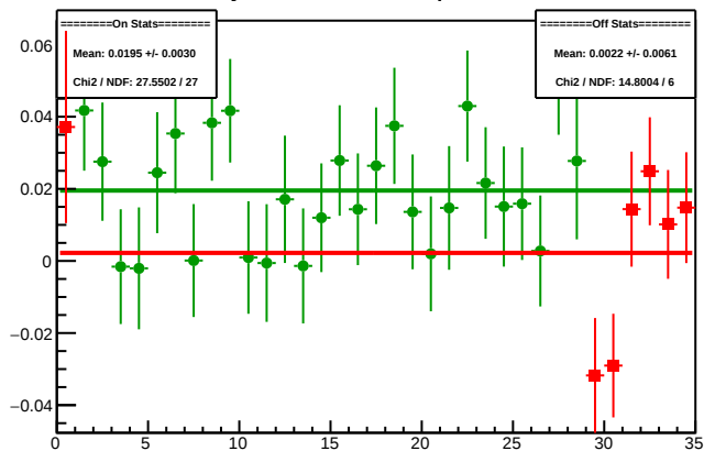
Cycle 4300.7: Multiplet Diffs
