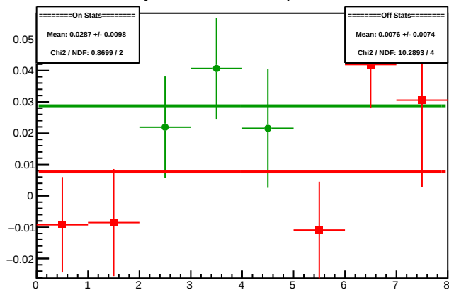
Cycle 4300.10: Multiplet Diffs
