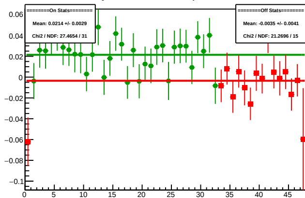
Cycle 4300.3: Multiplet Diffs
