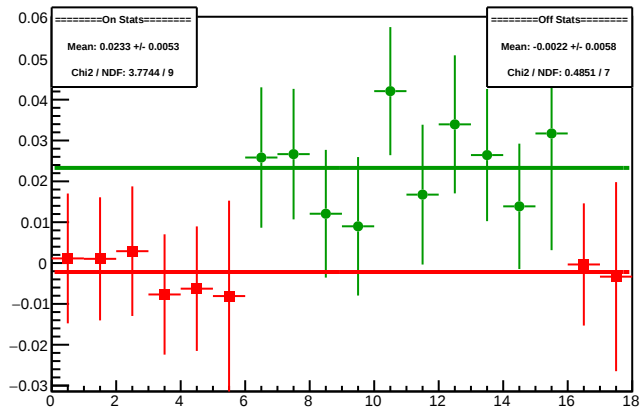
Cycle 4300.1: Multiplet Diffs
