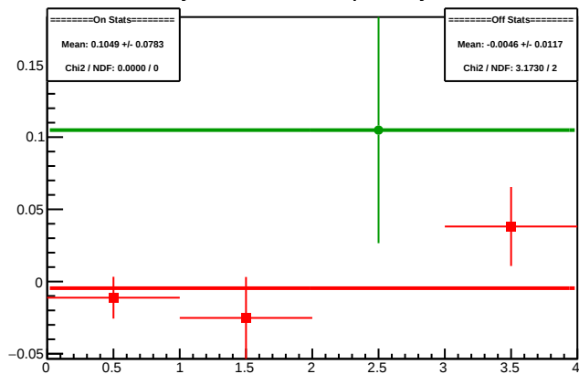
Cycle 4300.6: Multiplet Asyms
