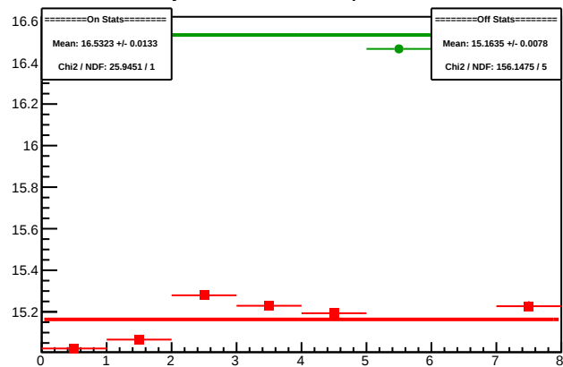
Cycle 4300.12: Multiplet Sums
