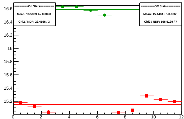
Cycle 4300.11: Multiplet Sums
