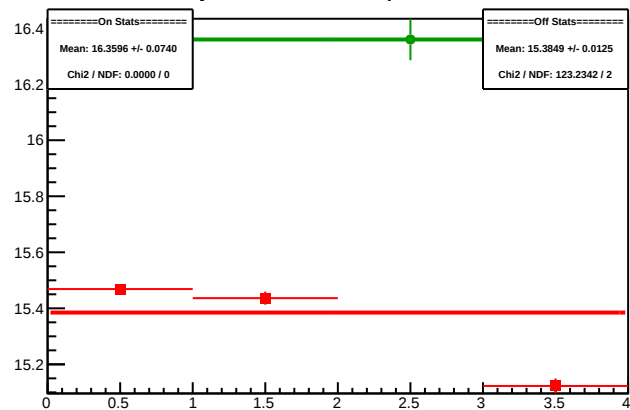
Cycle 4300.6: Multiplet Sums
