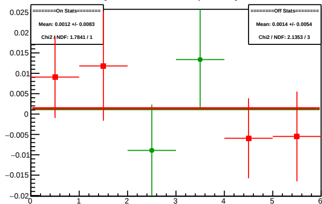
Cycle 4300.9: Multiplet Asyms
