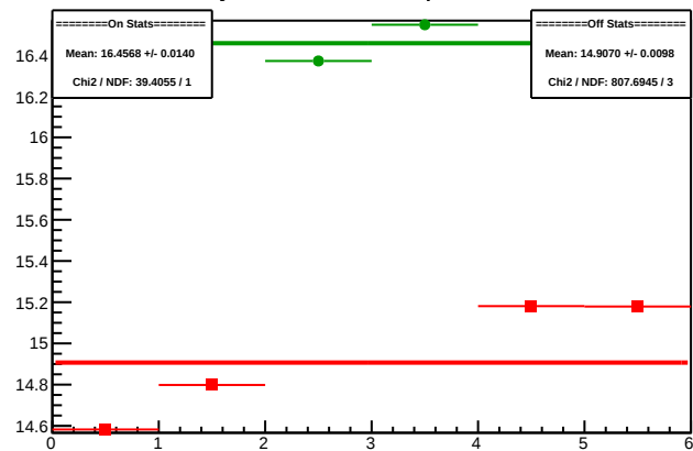
Cycle 4300.9: Multiplet Sums
