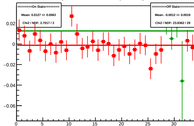
Cycle 4300.4: Multiplet Asyms
