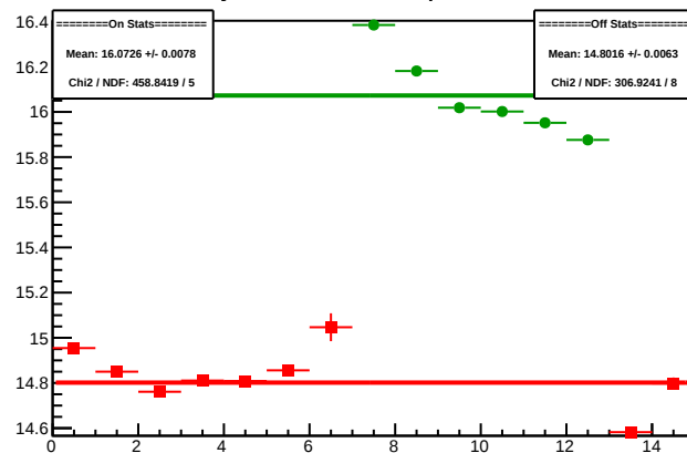
Cycle 4300.8: Multiplet Sums
