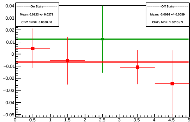
Cycle 4300.5: Multiplet Diffs
