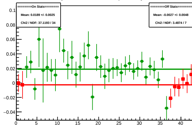
Cycle 4300.2: Multiplet Asyms
