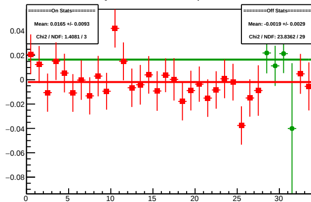
Cycle 4300.4: Multiplet Diffs
