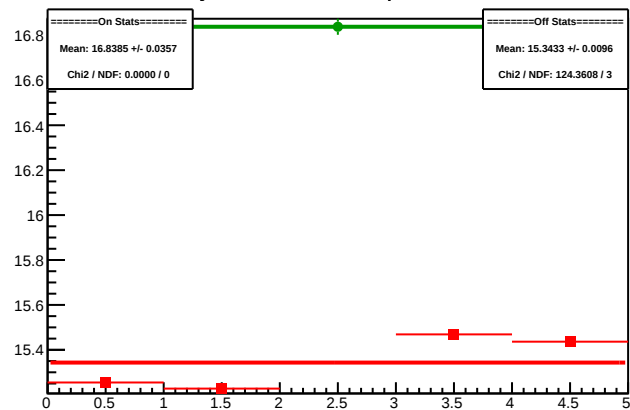
Cycle 4300.5: Multiplet Sums
