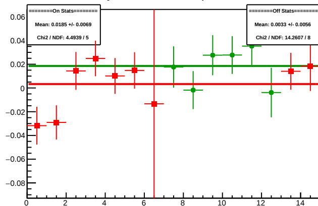
Cycle 4300.8: Multiplet Diffs
