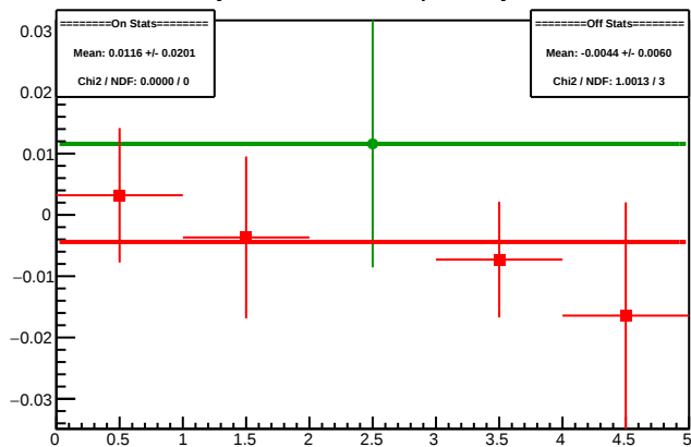
Cycle 4300.5: Multiplet Asyms
