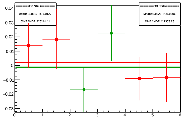
Cycle 4300.9: Multiplet Diffs
