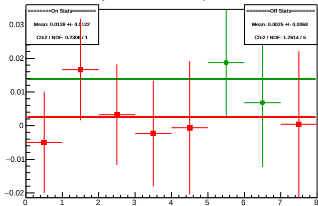
Cycle 4300.12: Multiplet Diffs
