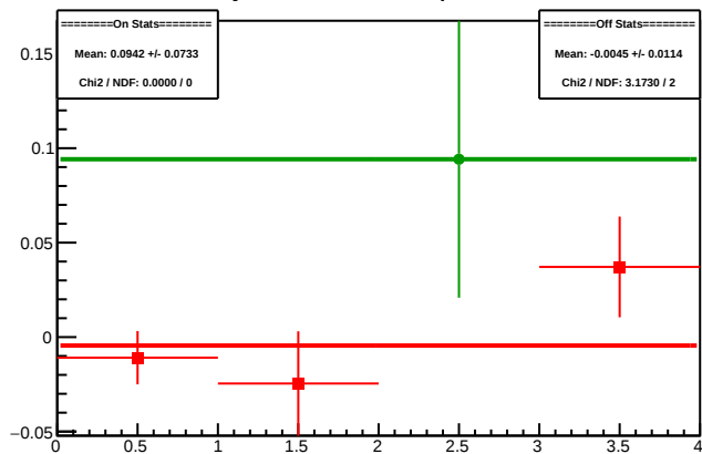
Cycle 4300.6: Multiplet Diffs
