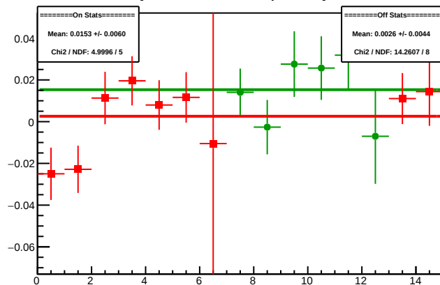
Cycle 4300.8: Multiplet Asyms
