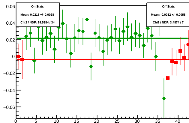
Cycle 4300.2: Multiplet Diffs
