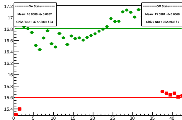
Cycle 4300.2: Multiplet Sums
