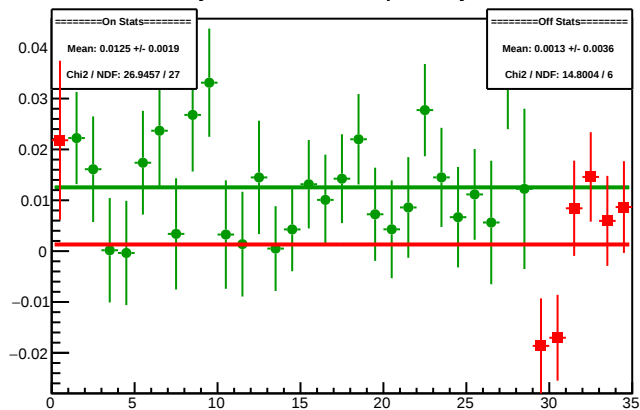
Cycle 4300.7: Multiplet Asyms
