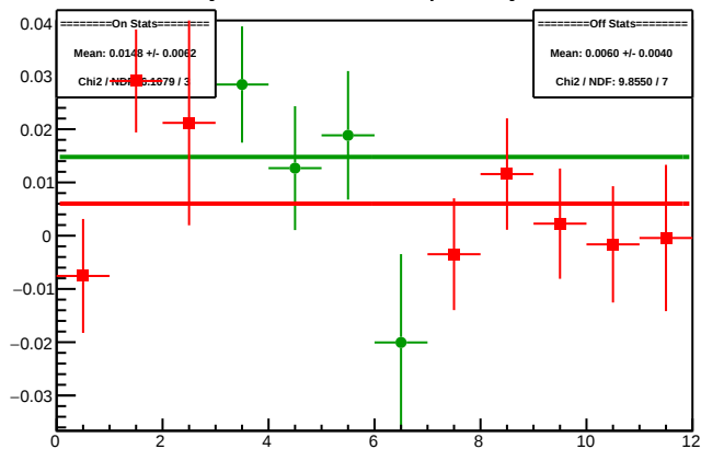
Cycle 4300.11: Multiplet Asyms
