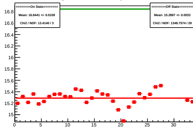
Cycle 4300.4: Multiplet Sums
