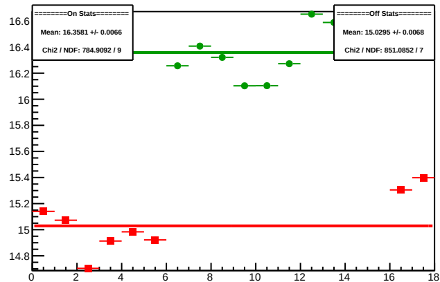
Cycle 4300.1: Multiplet Sums
