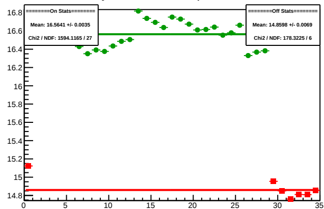
Cycle 4300.7: Multiplet Sums
