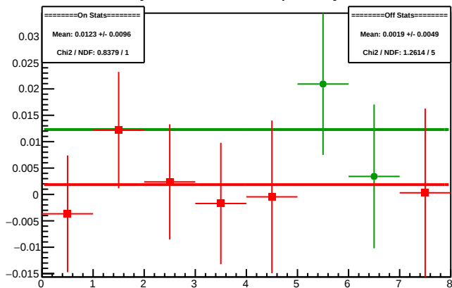
Cycle 4300.12: Multiplet Asyms
