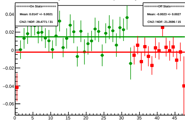
Cycle 4300.3: Multiplet Asyms
