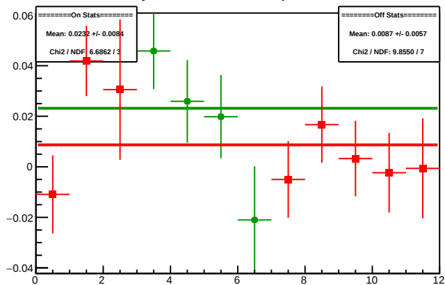
Cycle 4300.11: Multiplet Diffs
