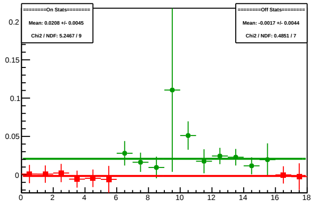
Cycle 4300.1: Multiplet Asyms
