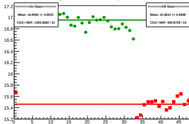
Cycle 4300.3: Multiplet Sums
