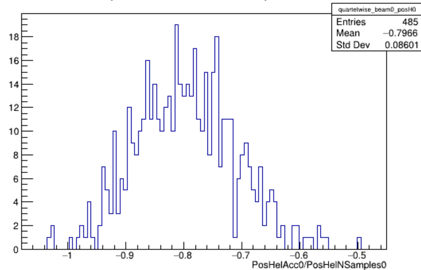
Run 4306 quartetwise, PosHelAcc0/NSamples0: Beam OFF
