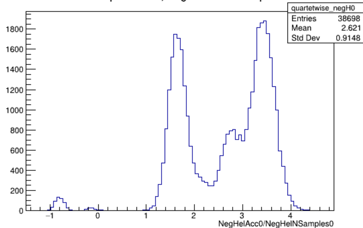
Run 4306 quartetwise, NegHelAcc0/NSamples0: All
