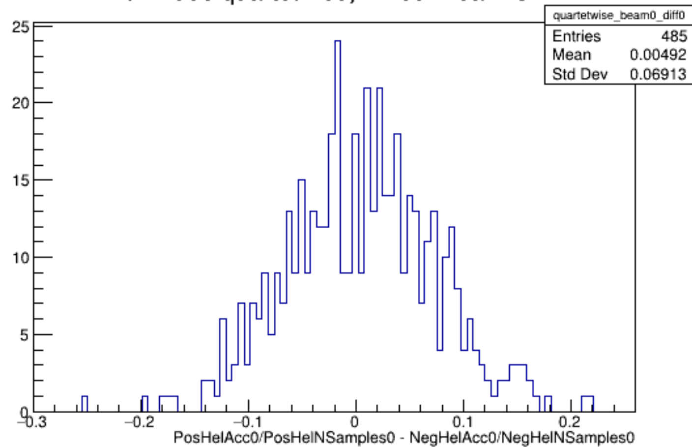
Run 4306 quartetwise, Diffs0: Beam OFF
