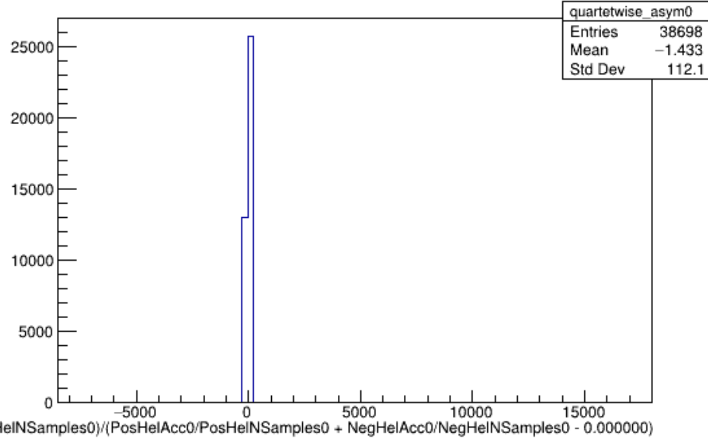
Run 4306 quartetwise, Asyms0 (Raw): All
