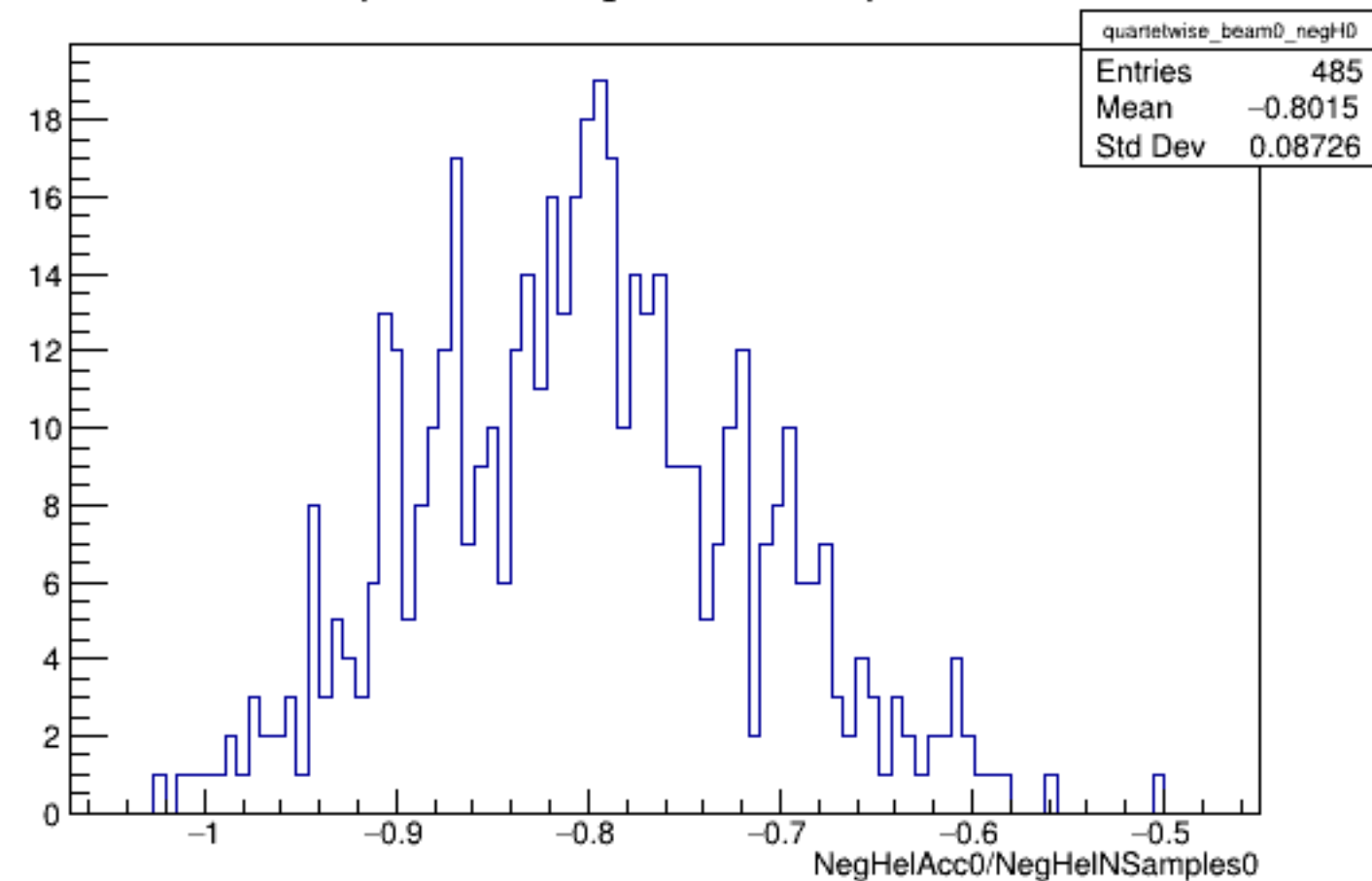
Run 4306 quartetwise, NegHelAcc0/NSamples0: Beam OFF
