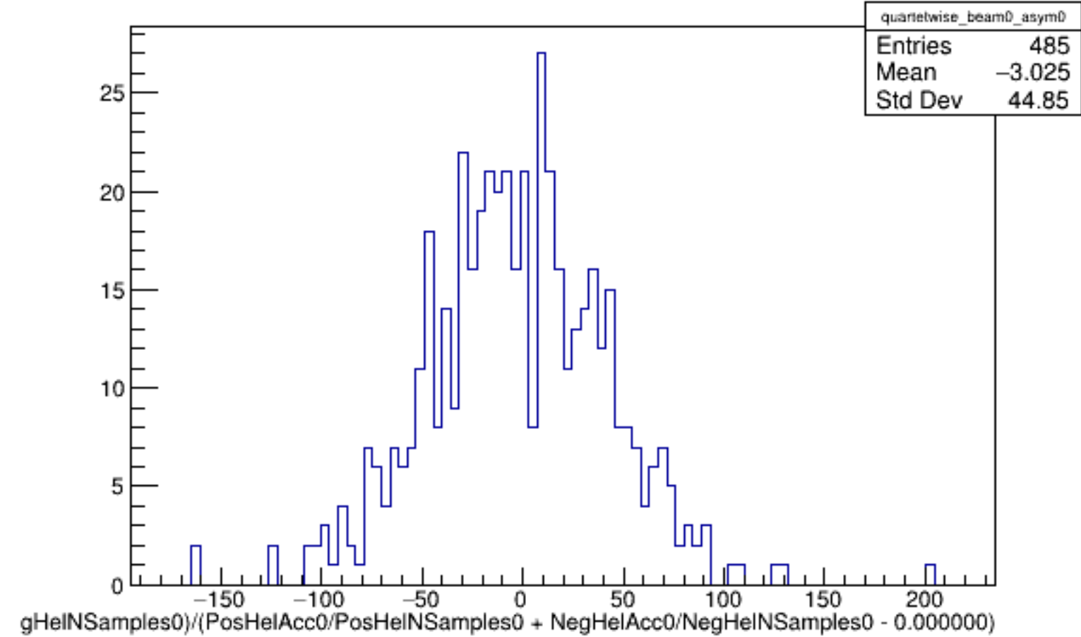
Run 4306 quartetwise, Asyms0 (Raw): Beam OFF
