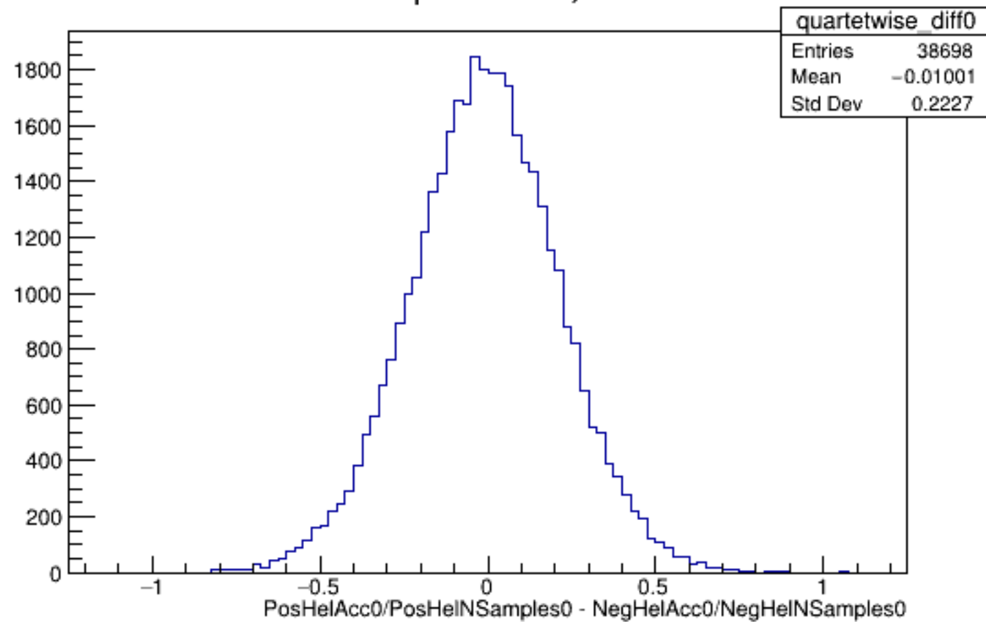
Run 4306 quartetwise, Diffs0: All
