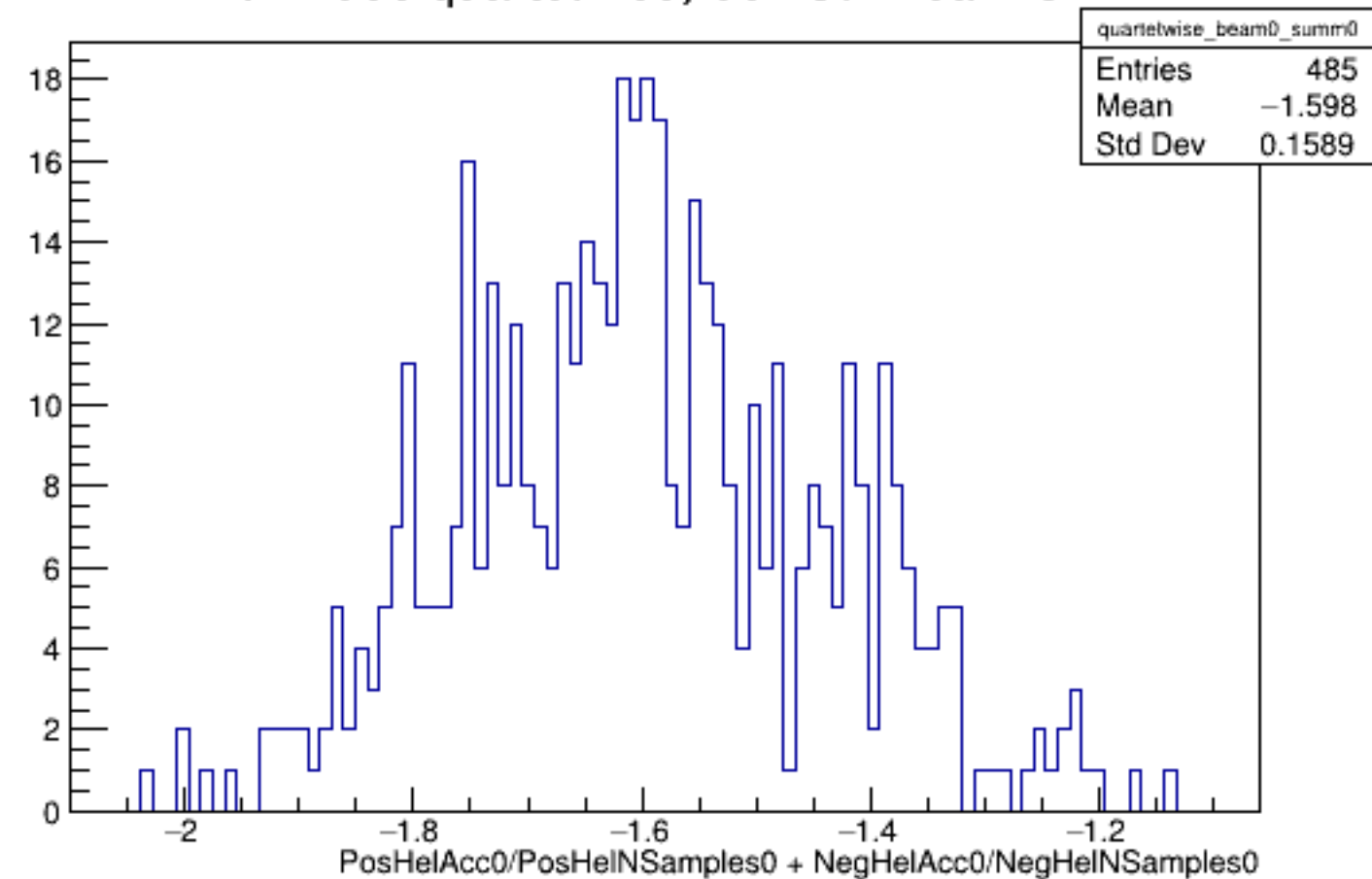
Run 4306 quartetwise, Sums0: Beam OFF
