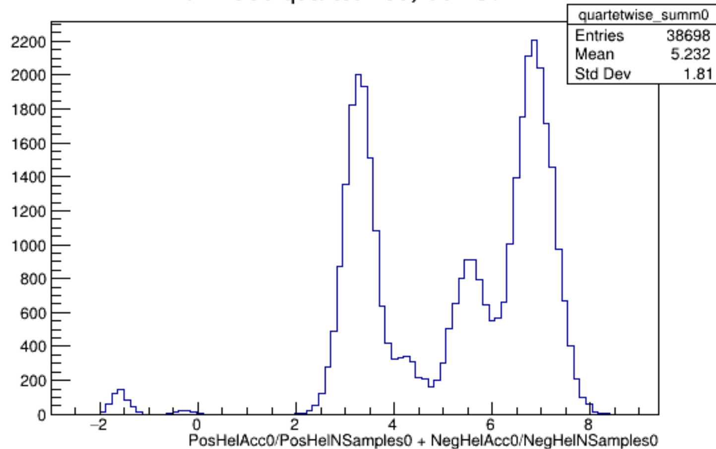
Run 4306 quartetwise, Sums0: All
