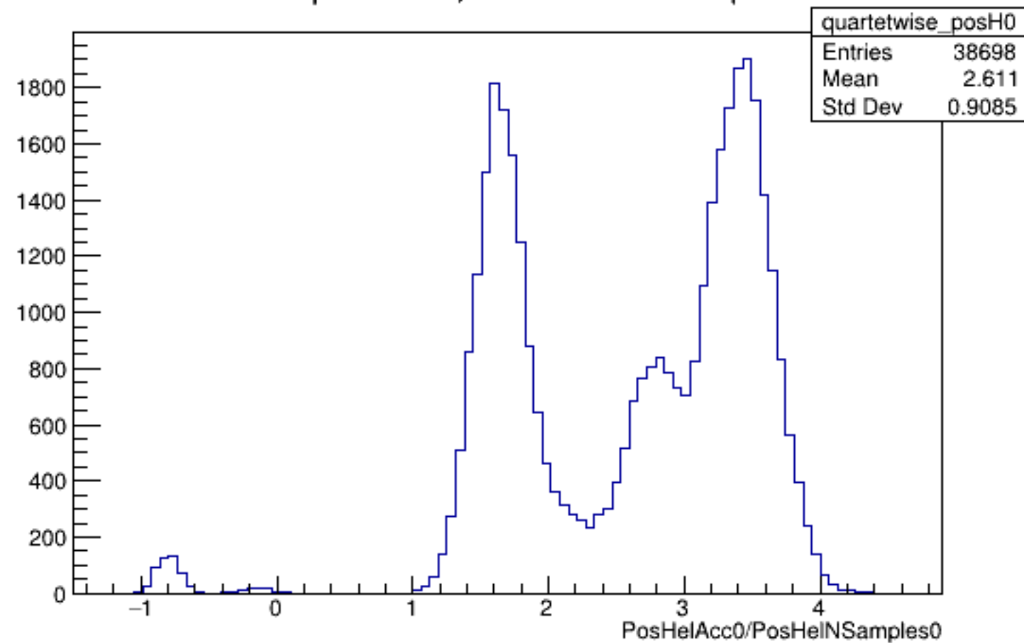
Run 4306 quartetwise, PosHelAcc0/NSamples0: All
