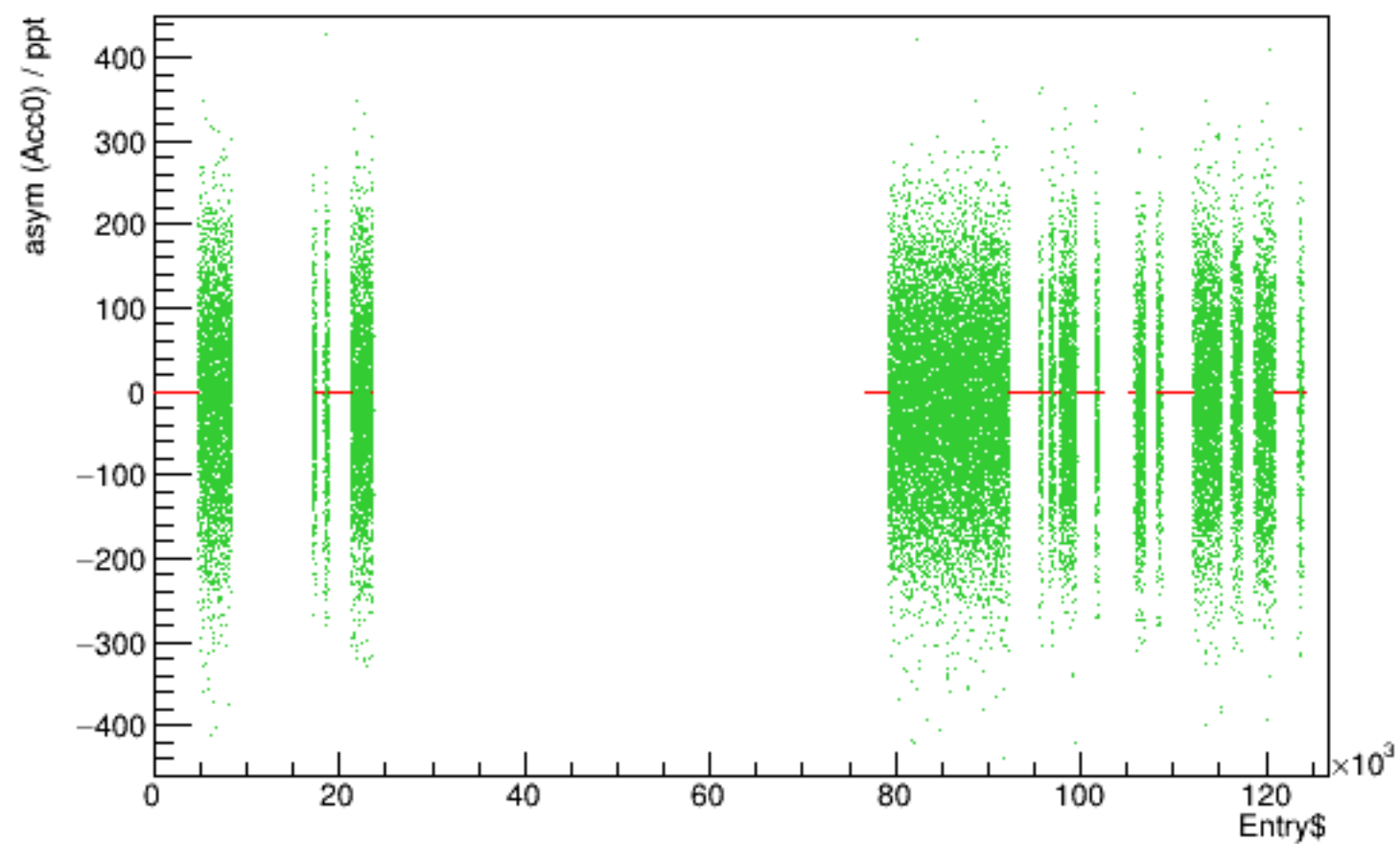
Run 4316 quartetwise, asym0sub vs time
