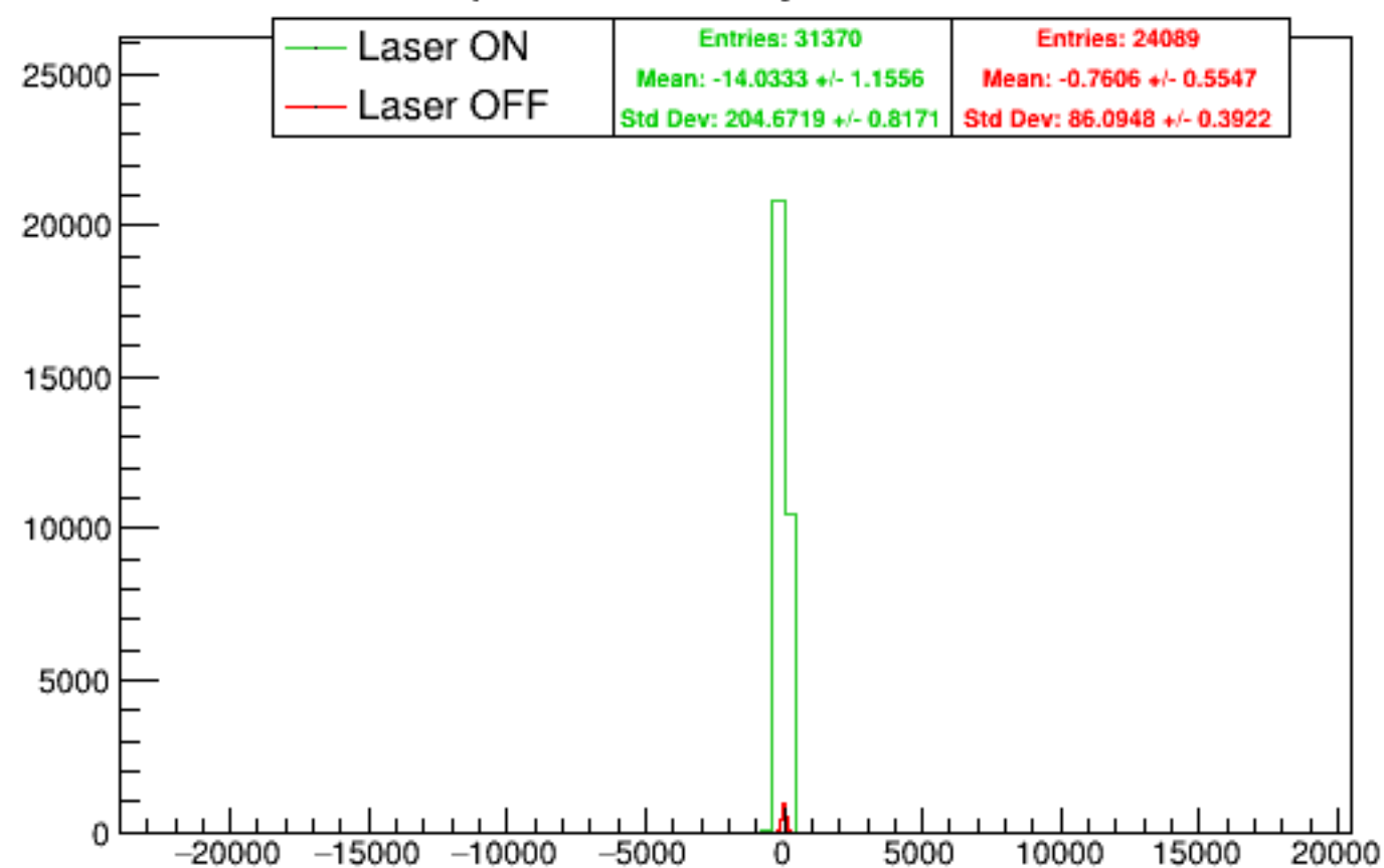
Run 4316 quartetwise, asym0sub: Beam ON
