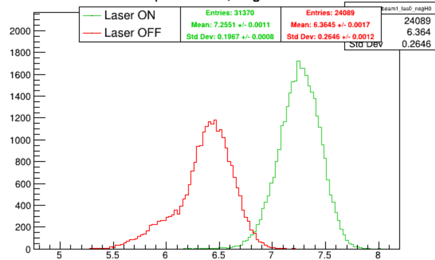
Run 4316 quartetwise, negH0: Beam ON
