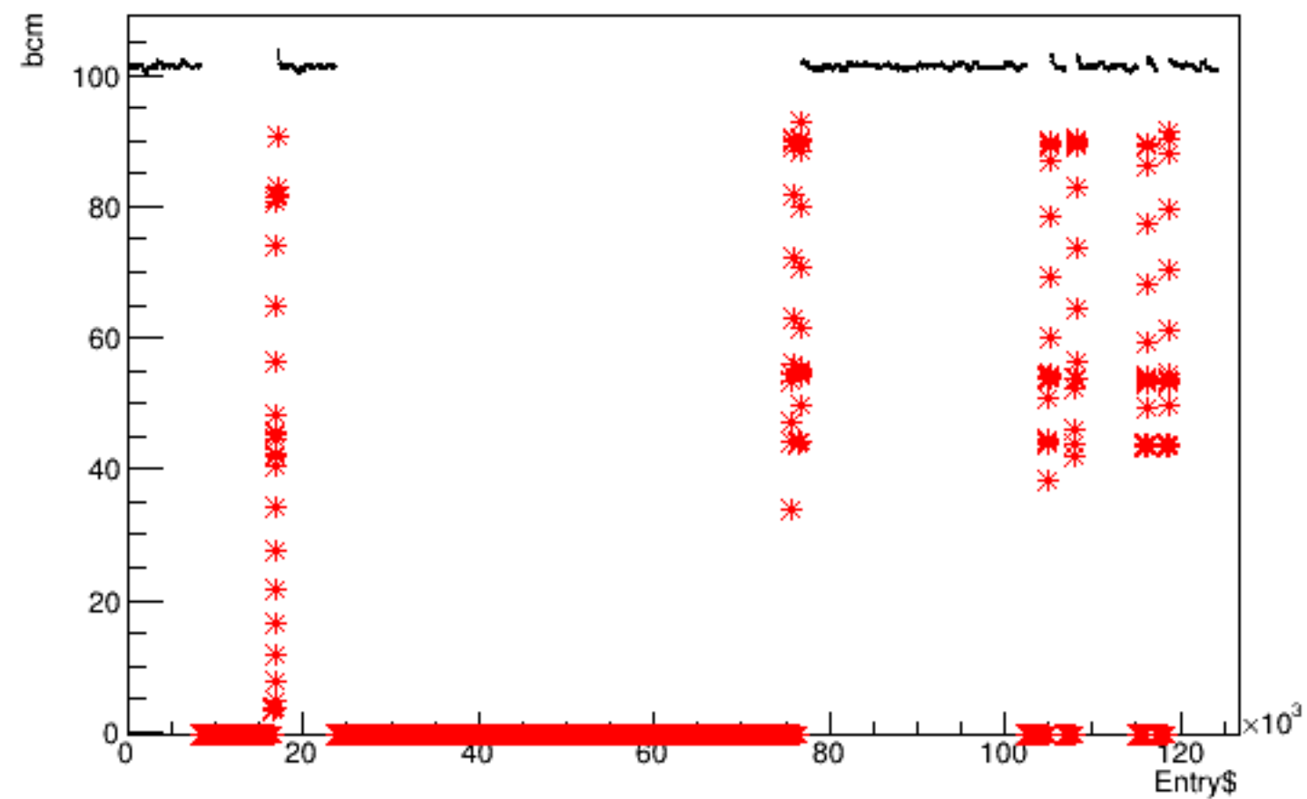
Run 4316 quartetwise, bcm vs time
