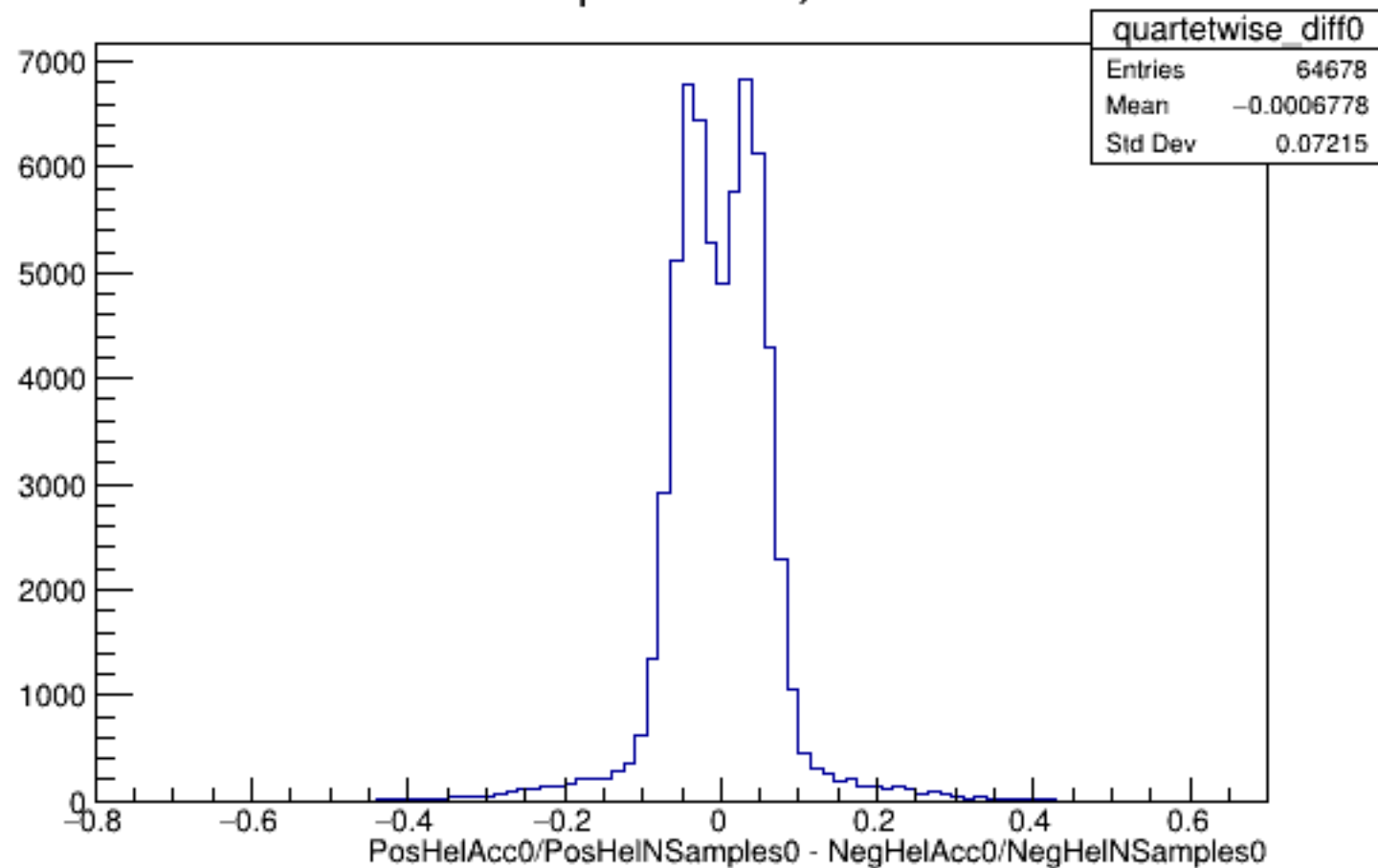
Run 4318 quartetwise, Diffs0: All
