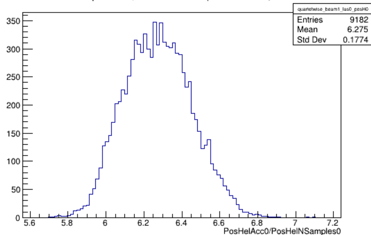
Run 4318 quartetwise, PosHelAcc0/NSamples0: Beam ON, Laser OFF
