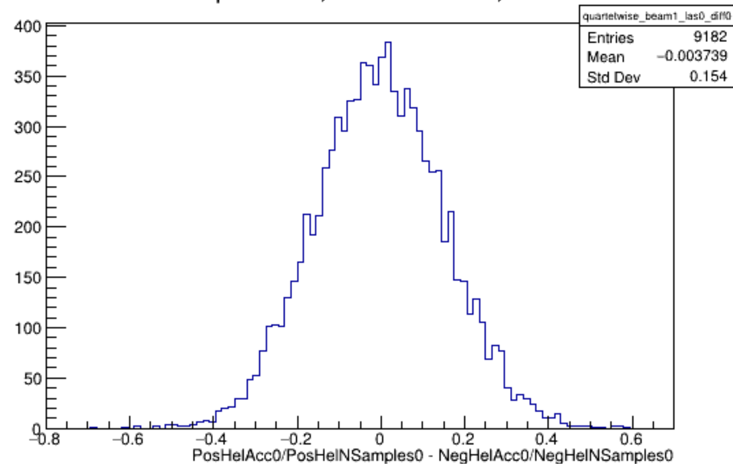
Run 4318 quartetwise, Diffs0: Beam ON, Laser OFF
