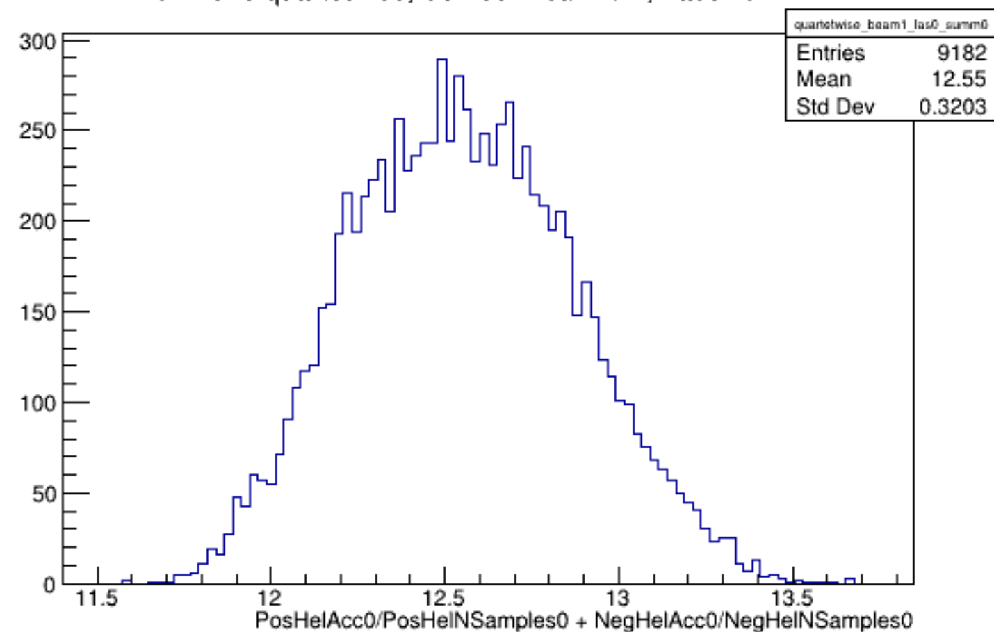
Run 4318 quartetwise, Sums0: Beam ON, Laser OFF
