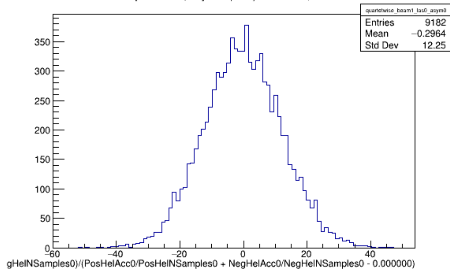
Run 4318 quartetwise, Asyms0 (Raw): Beam ON, Laser OFF
