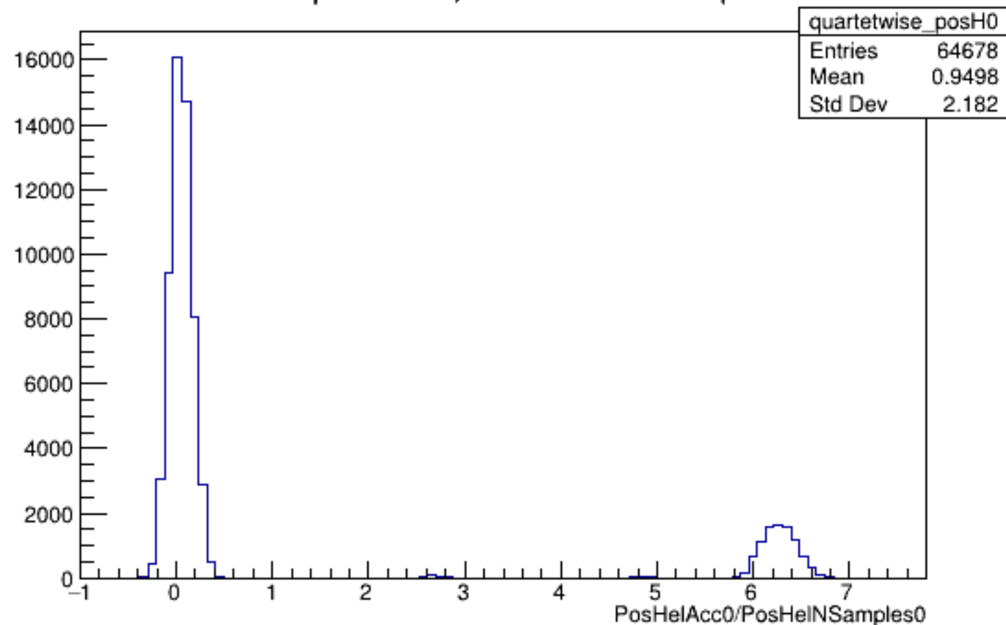
Run 4318 quartetwise, PosHelAcc0/NSamples0: All
