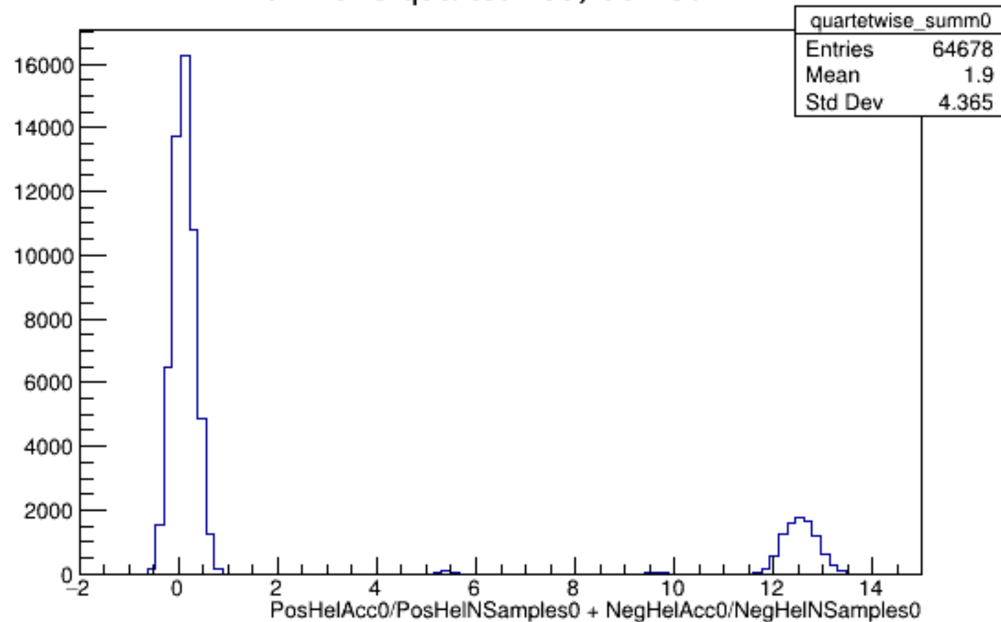
Run 4318 quartetwise, Sums0: All
