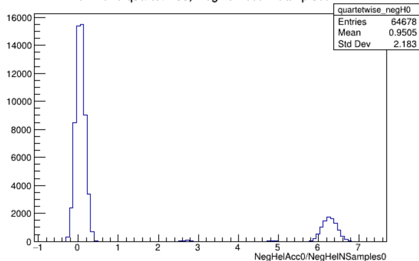
Run 4318 quartetwise, NegHelAcc0/NSamples0: All
