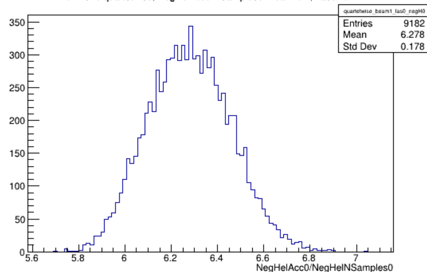
Run 4318 quartetwise, NegHelAcc0/NSamples0: Beam ON, Laser OFF
