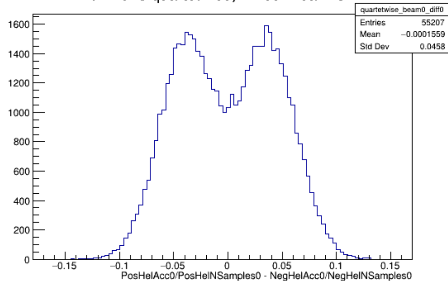
Run 4318 quartetwise, Diffs0: Beam OFF
