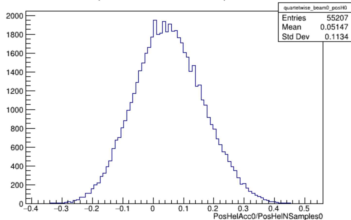
Run 4318 quartetwise, PosHelAcc0/NSamples0: Beam OFF
