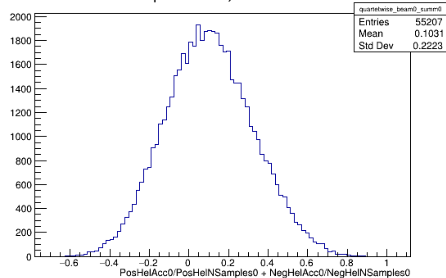
Run 4318 quartetwise, Sums0: Beam OFF
