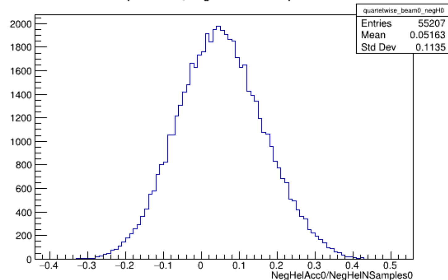
Run 4318 quartetwise, NegHelAcc0/NSamples0: Beam OFF
