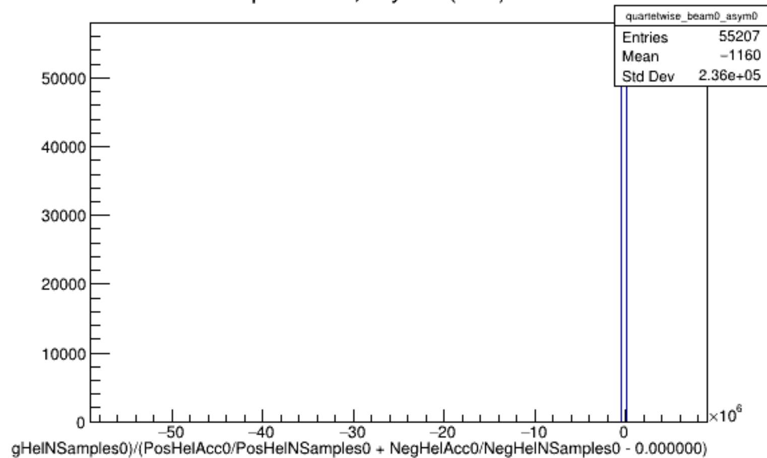
Run 4318 quartetwise, Asyms0 (Raw): Beam OFF
