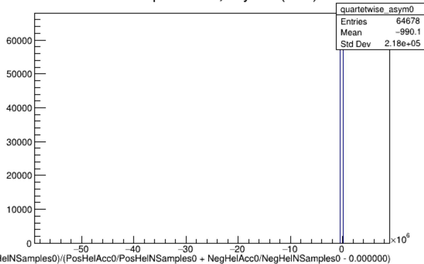
Run 4318 quartetwise, Asyms0 (Raw): All
