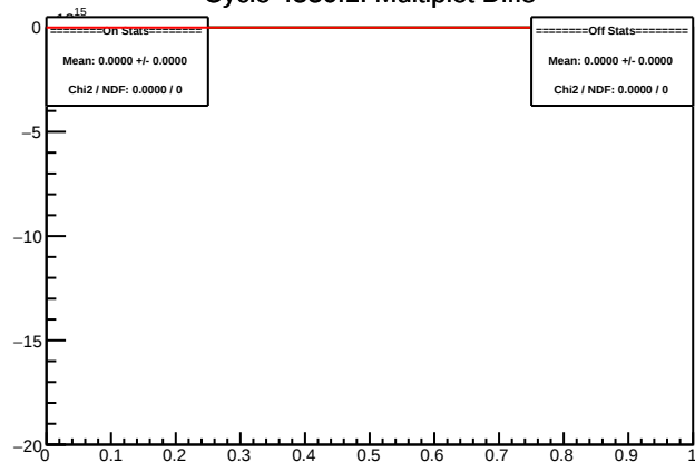
Cycle 4330.1: Multiplet Diffs
