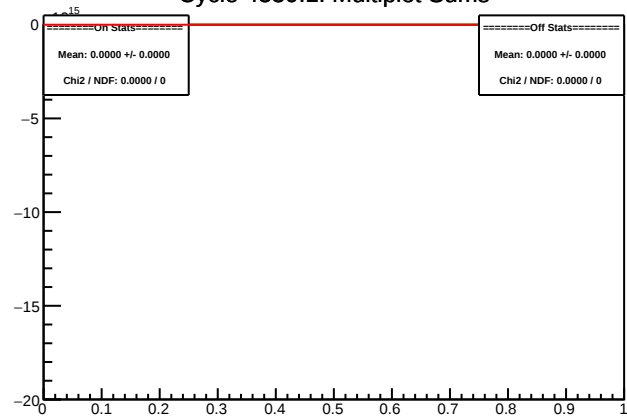
Cycle 4330.1: Multiplet Sums
