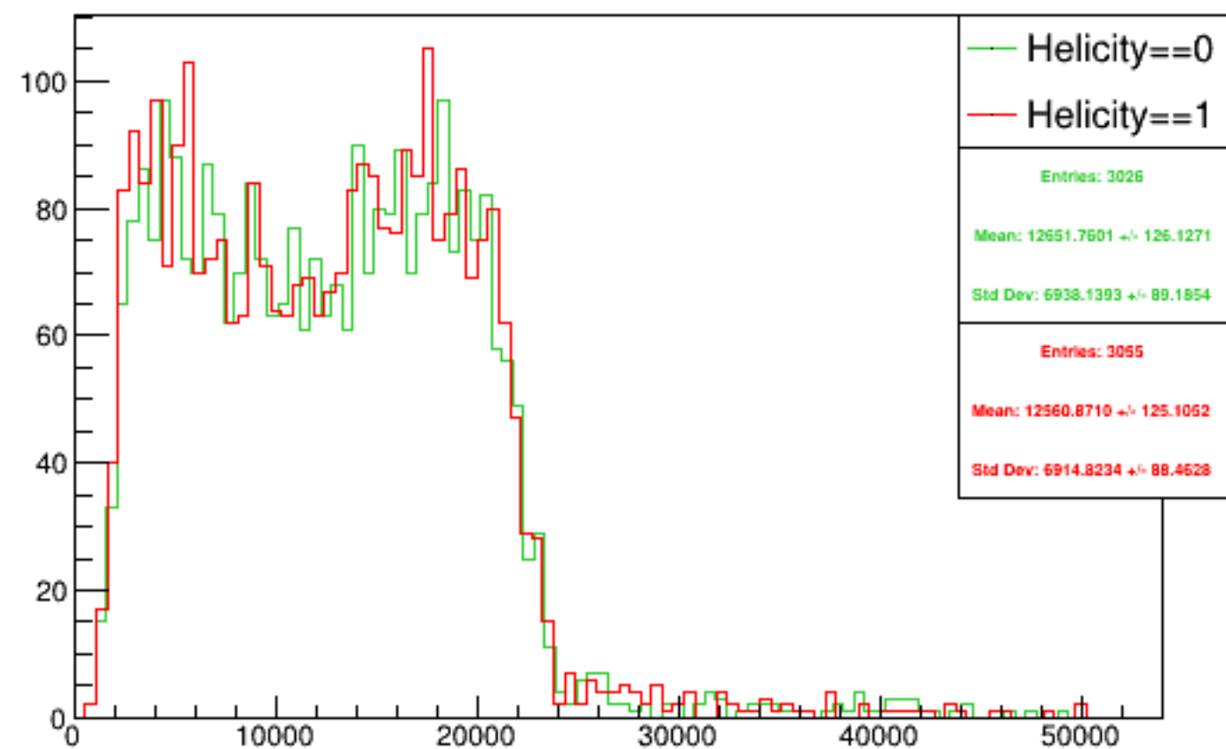
Run 4336 triggerwise, sums: Beam ON, Laser ON
