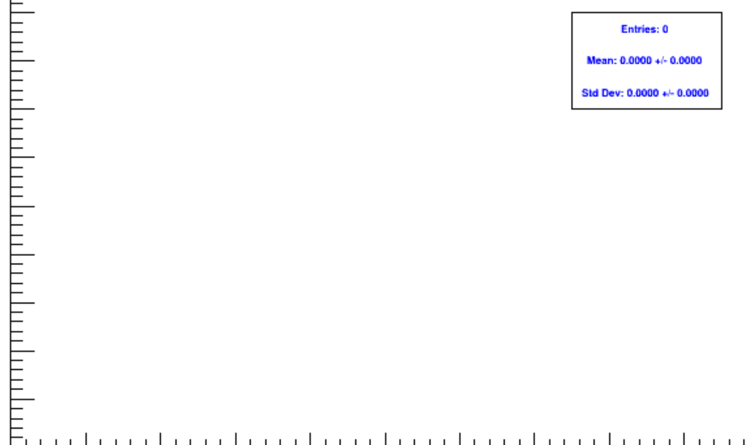
Run 4336 triggerwise, sums: Beam OFF
