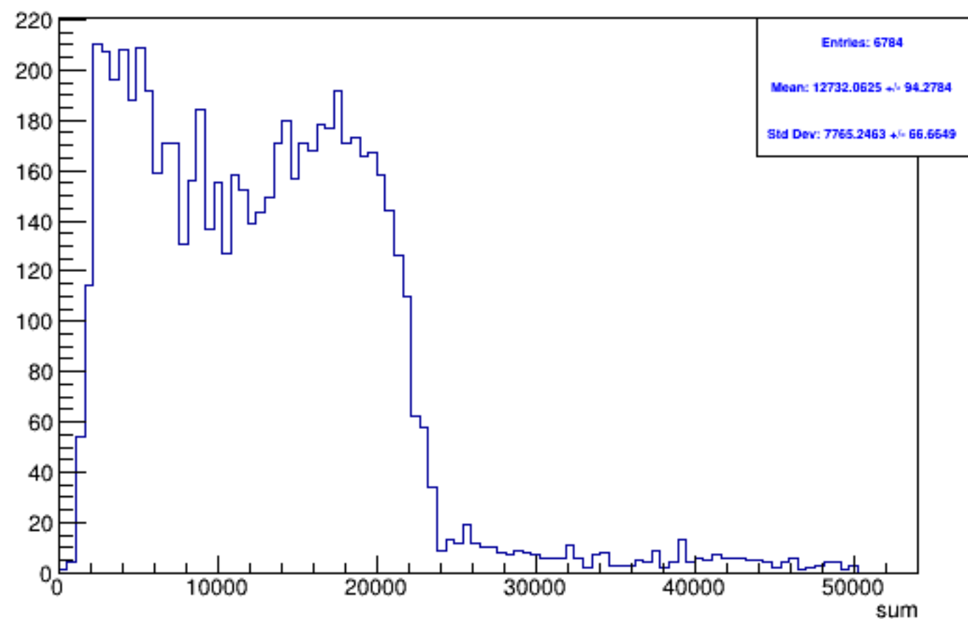
Run 4336 triggerwise, sums: All
