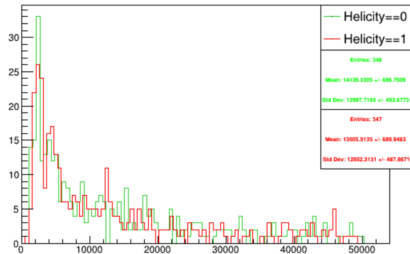
Run 4336 triggerwise, sums: Beam ON, Laser OFF
