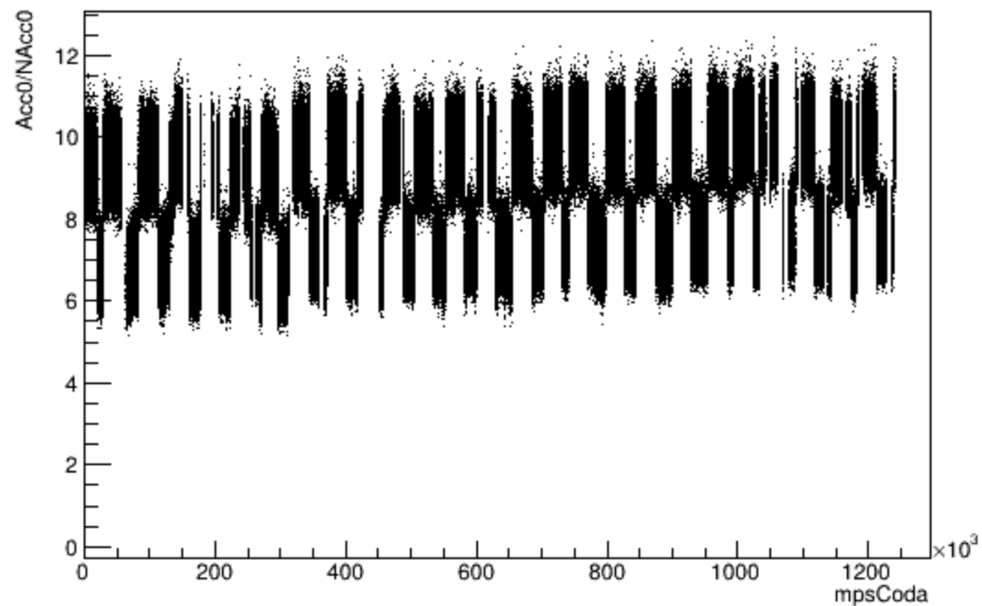
Run 4352 mpwise, Acc0/NAcc0:mpsCoda, beam ON, laser OFF
