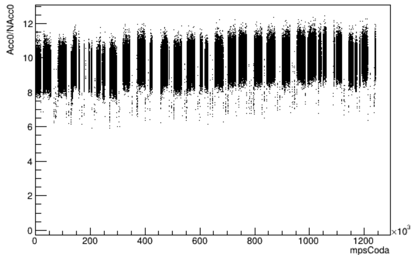
Run 4352 mpwise, Acc0/NAcc0:mpsCoda, beam ON, laser ON
