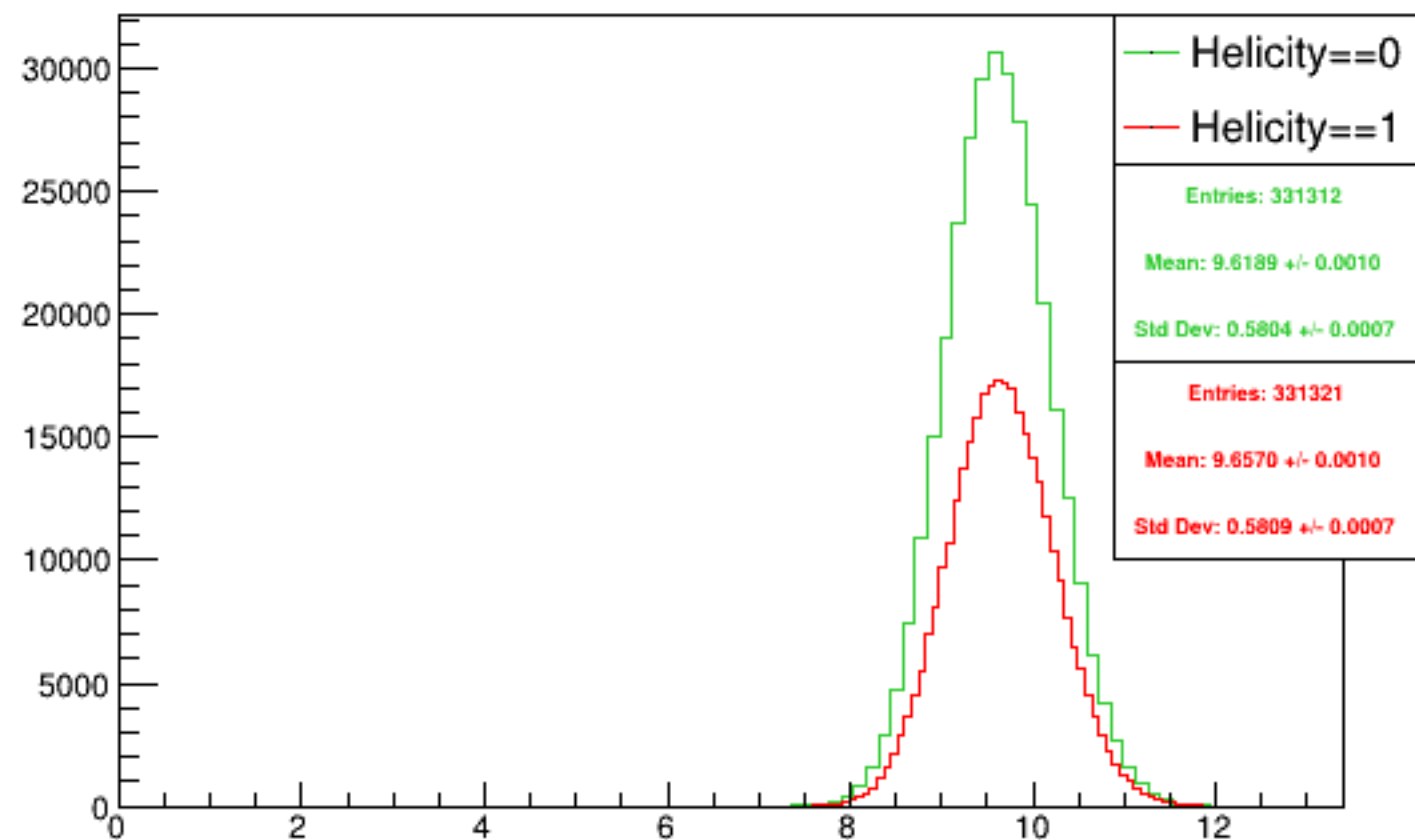
Run 4352 mpwise, acc0: Beam ON, Laser ON
