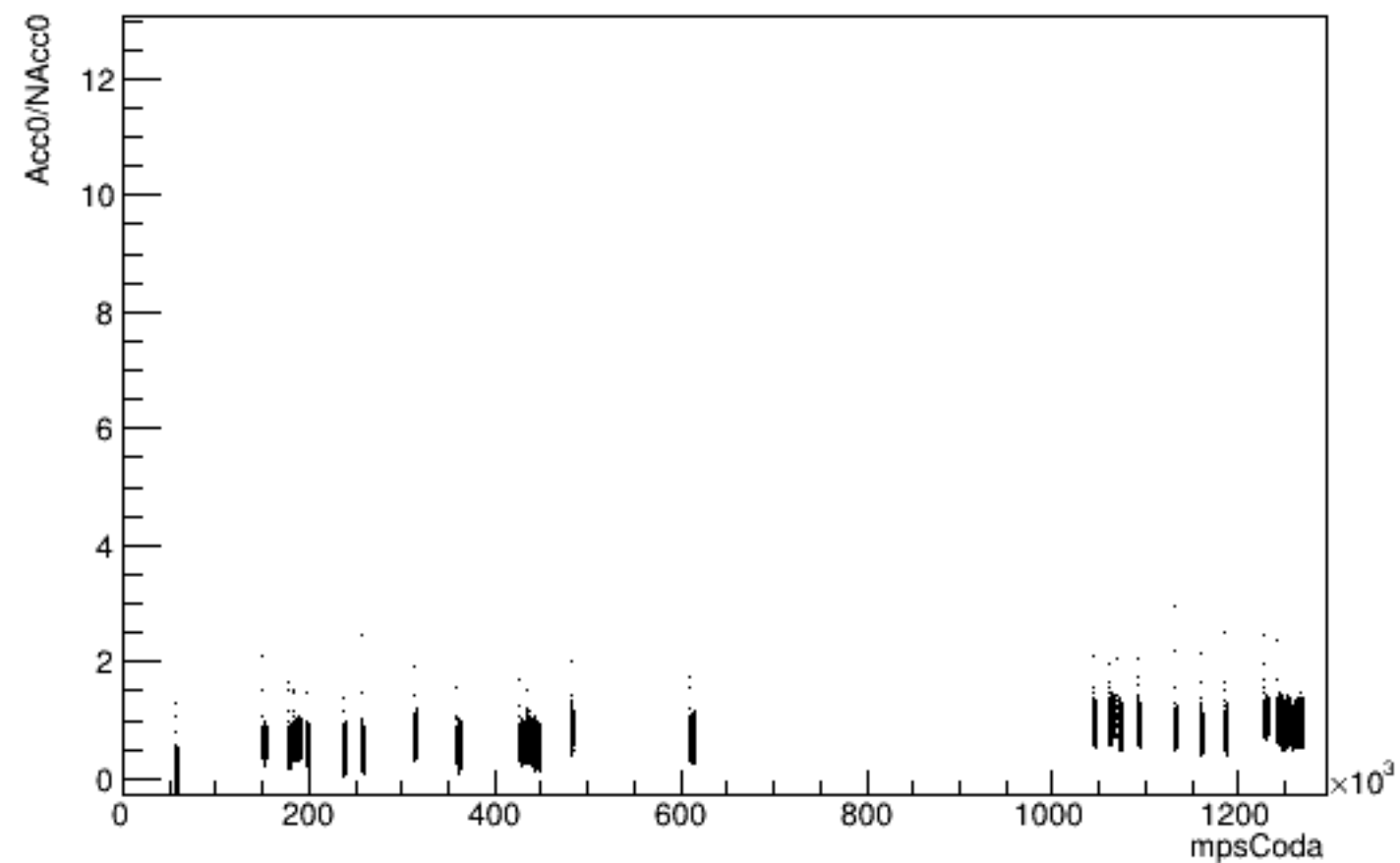
Run 4352 mpwise, Acc0/NAcc0:mpsCoda, beam OFF
