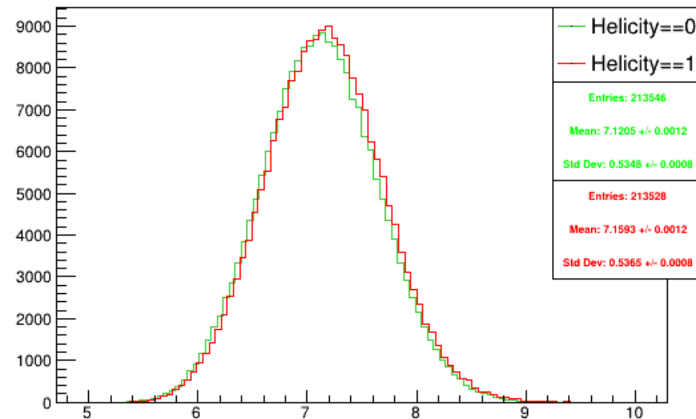
Run 4352 mpwise, acc0: Beam ON, Laser OFF
