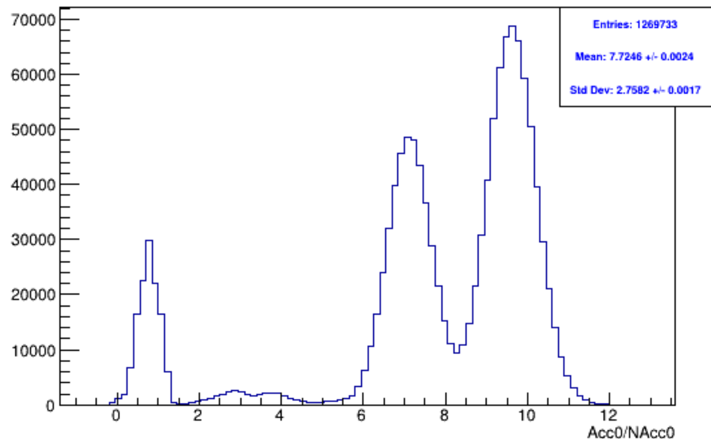
Run 4352 mpwise, acc0: All
