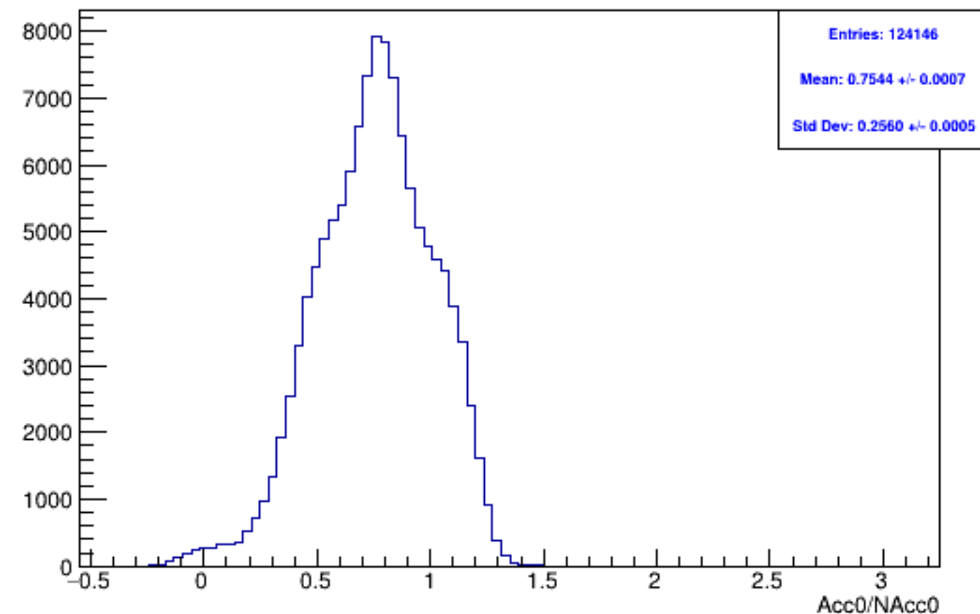
Run 4352 mpwise, acc0: Beam OFF
