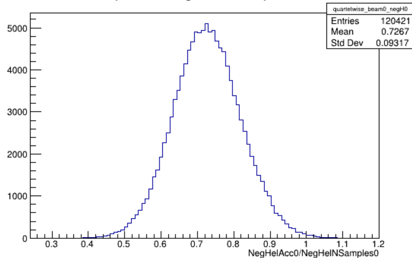
Run 4354 quartetwise, NegHelAcc0/NSamples0: Beam OFF
