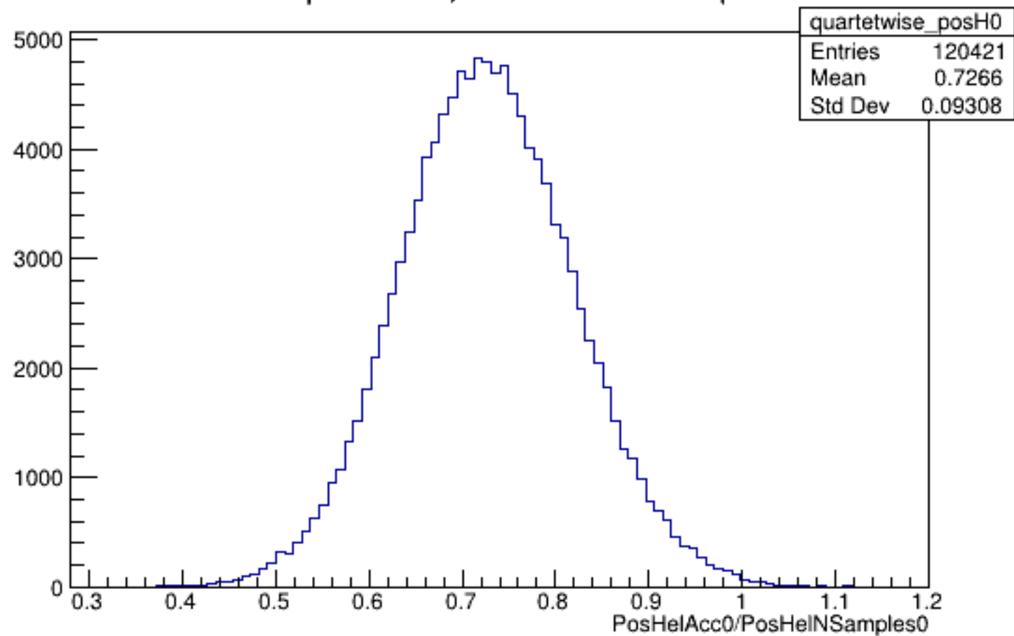
Run 4354 quartetwise, PosHelAcc0/NSamples0: All
