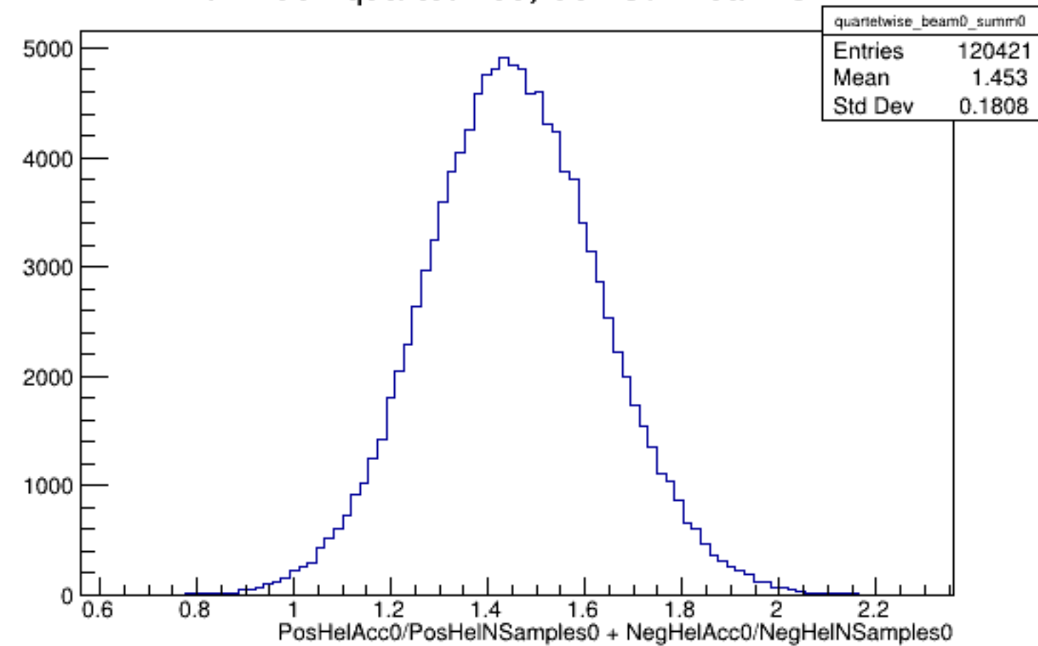
Run 4354 quartetwise, Sums0: Beam OFF
