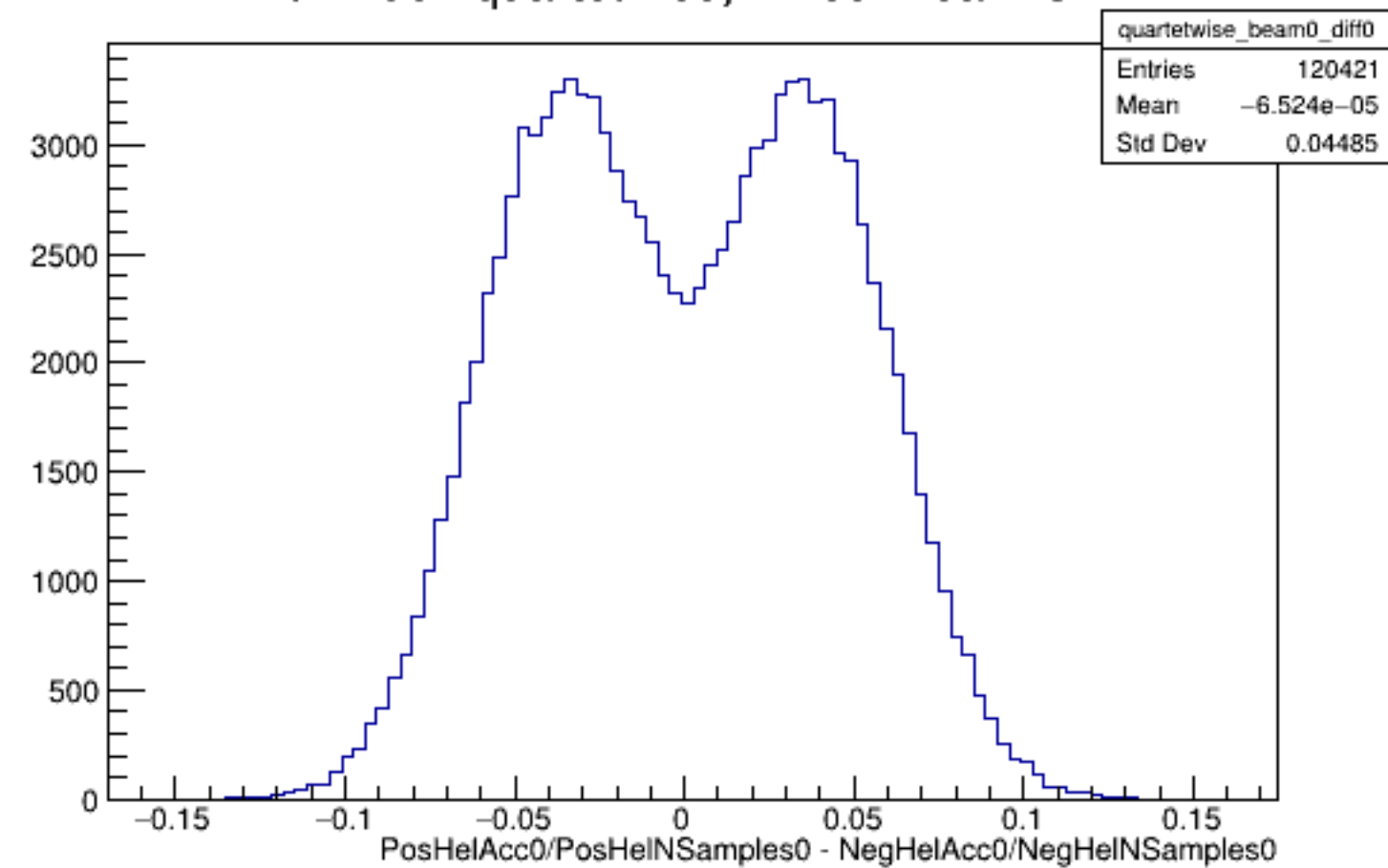
Run 4354 quartetwise, Diffs0: Beam OFF
