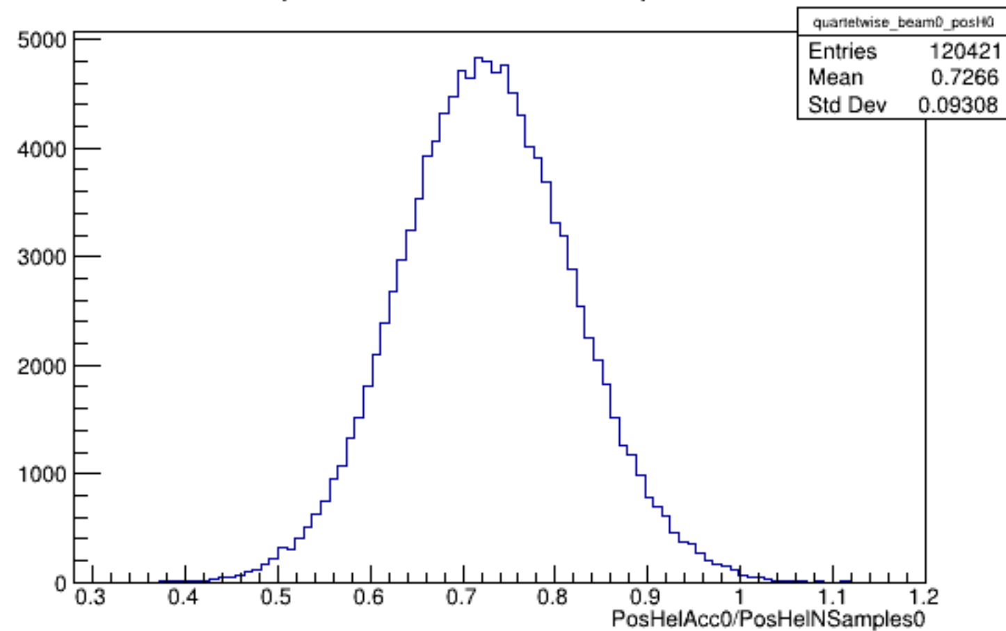
Run 4354 quartetwise, PosHelAcc0/NSamples0: Beam OFF
