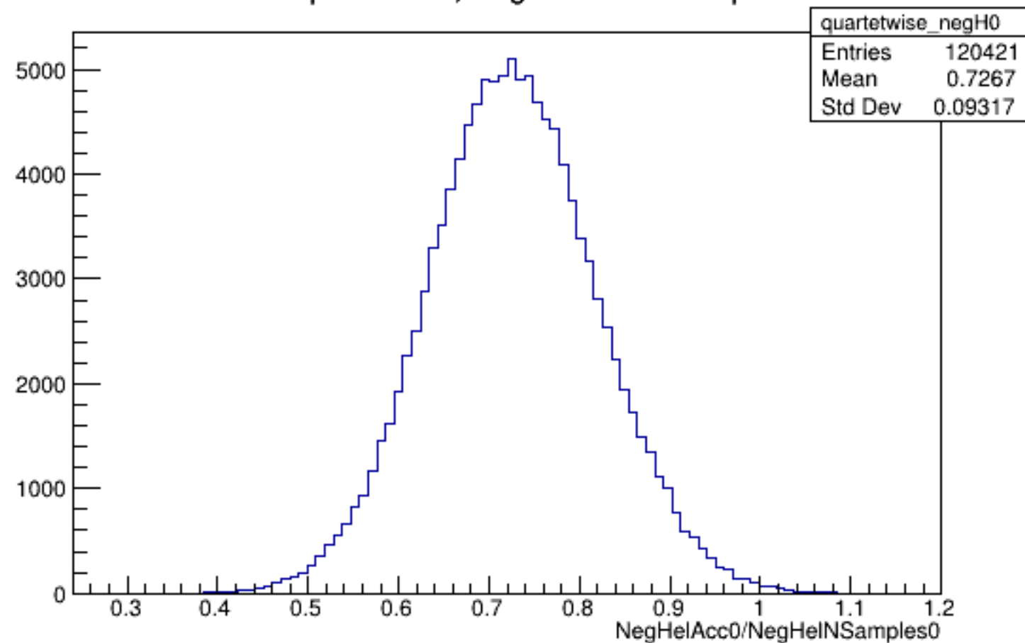
Run 4354 quartetwise, NegHelAcc0/NSamples0: All
