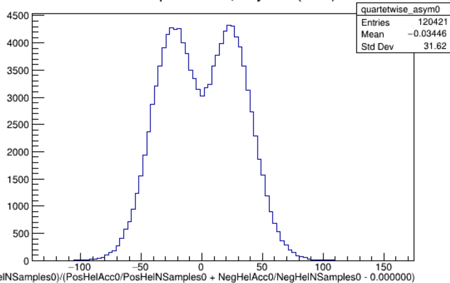
Run 4354 quartetwise, Asyms0 (Raw): All
