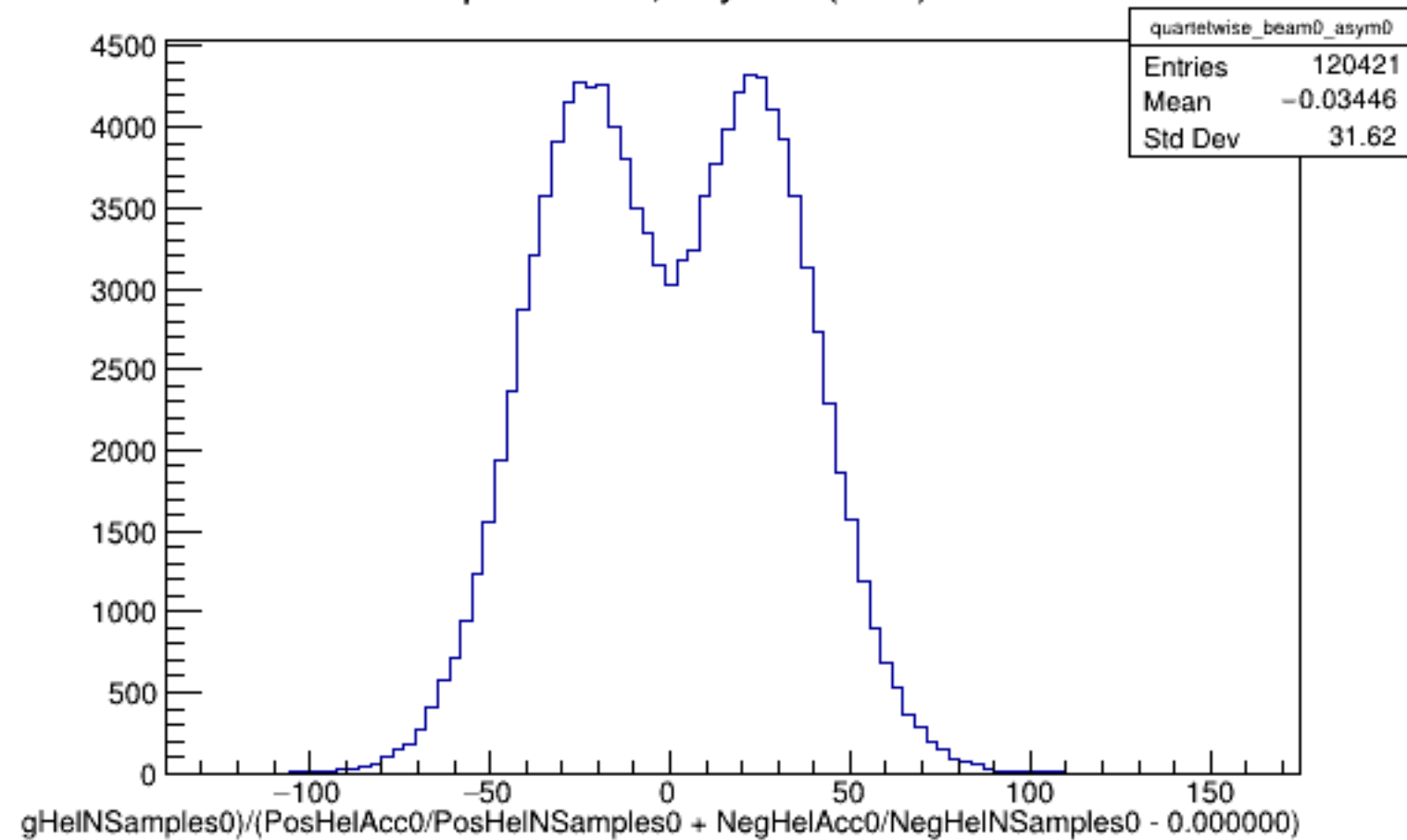
Run 4354 quartetwise, Asyms0 (Raw): Beam OFF
