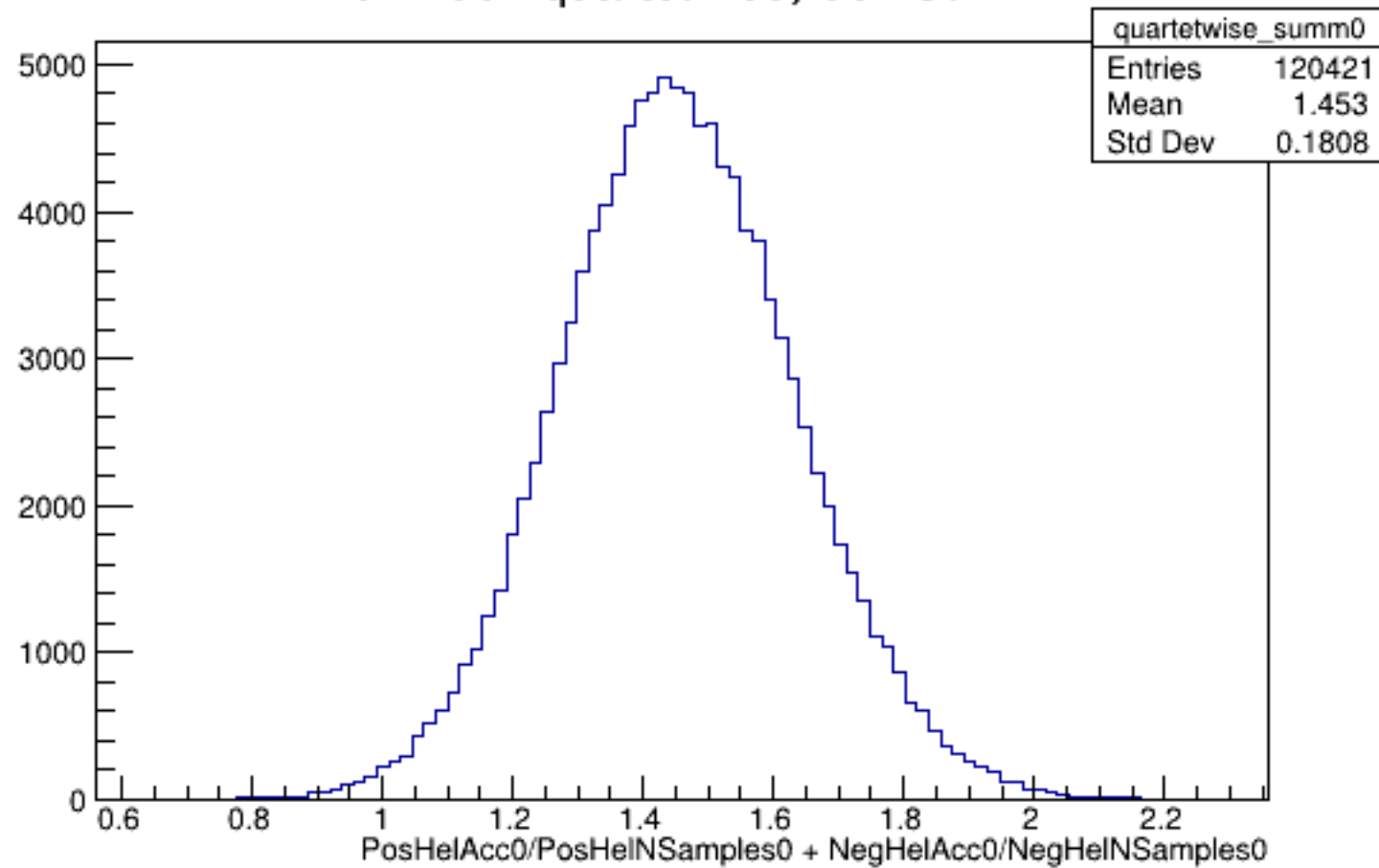
Run 4354 quartetwise, Sums0: All
