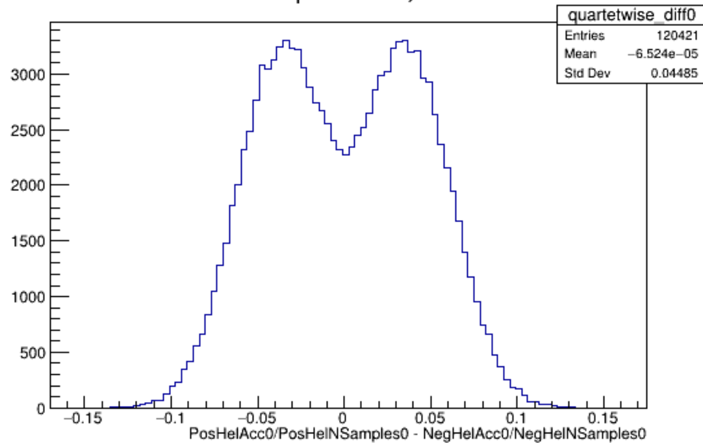
Run 4354 quartetwise, Diffs0: All
