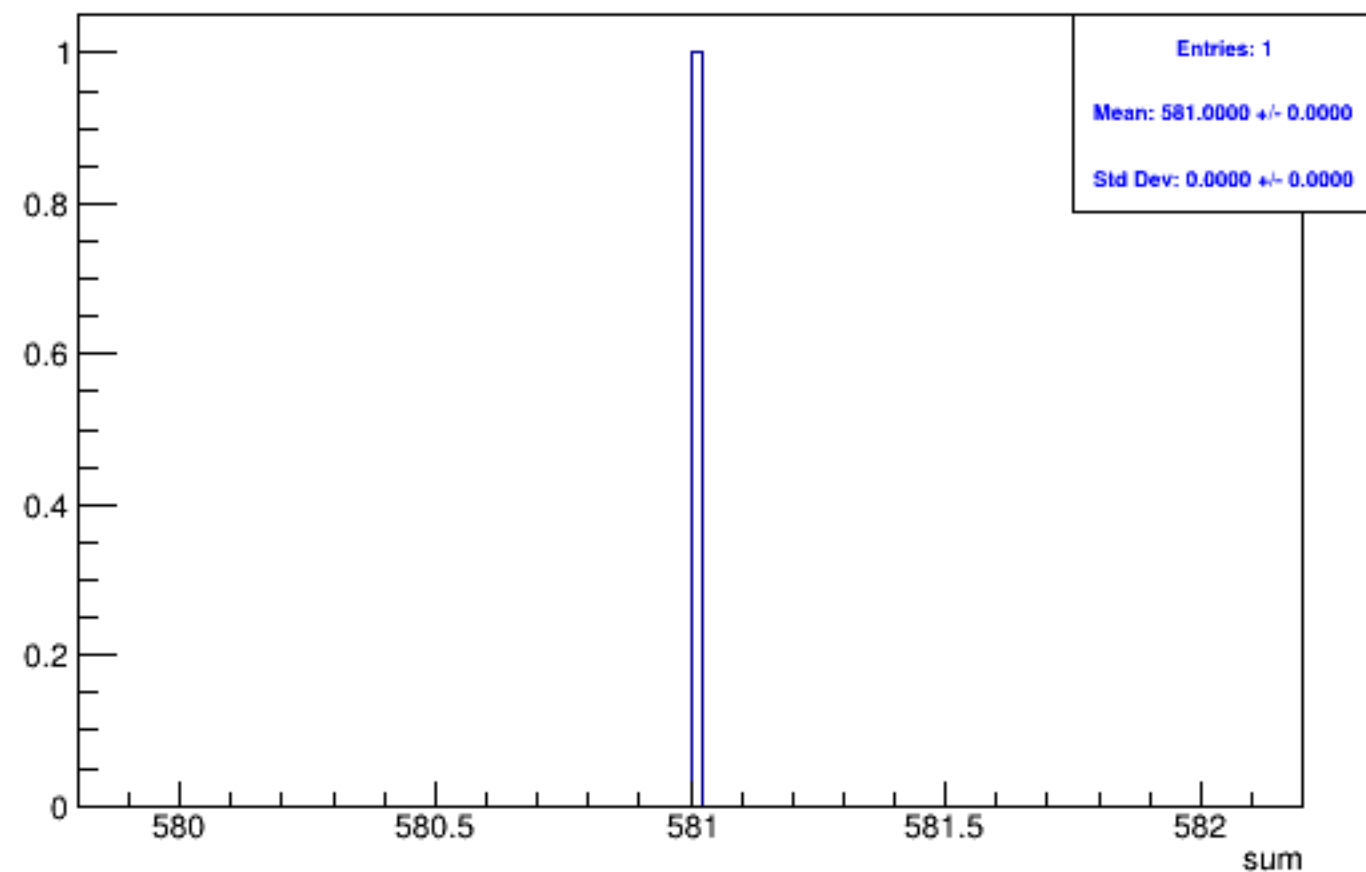
Run 4354 triggerwise, sums: Beam OFF
