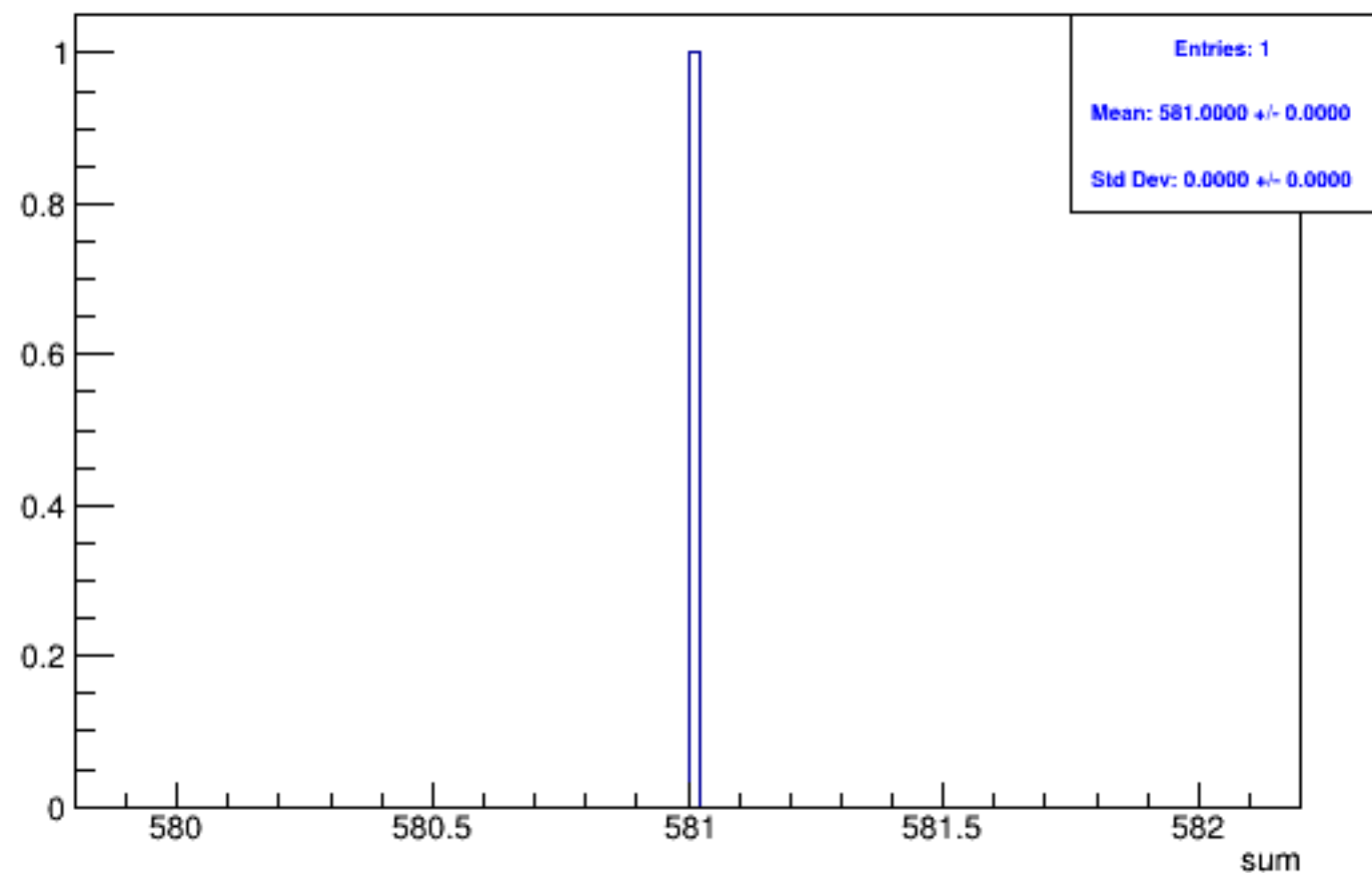
Run 4354 triggerwise, sums: All
