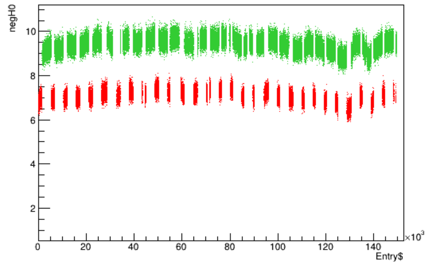
Run 4357 quartetwise, negH0 vs time
