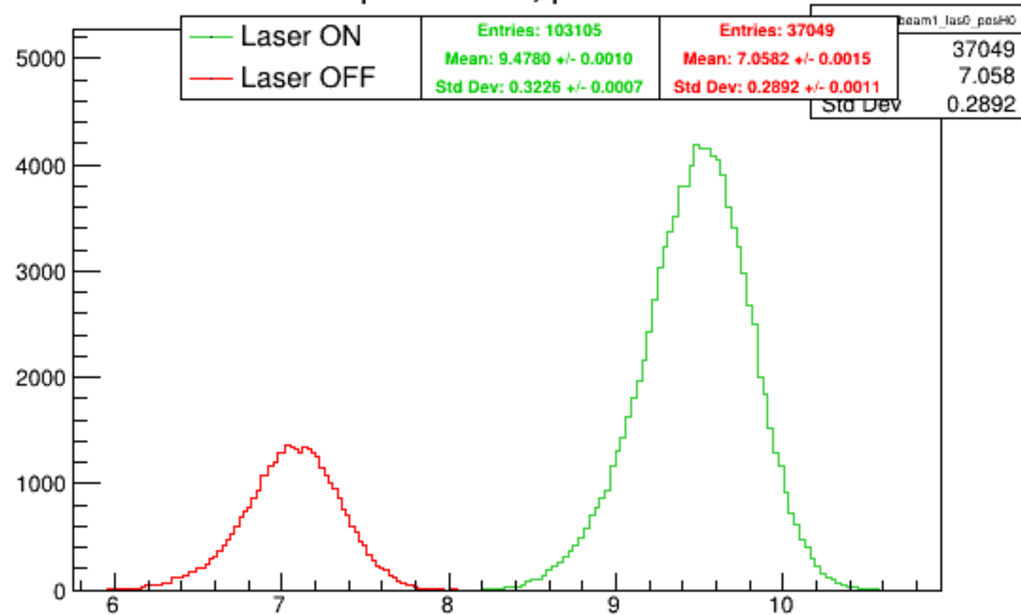
Run 4357 quartetwise, posH0: Beam ON
