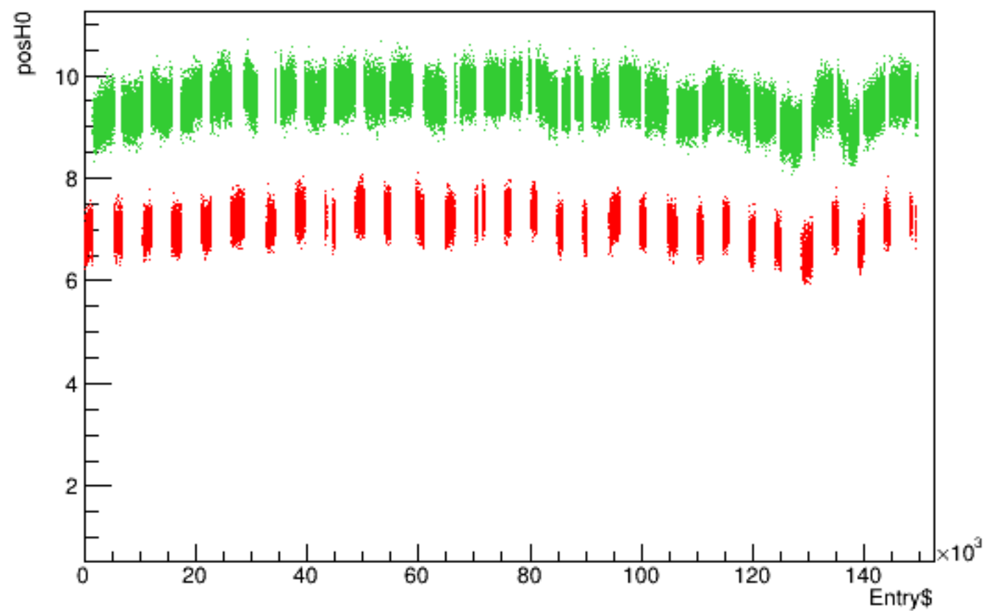
Run 4357 quartetwise, posH0 vs time
