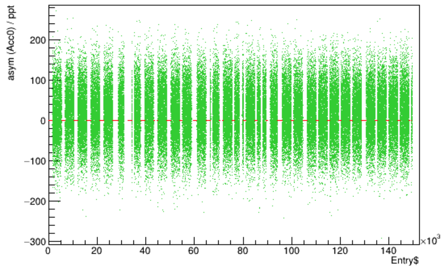
Run 4357 quartetwise, asym0sub vs time
