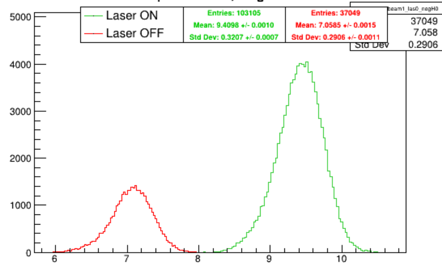
Run 4357 quartetwise, negH0: Beam ON
