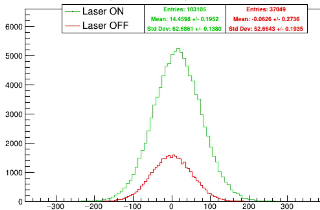
Run 4357 quartetwise, asym0sub: Beam ON
