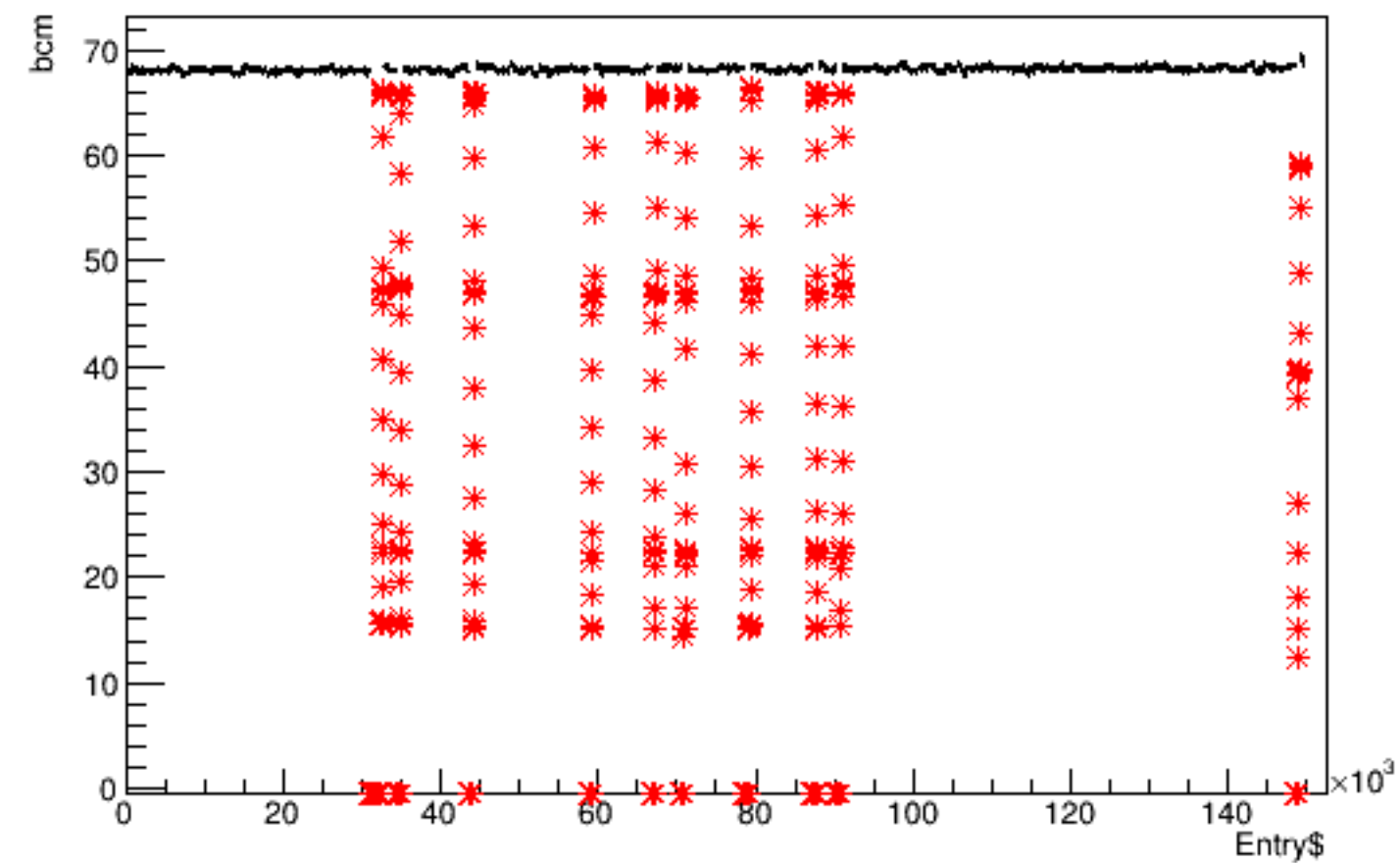
Run 4357 quartetwise, bcm vs time
