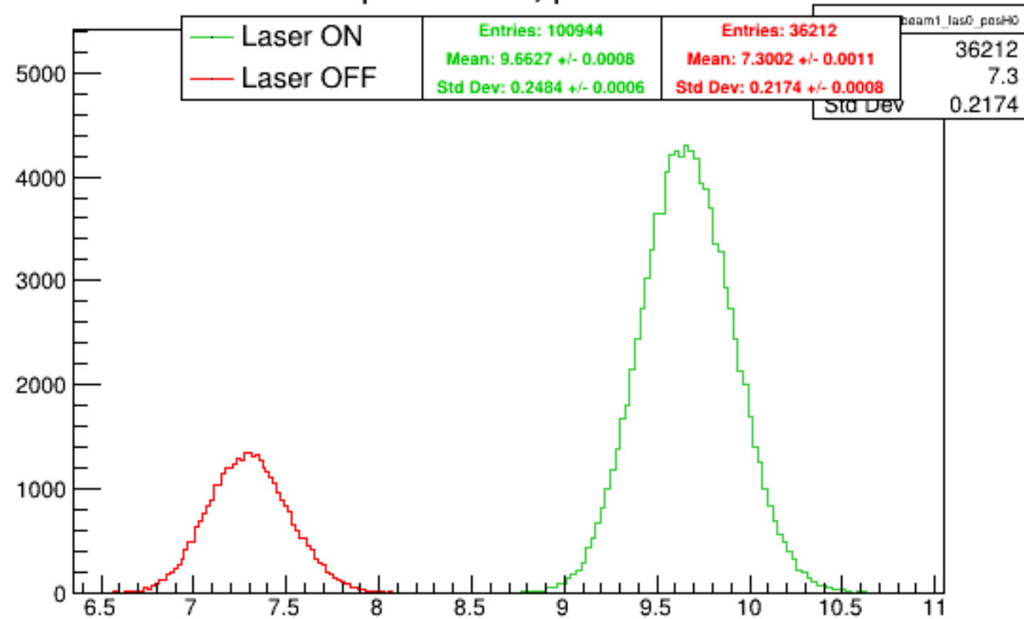
Run 4362 quartetwise, posH0: Beam ON
