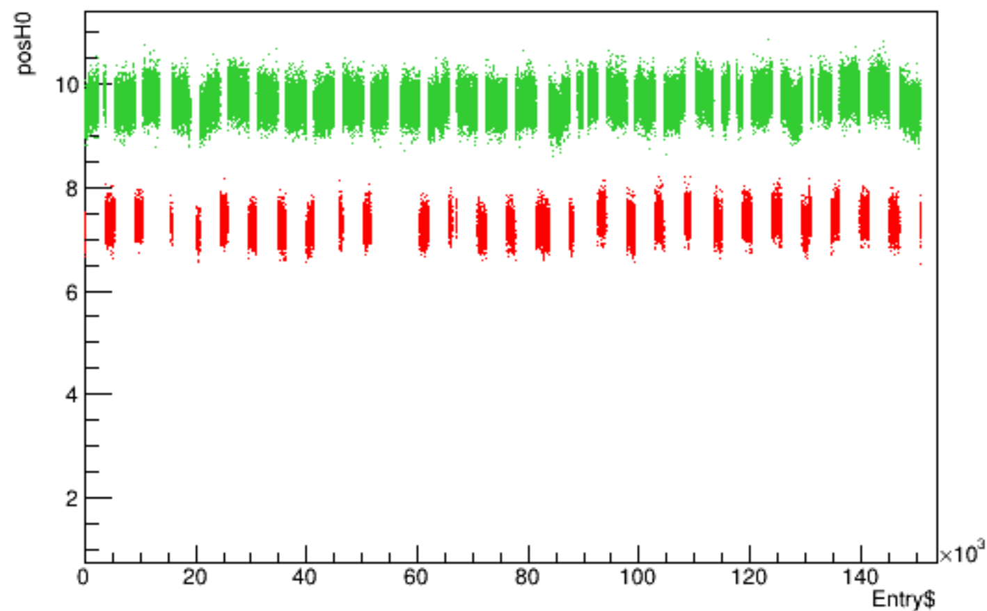
Run 4362 quartetwise, posH0 vs time
