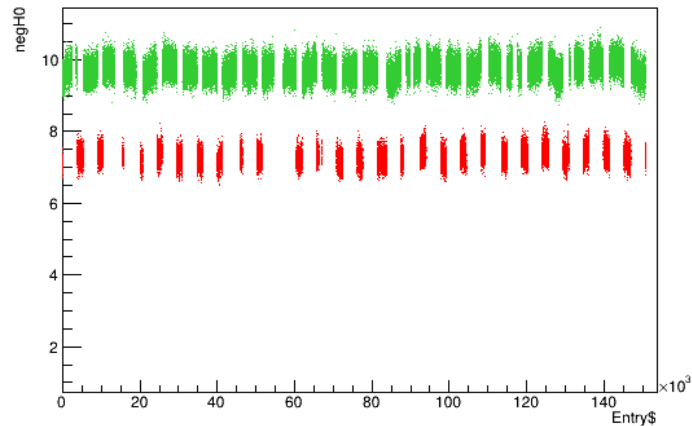
Run 4362 quartetwise, negH0 vs time
