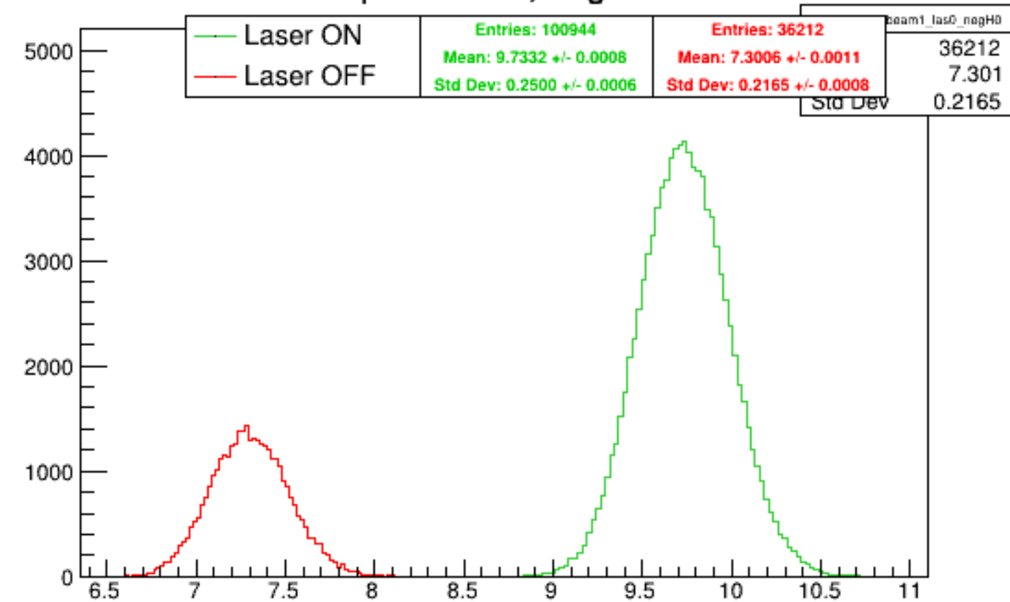
Run 4362 quartetwise, negH0: Beam ON
