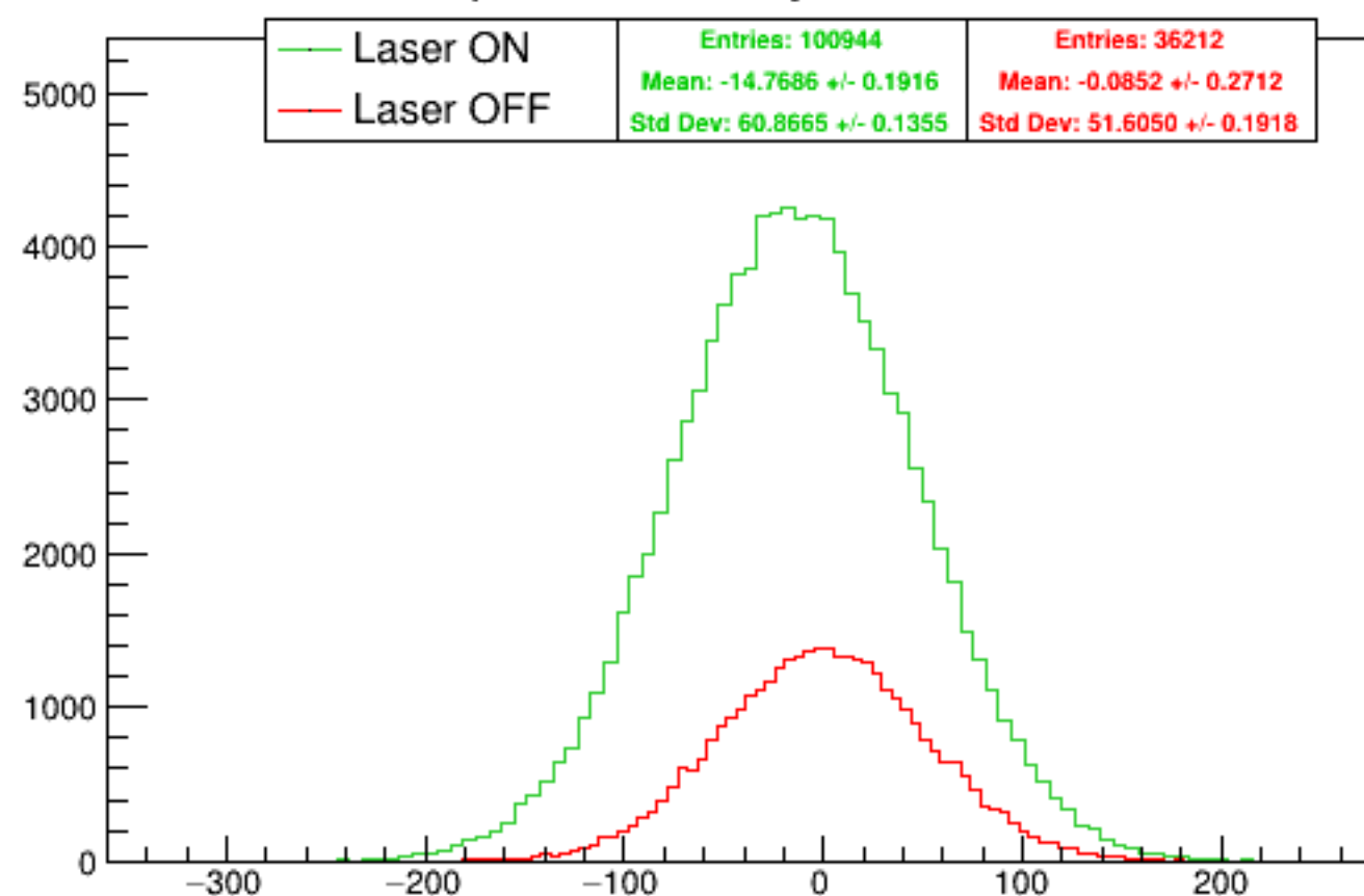
Run 4362 quartetwise, asym0sub: Beam ON
