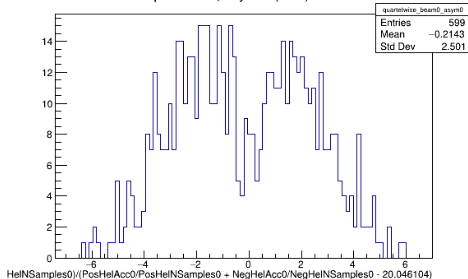
Run 4374 quartetwise, Asyms0 (Raw): Beam OFF
