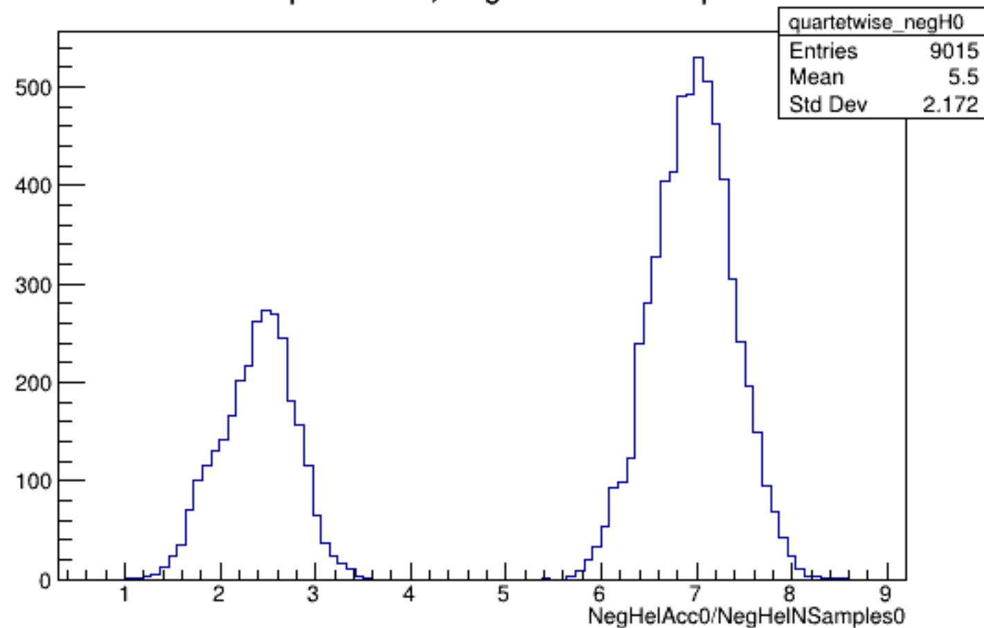
Run 4378 quartetwise, NegHelAcc0/NSamples0: All
