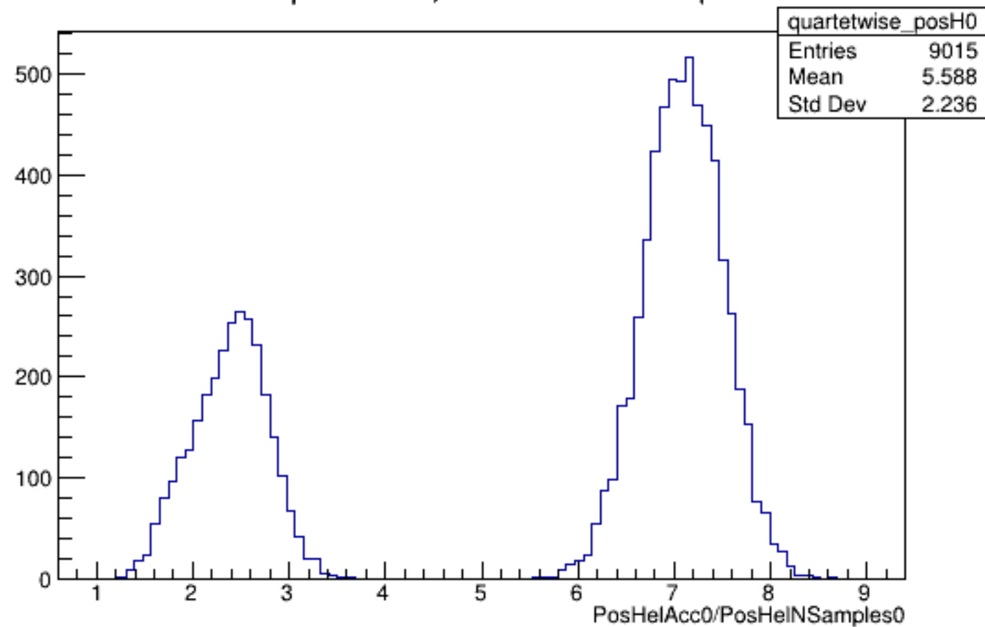
Run 4378 quartetwise, PosHelAcc0/NSamples0: All
