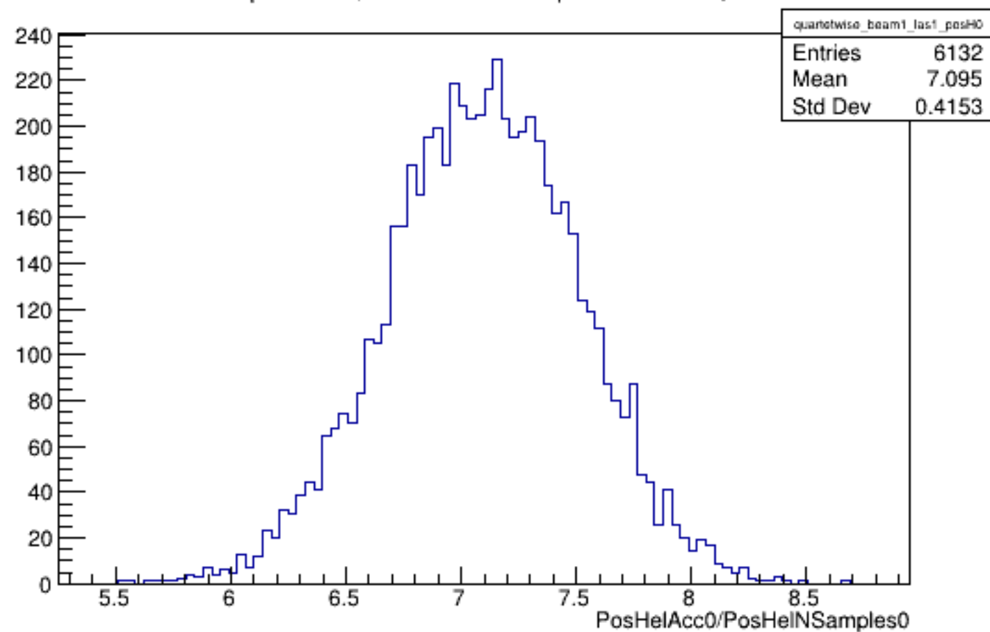
Run 4378 quartetwise, PosHelAcc0/NSamples0: Beam ON, Laser ON
