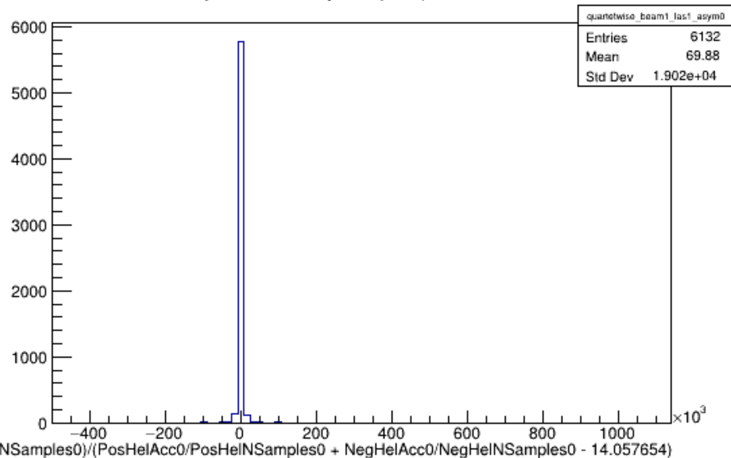
Run 4378 quartetwise, Asyms0 (Raw): Beam ON, Laser ON
