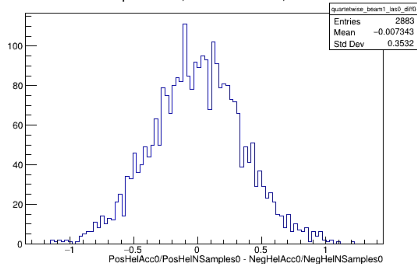
Run 4378 quartetwise, Diffs0: Beam ON, Laser OFF
