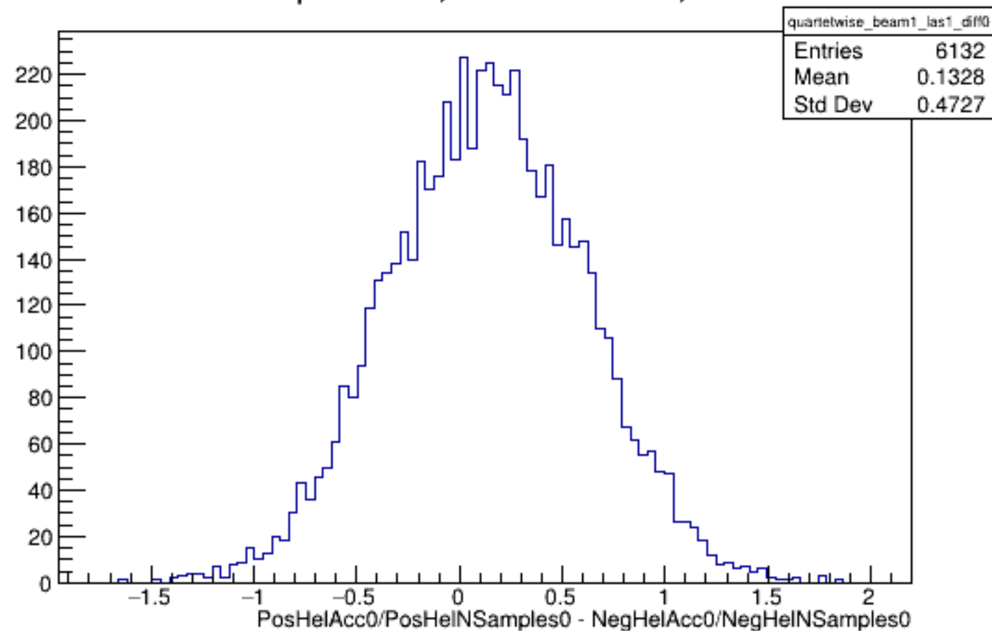
Run 4378 quartetwise, Diffs0: Beam ON, Laser ON
