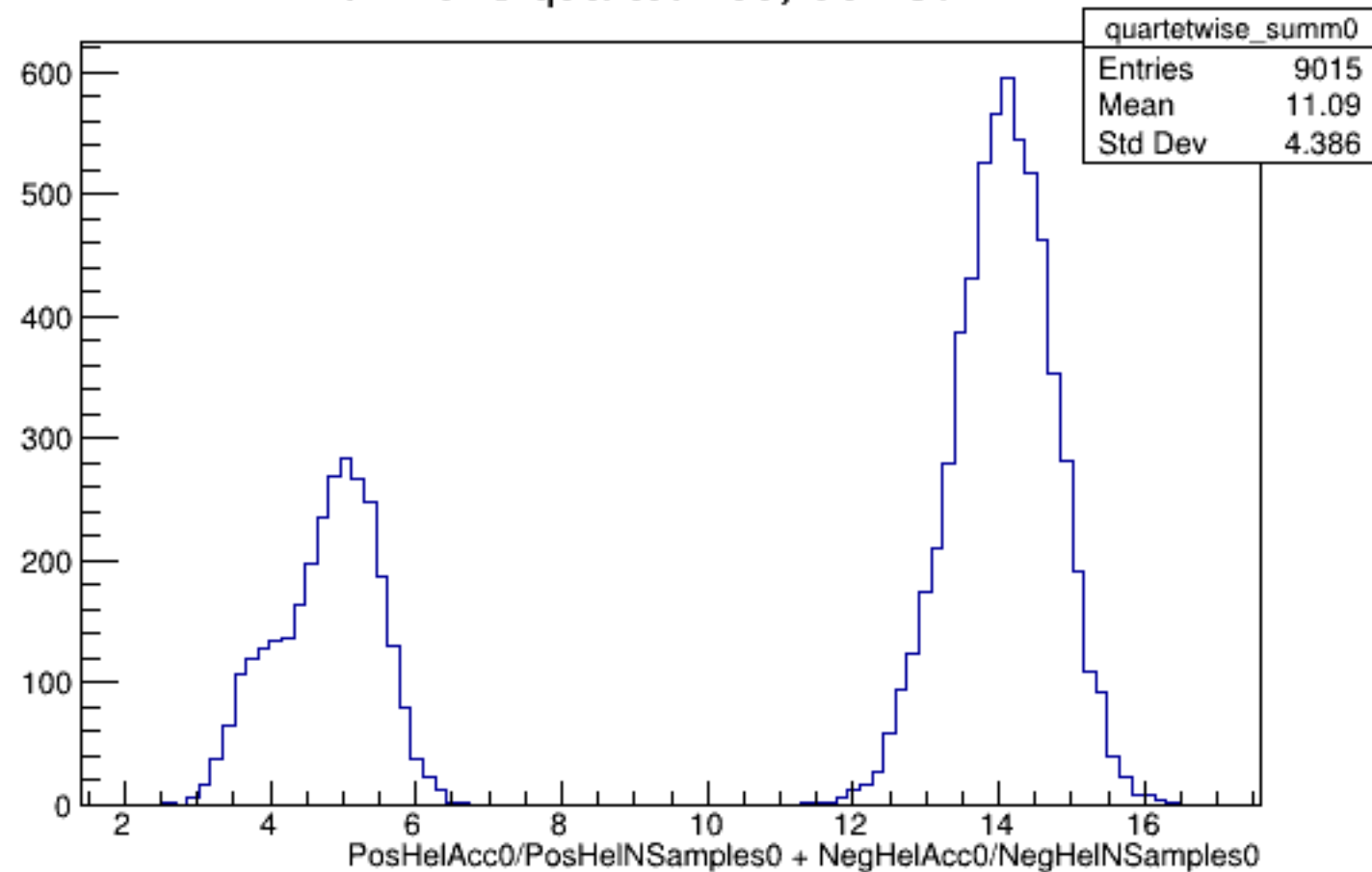
Run 4378 quartetwise, Sums0: All
