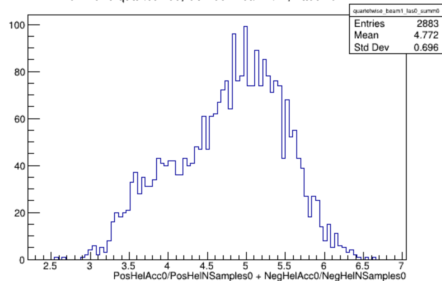
Run 4378 quartetwise, Sums0: Beam ON, Laser OFF
