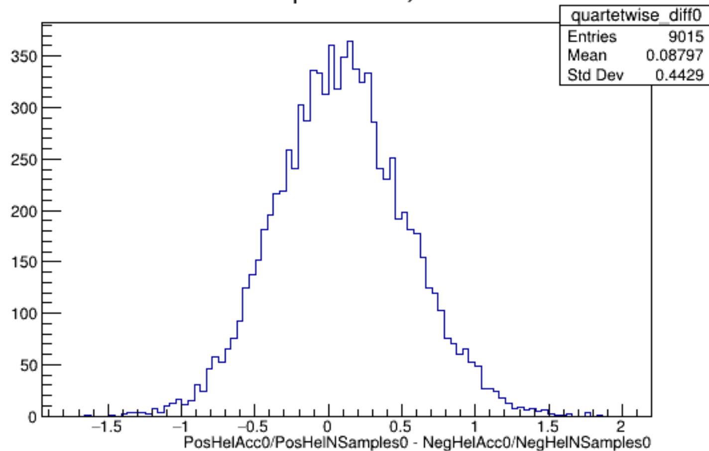
Run 4378 quartetwise, Diffs0: All
