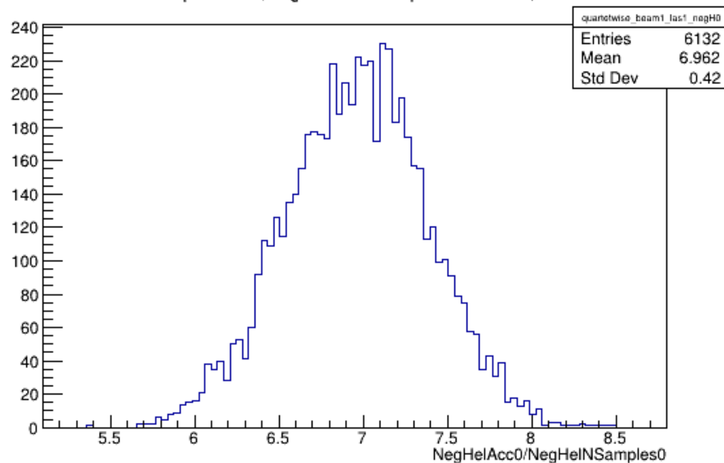
Run 4378 quartetwise, NegHelAcc0/NSamples0: Beam ON, Laser ON
