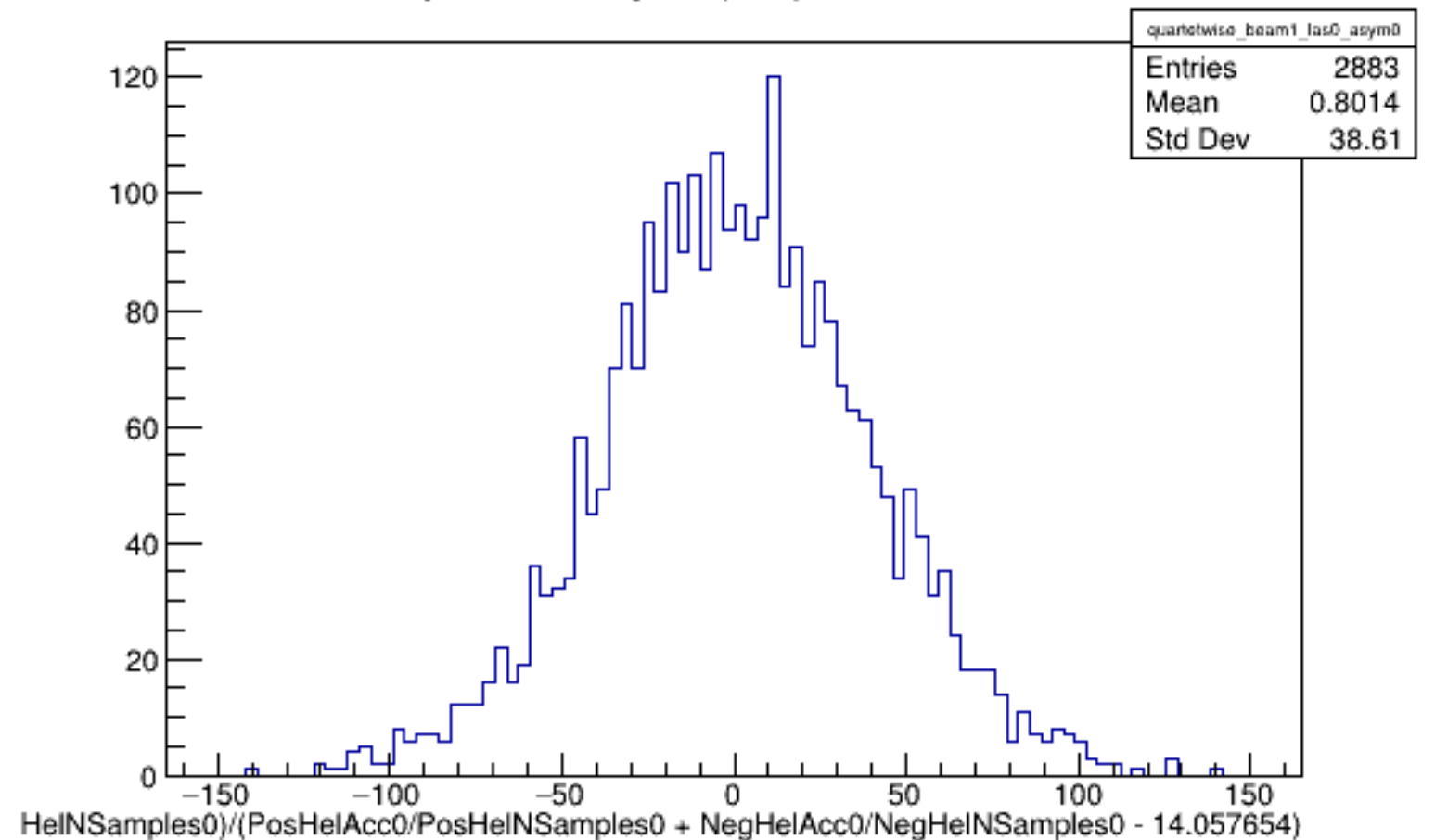
Run 4378 quartetwise, Asyms0 (Raw): Beam ON, Laser OFF
