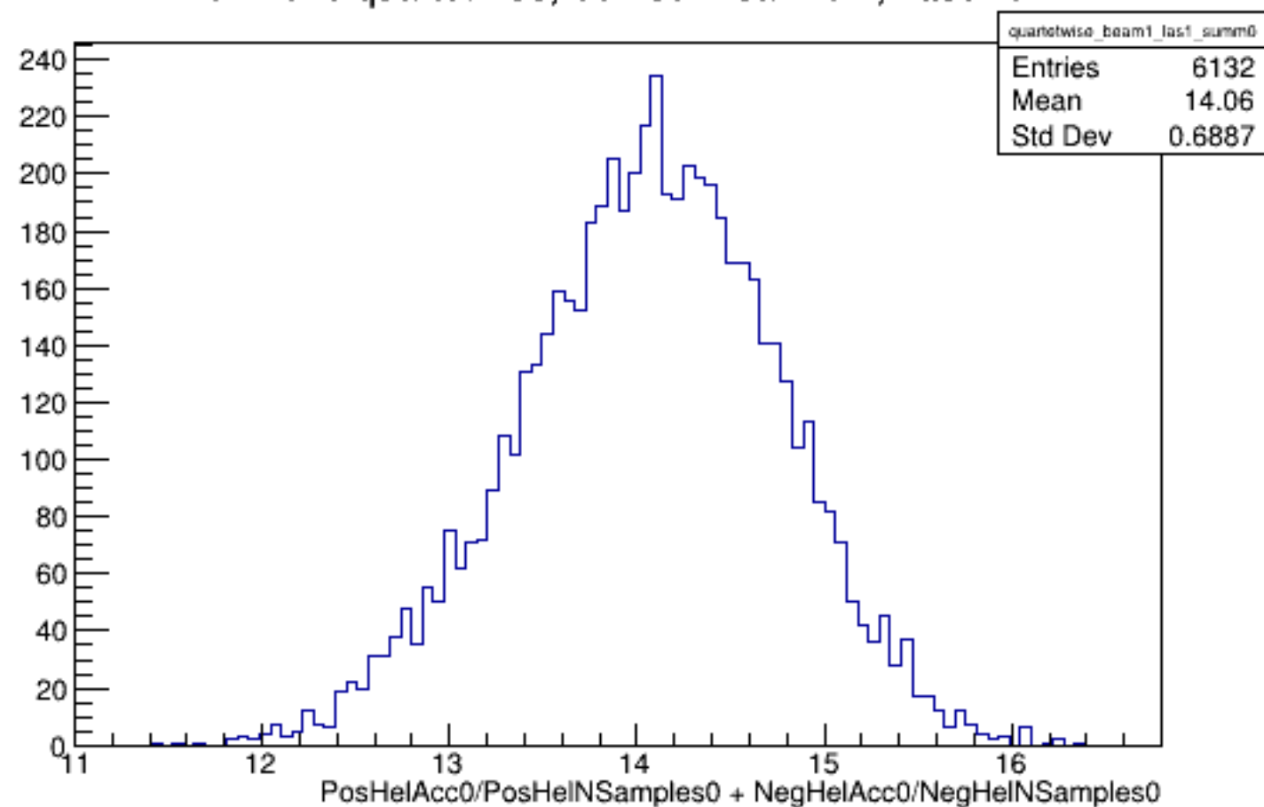
Run 4378 quartetwise, Sums0: Beam ON, Laser ON
