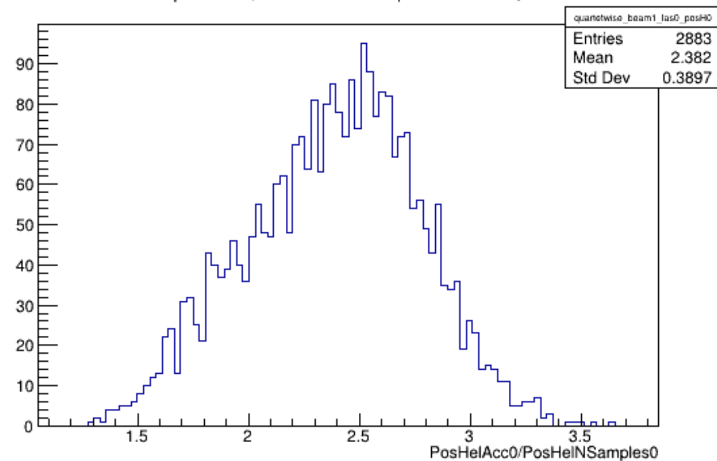
Run 4378 quartetwise, PosHelAcc0/NSamples0: Beam ON, Laser OFF
