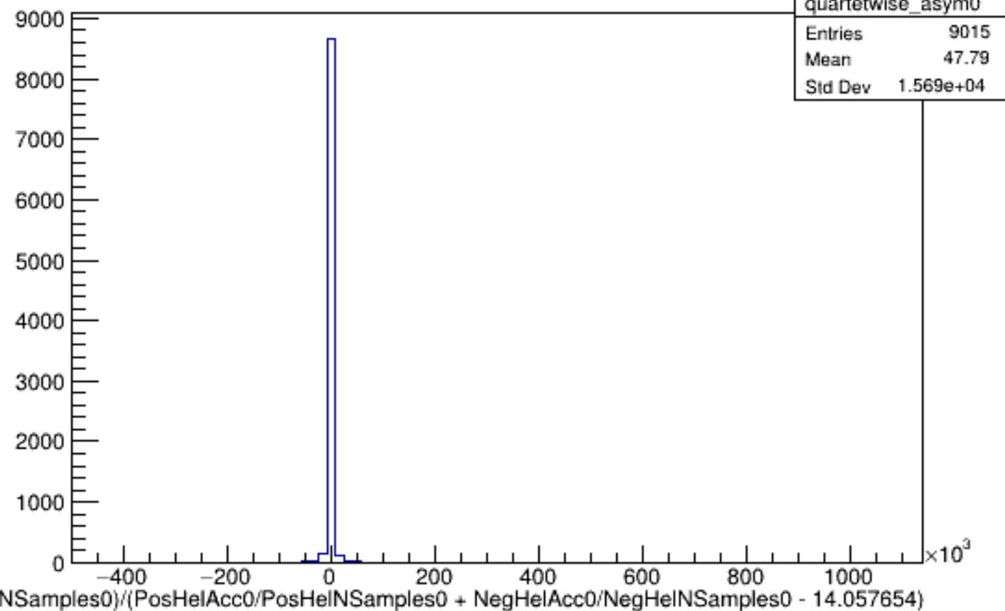
Run 4378 quartetwise, Asyms0 (Raw): All
