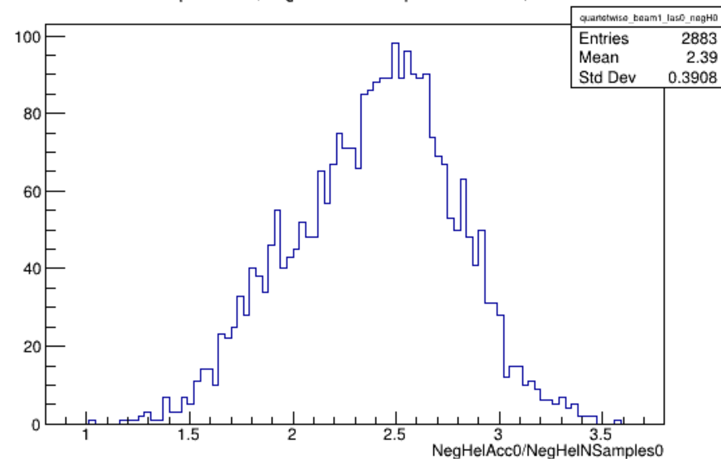
Run 4378 quartetwise, NegHelAcc0/NSamples0: Beam ON, Laser OFF
