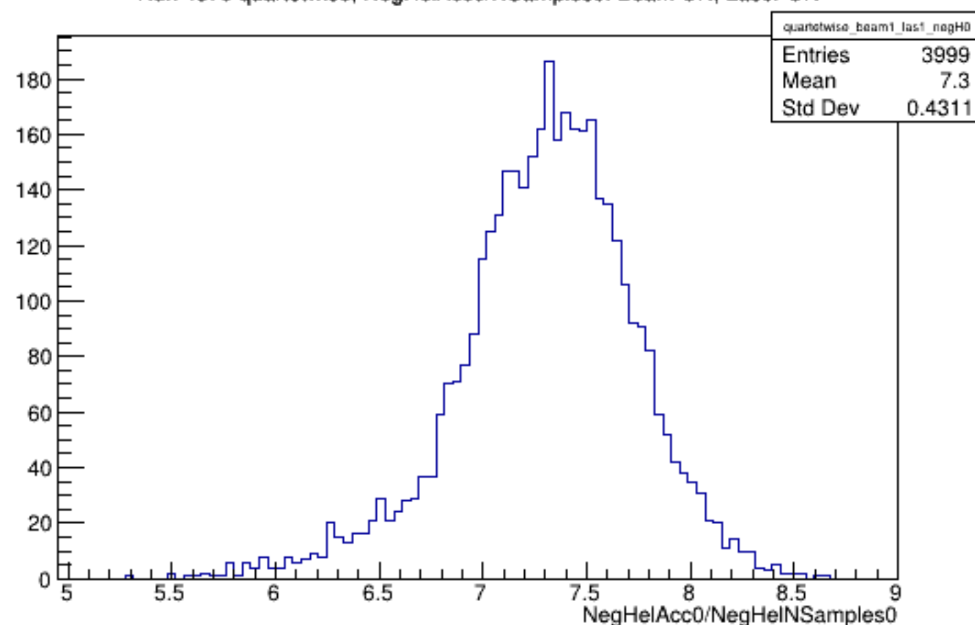
Run 4379 quartetwise, NegHelAcc0/NSamples0: Beam ON, Laser ON
