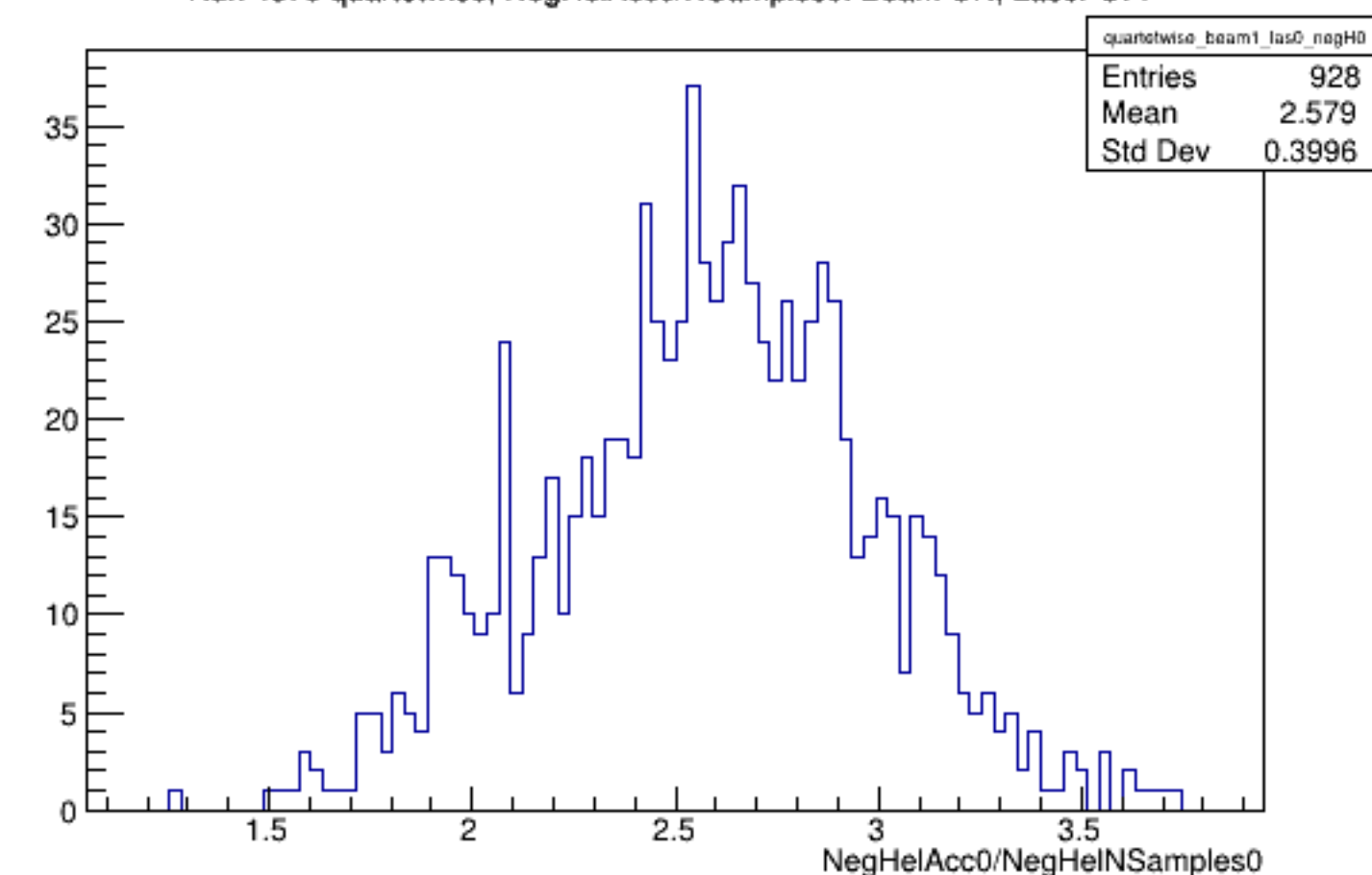
Run 4379 quartetwise, NegHelAcc0/NSamples0: Beam ON, Laser OFF
