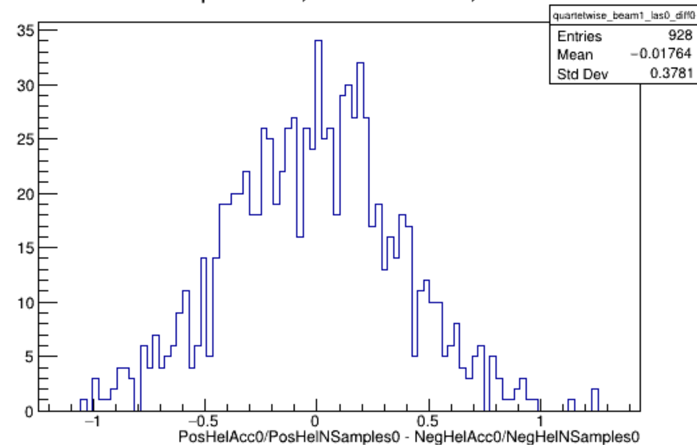
Run 4379 quartetwise, Diffs0: Beam ON, Laser OFF
