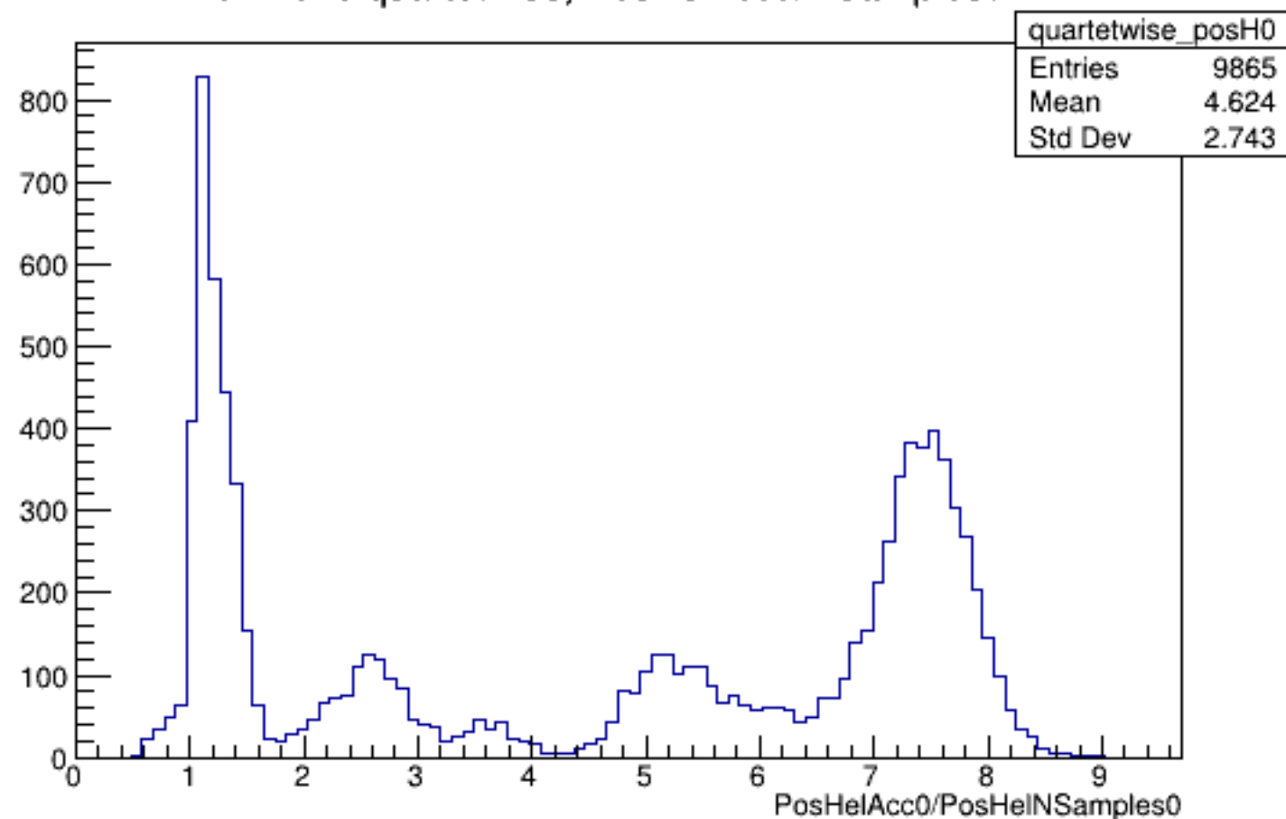
Run 4379 quartetwise, PosHelAcc0/NSamples0: All
