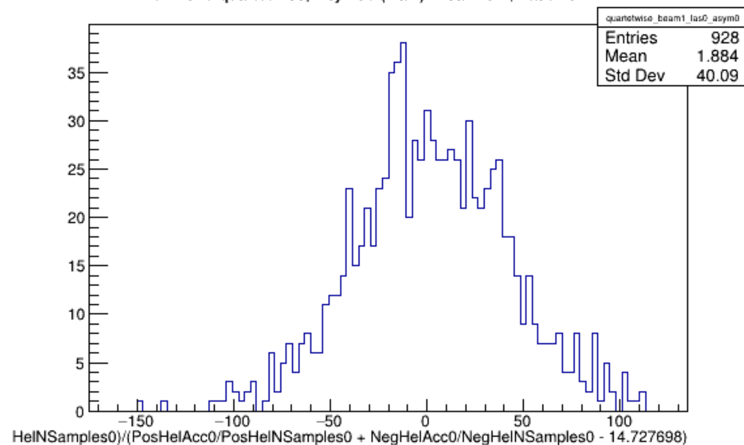
Run 4379 quartetwise, Asyms0 (Raw): Beam ON, Laser OFF
