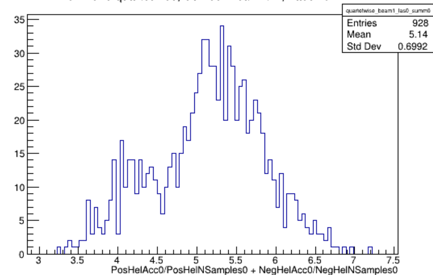
Run 4379 quartetwise, Sums0: Beam ON, Laser OFF
