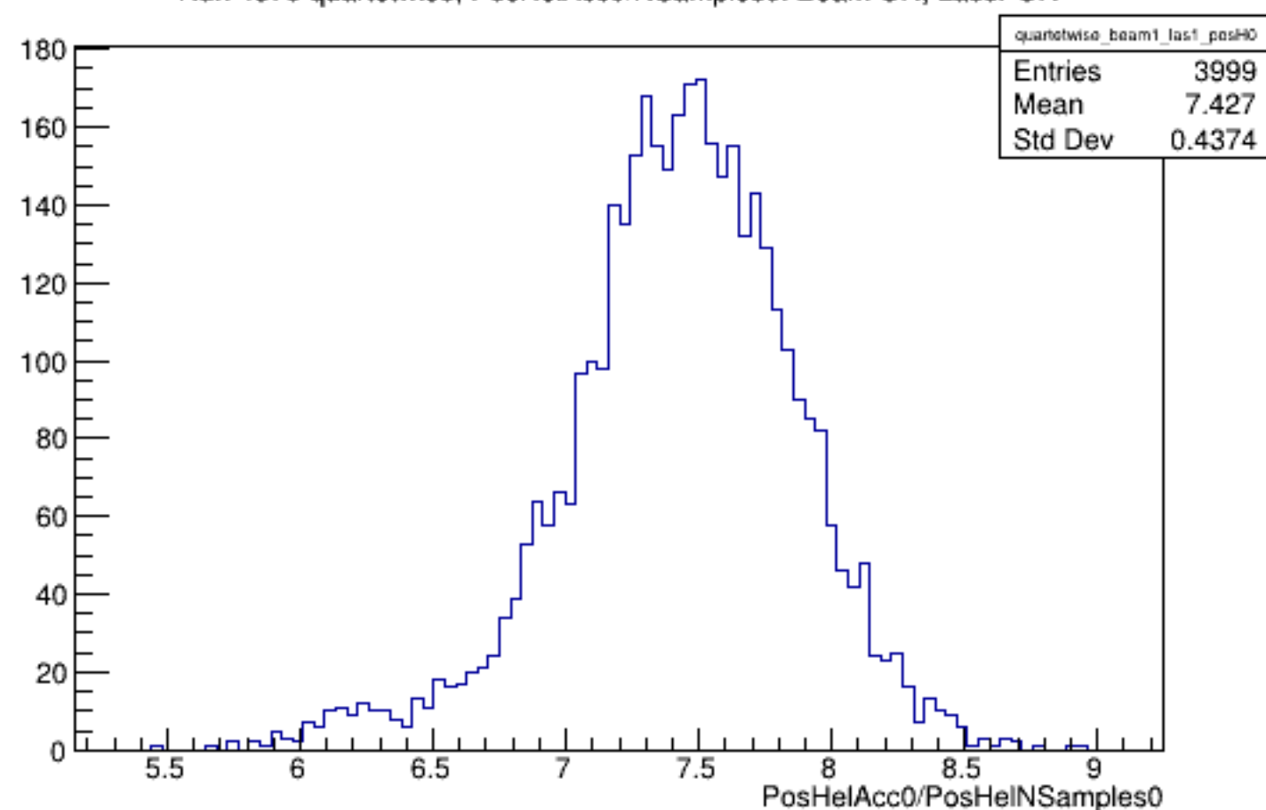
Run 4379 quartetwise, PosHelAcc0/NSamples0: Beam ON, Laser ON
