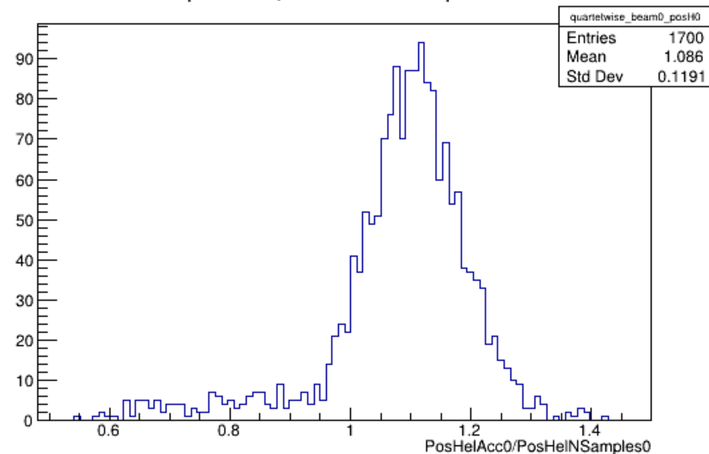
Run 4379 quartetwise, PosHelAcc0/NSamples0: Beam OFF
