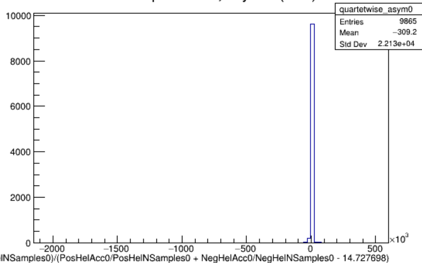
Run 4379 quartetwise, Asyms0 (Raw): All
