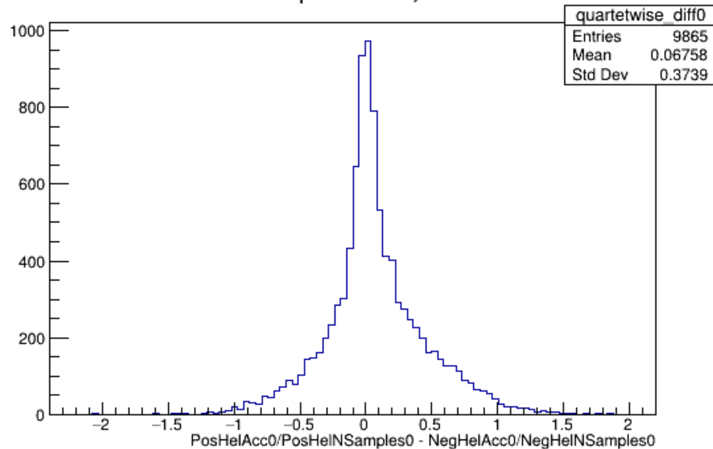
Run 4379 quartetwise, Diffs0: All
