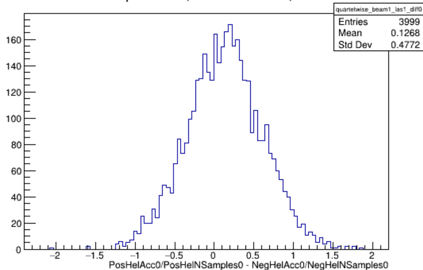
Run 4379 quartetwise, Diffs0: Beam ON, Laser ON
