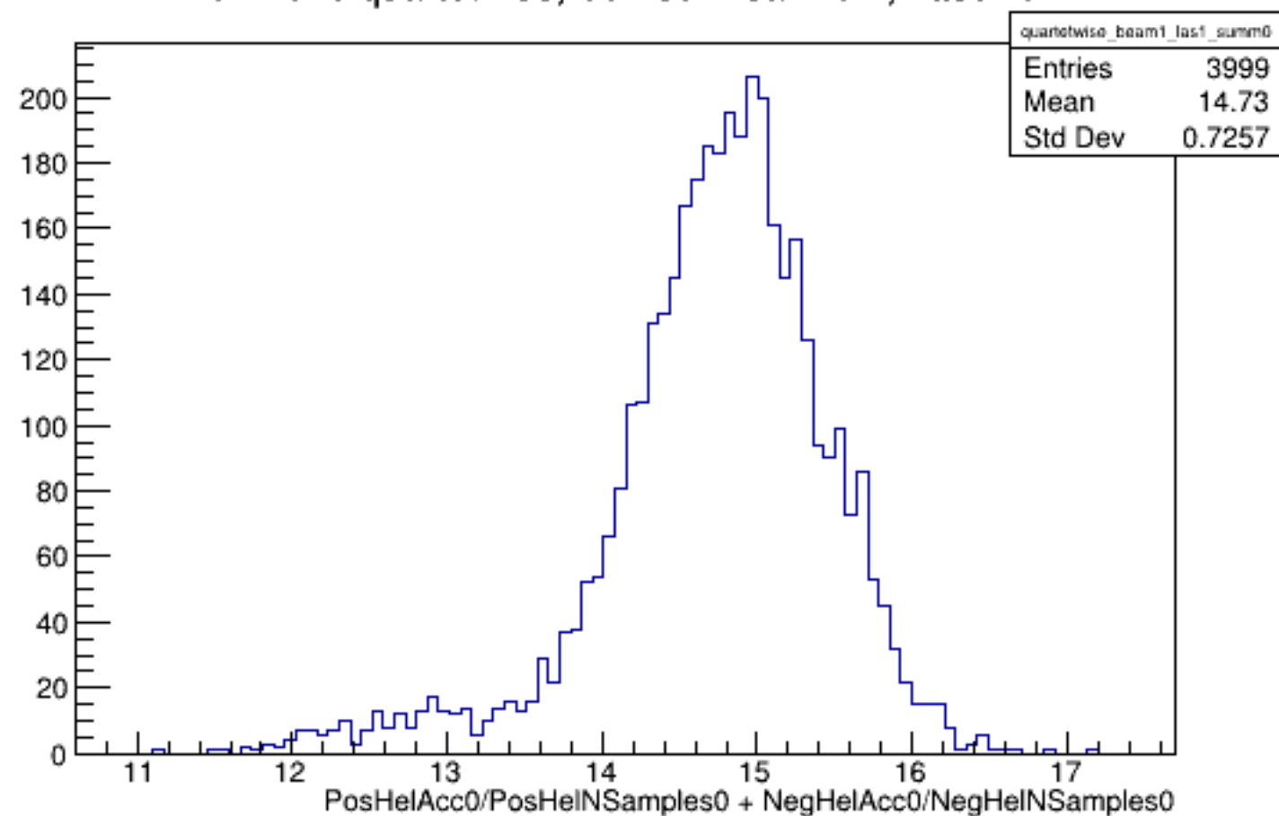
Run 4379 quartetwise, Sums0: Beam ON, Laser ON
