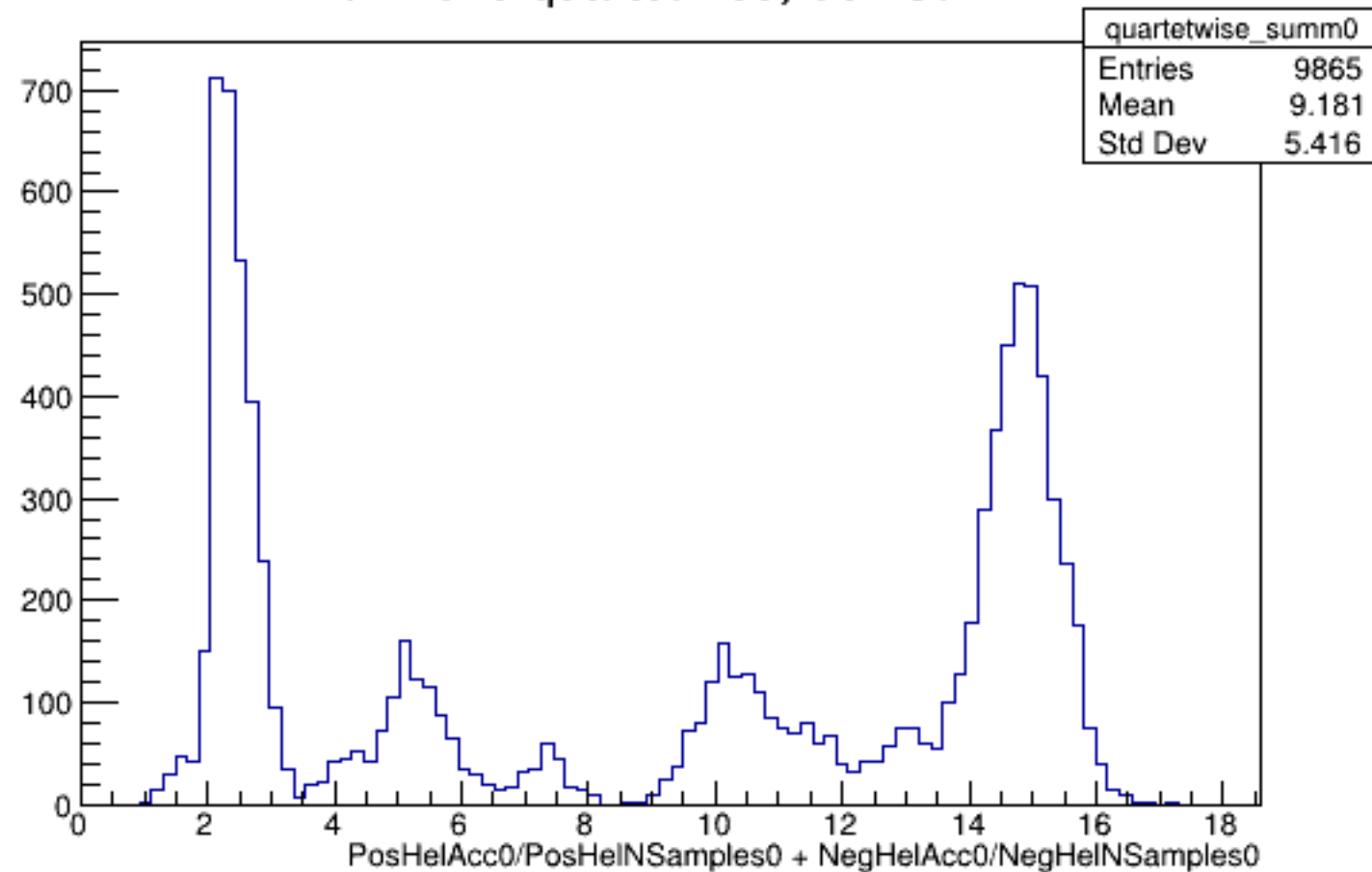
Run 4379 quartetwise, Sums0: All
