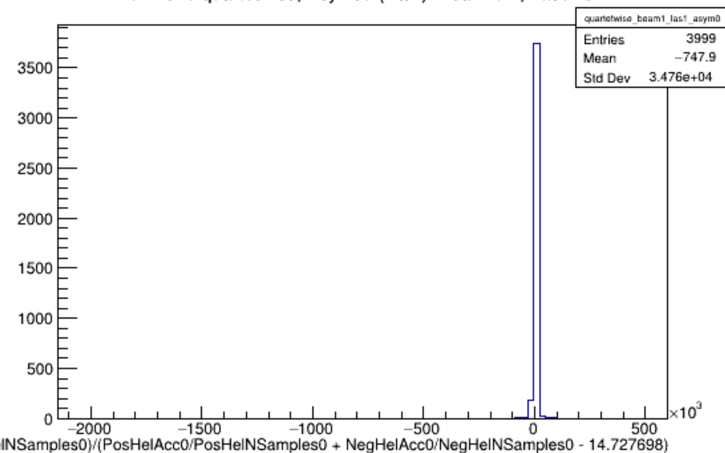
Run 4379 quartetwise, Asyms0 (Raw): Beam ON, Laser ON
