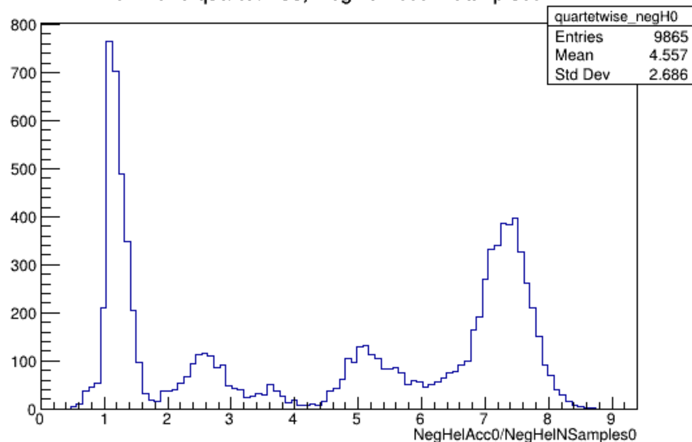
Run 4379 quartetwise, NegHelAcc0/NSamples0: All
