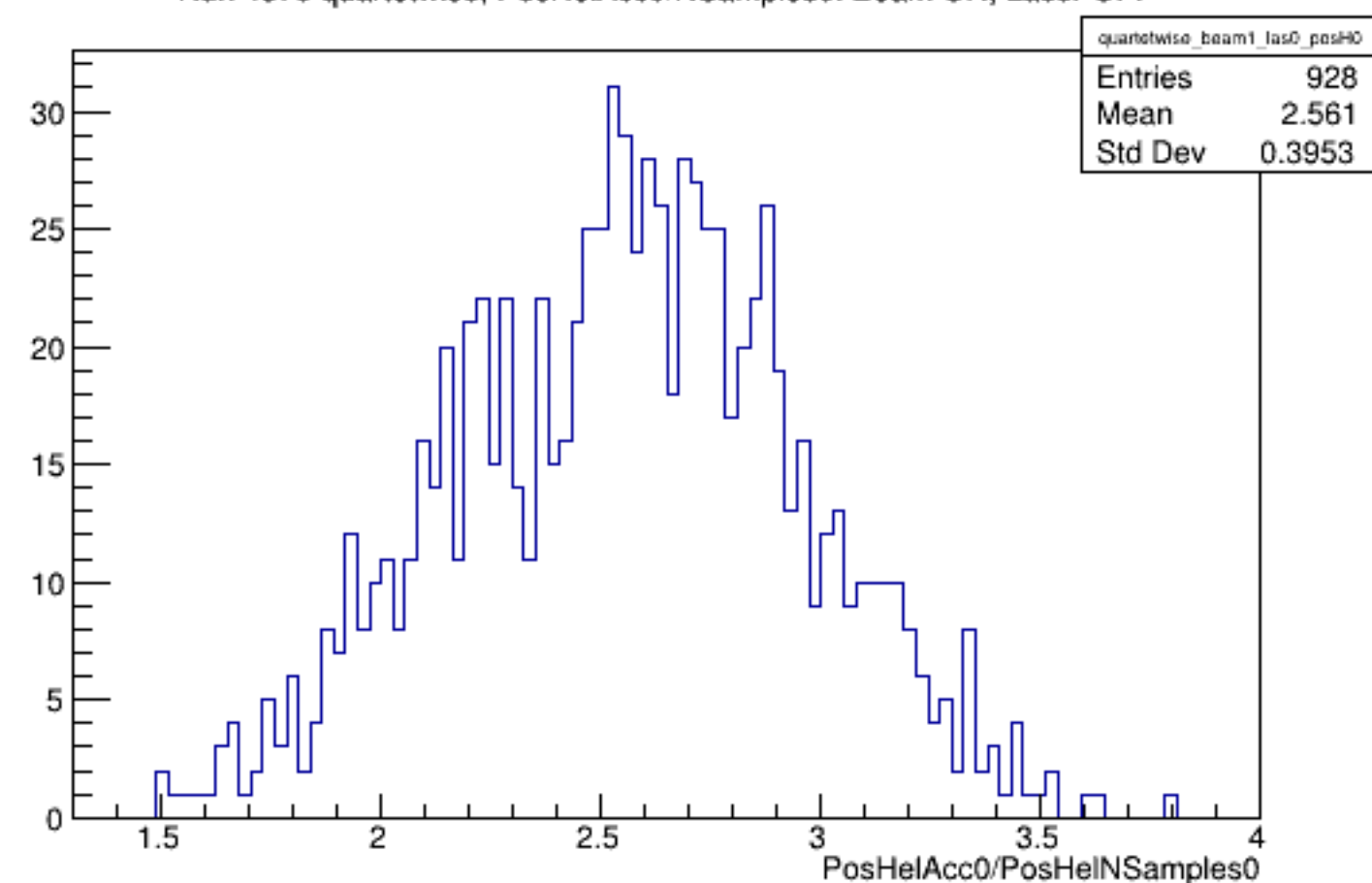
Run 4379 quartetwise, PosHelAcc0/NSamples0: Beam ON, Laser OFF
