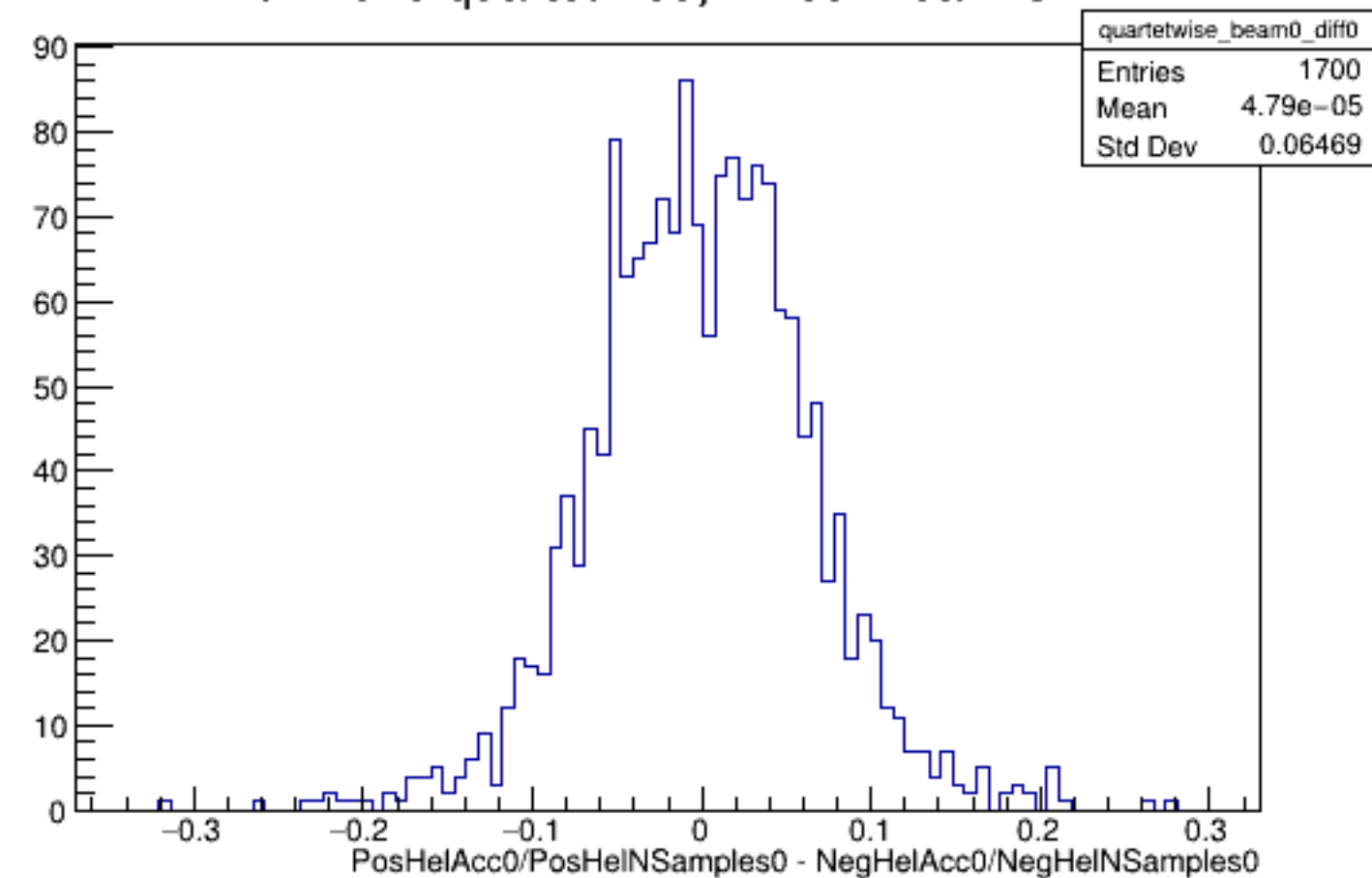
Run 4379 quartetwise, Diffs0: Beam OFF
