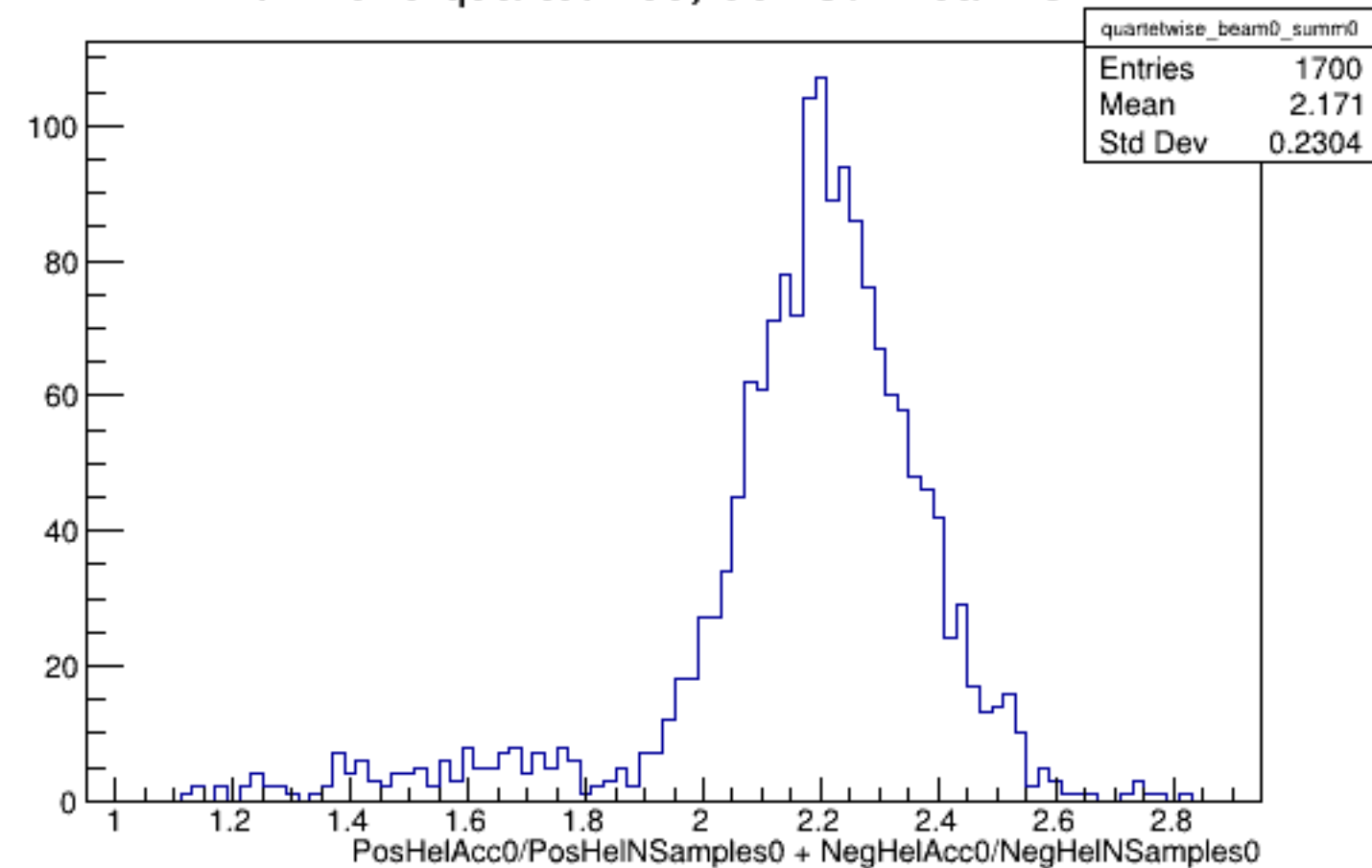
Run 4379 quartetwise, Sums0: Beam OFF
