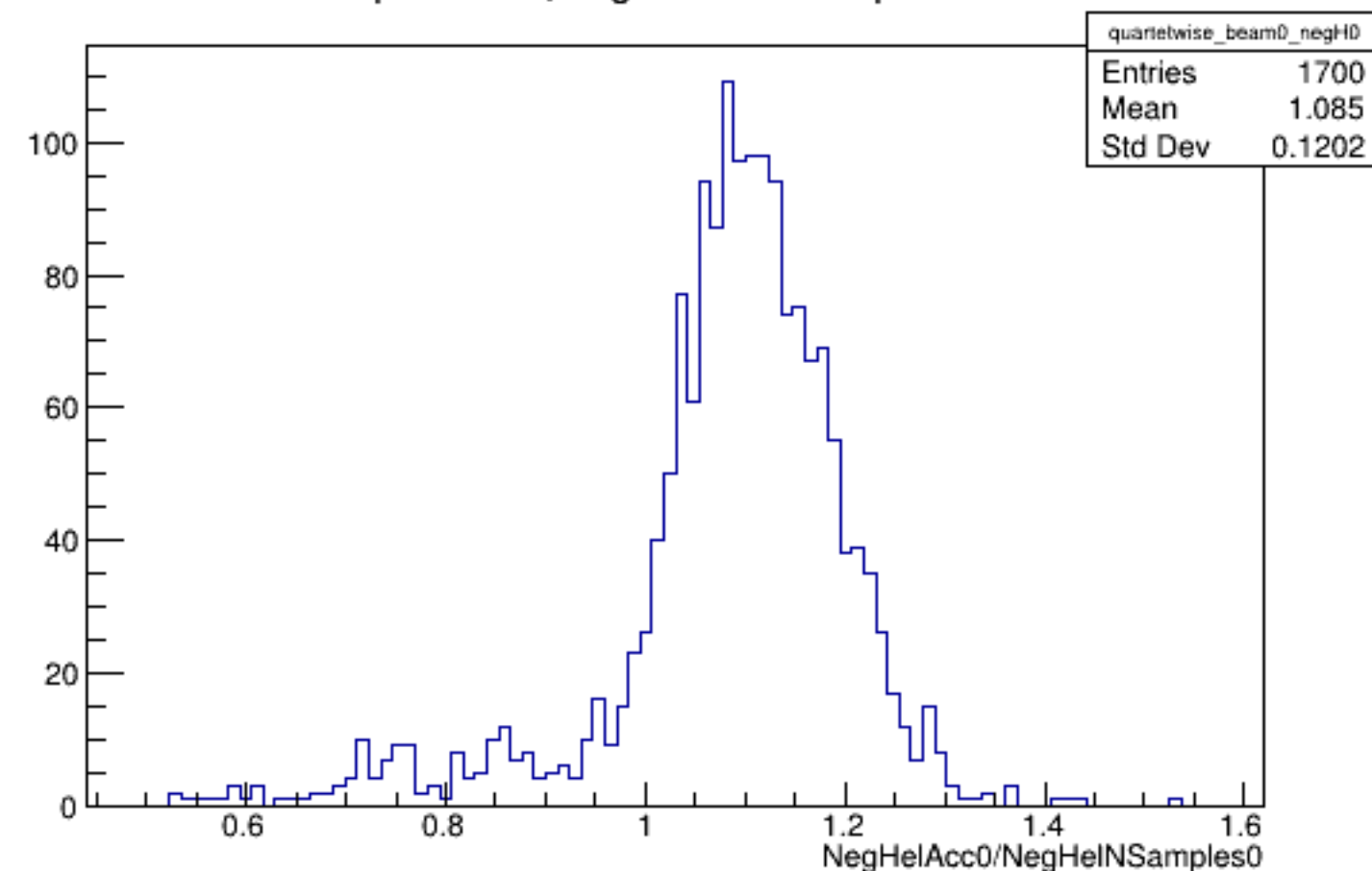
Run 4379 quartetwise, NegHelAcc0/NSamples0: Beam OFF
