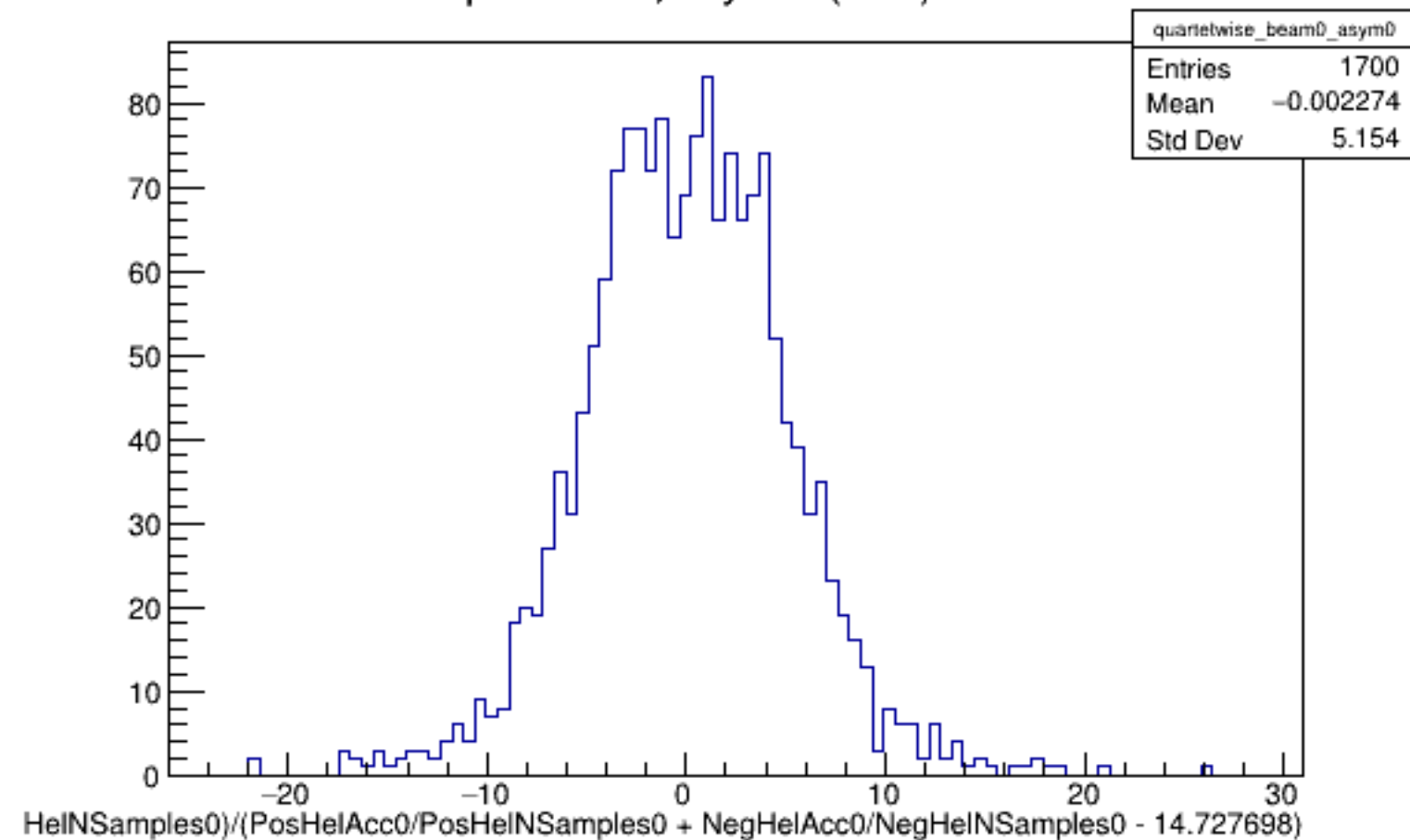
Run 4379 quartetwise, Asyms0 (Raw): Beam OFF
