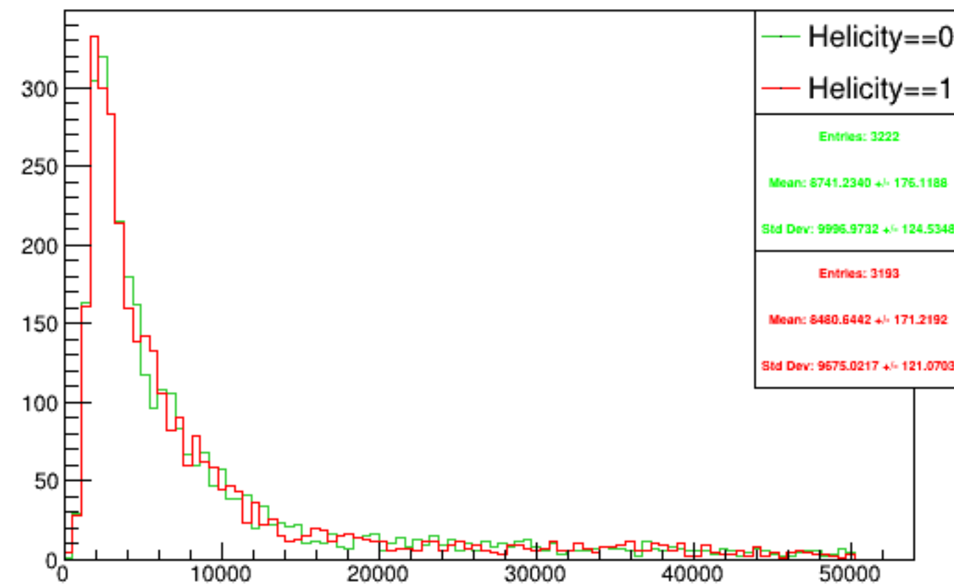
Run 4379 triggerwise, sums: Beam ON, Laser OFF
