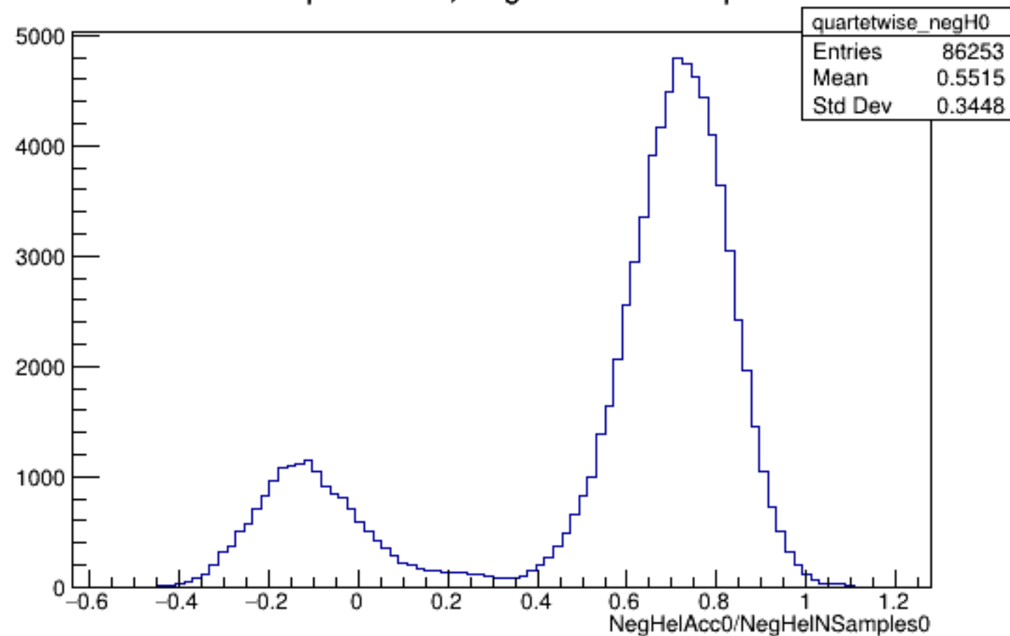
Run 4387 quartetwise, NegHelAcc0/NSamples0: All
