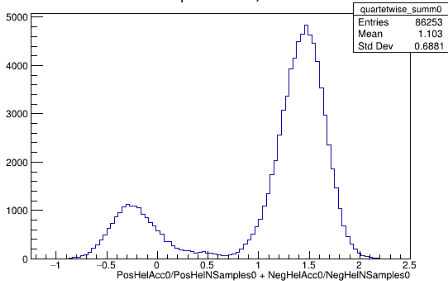
Run 4387 quartetwise, Sums0: All
