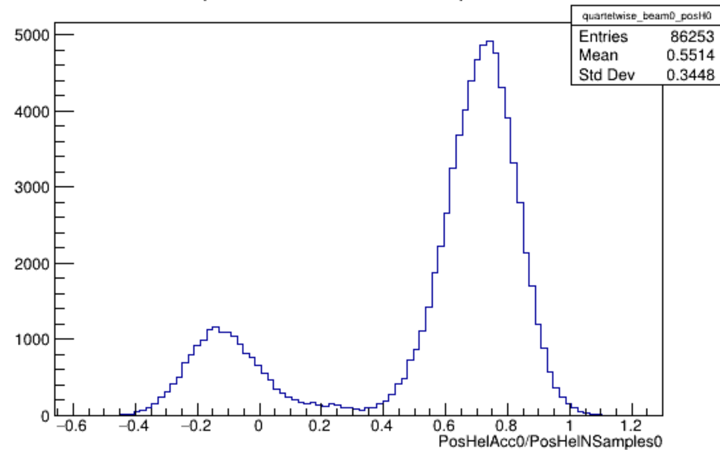
Run 4387 quartetwise, PosHelAcc0/NSamples0: Beam OFF
