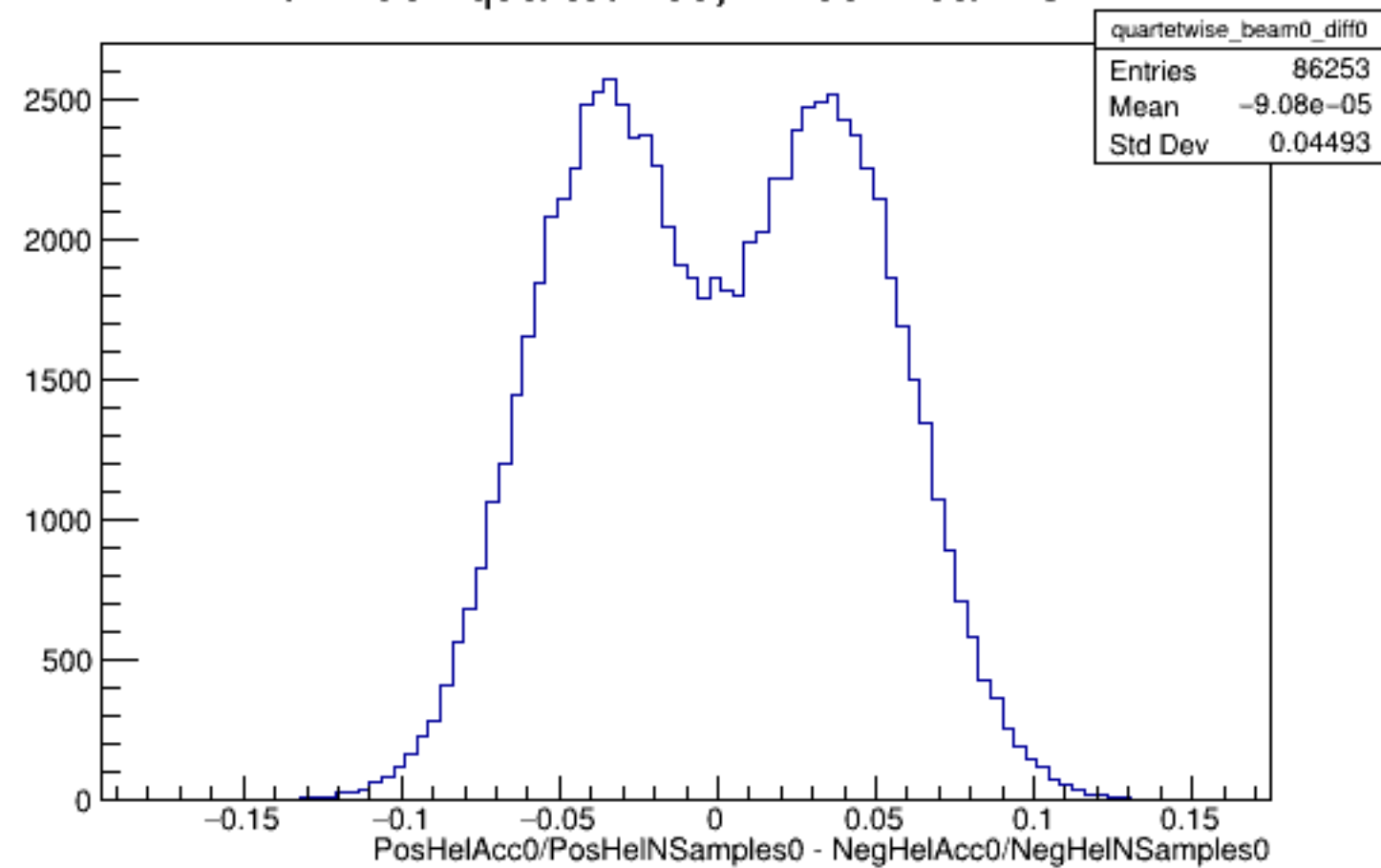
Run 4387 quartetwise, Diffs0: Beam OFF
