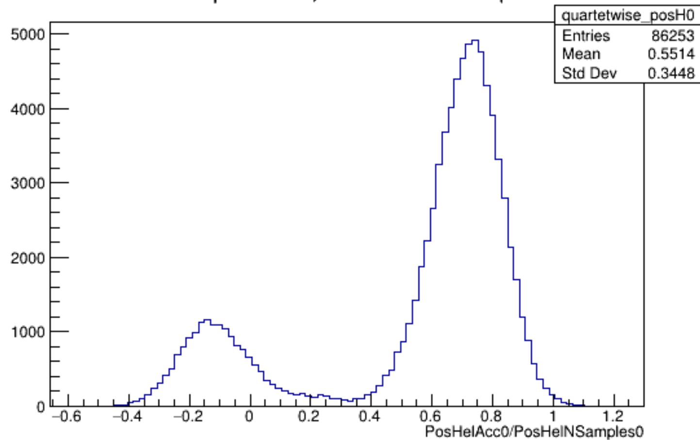
Run 4387 quartetwise, PosHelAcc0/NSamples0: All
