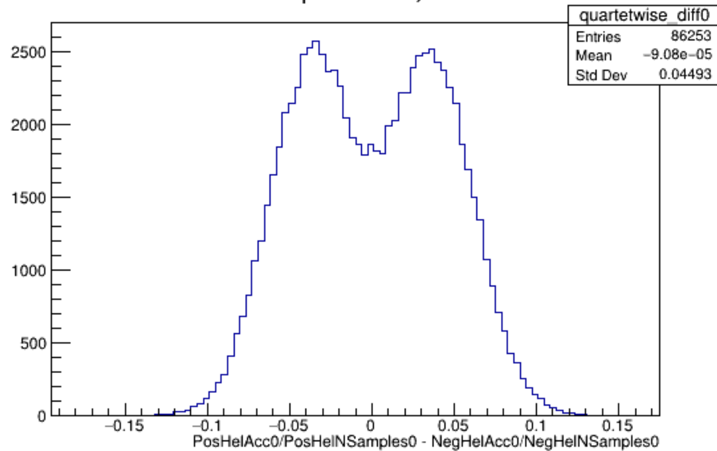
Run 4387 quartetwise, Diffs0: All
