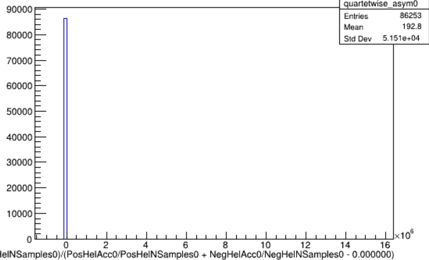
Run 4387 quartetwise, Asyms0 (Raw): All
