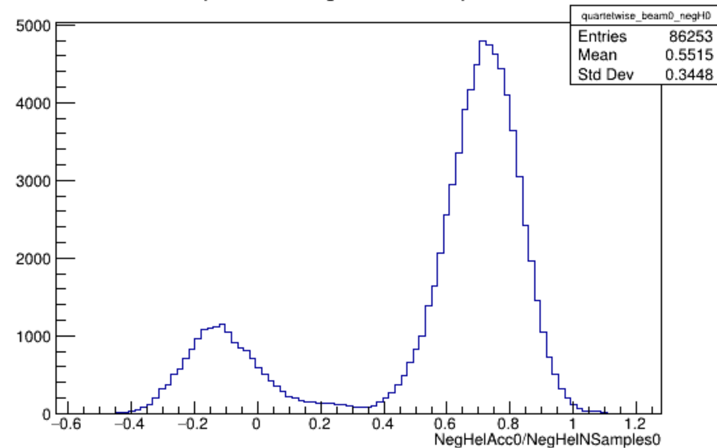
Run 4387 quartetwise, NegHelAcc0/NSamples0: Beam OFF
