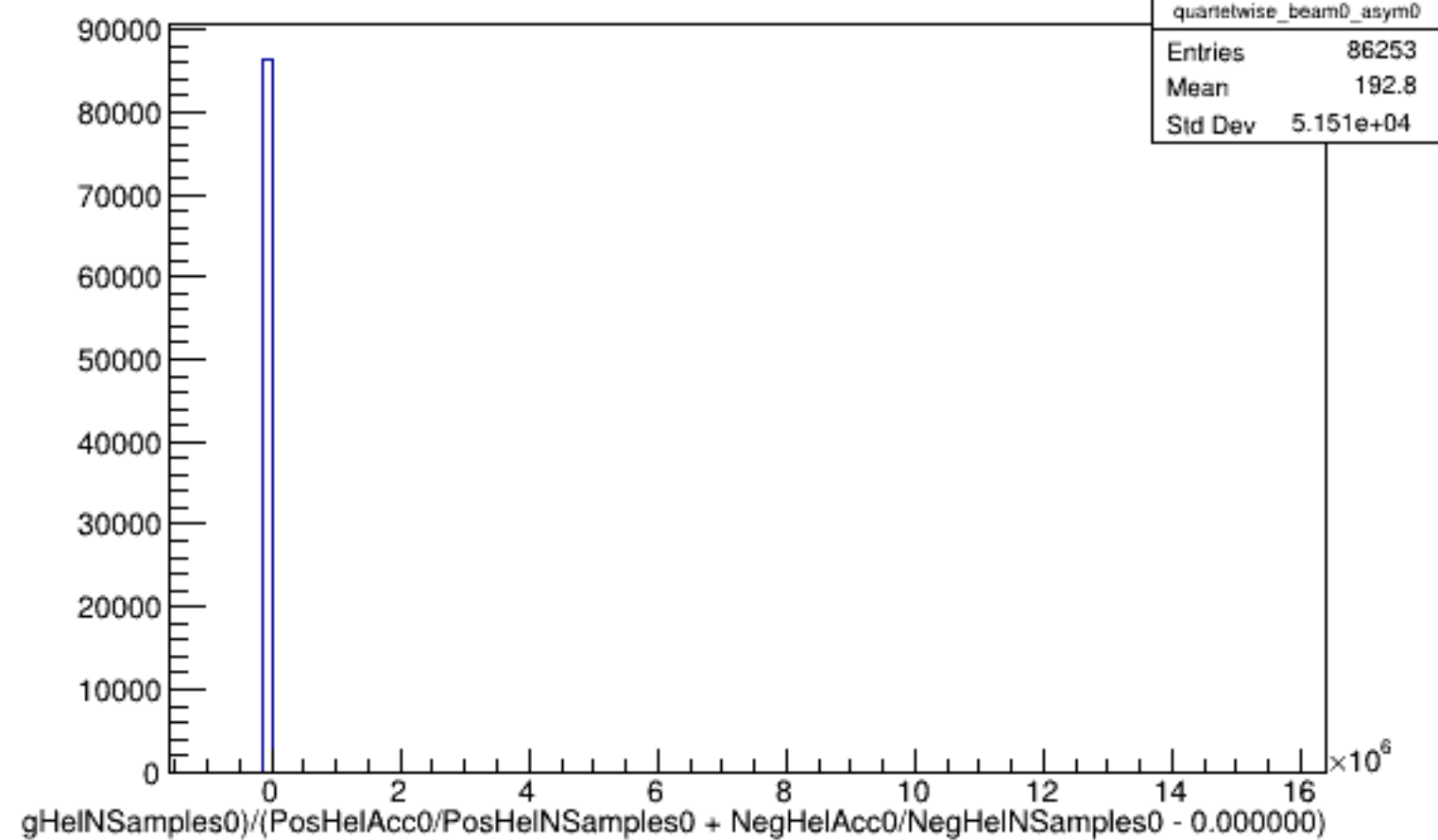
Run 4387 quartetwise, Asyms0 (Raw): Beam OFF
