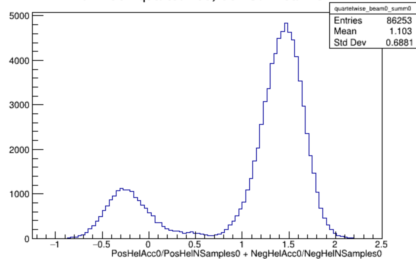
Run 4387 quartetwise, Sums0: Beam OFF
