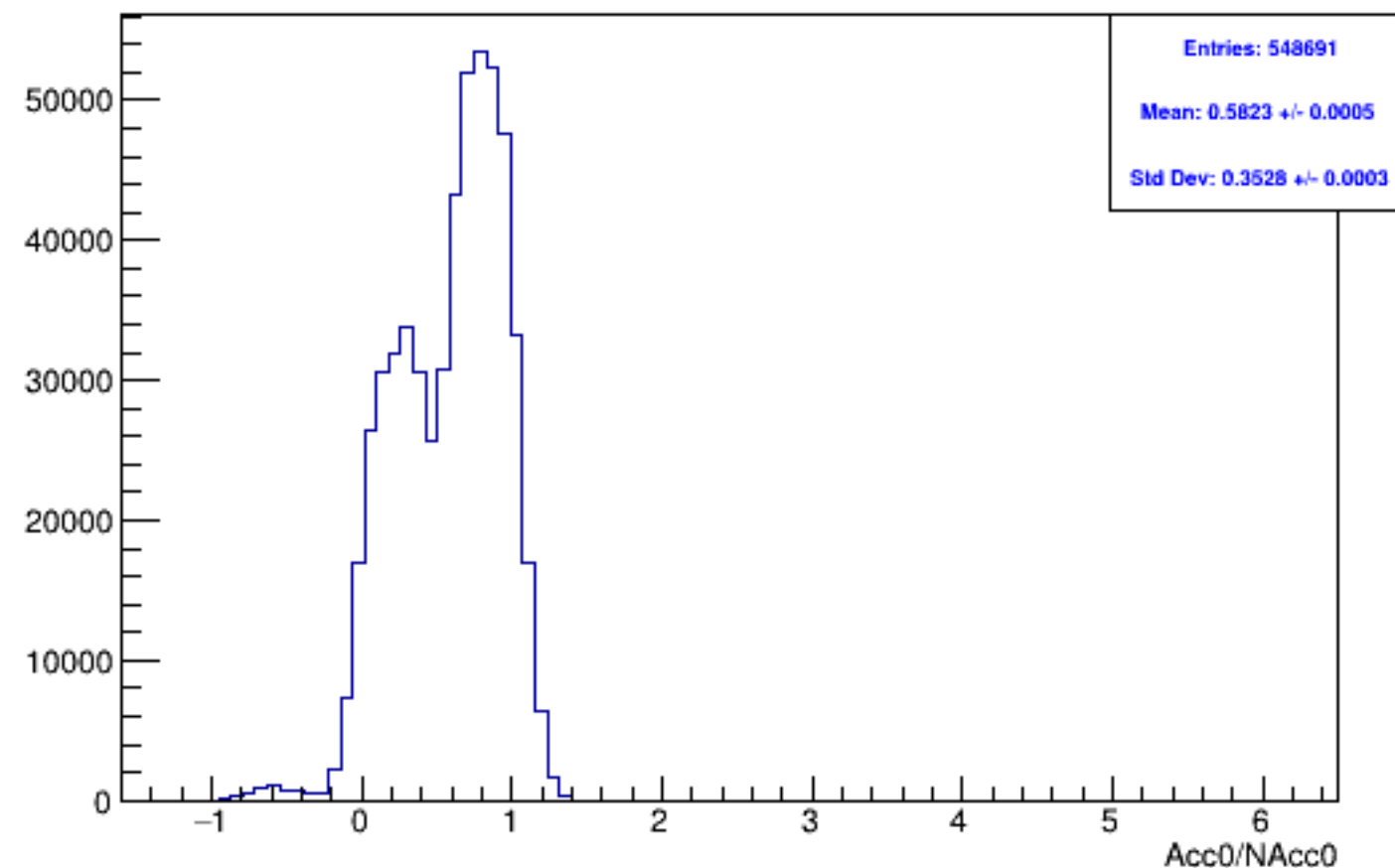
Run 4403 mpwise, acc0: Beam OFF
