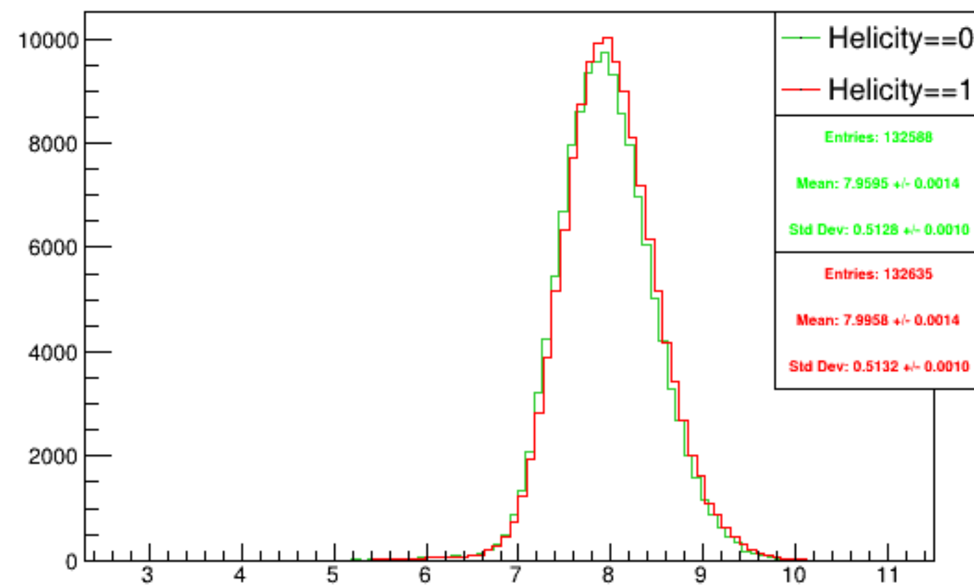
Run 4403 mpwise, acc0: Beam ON, Laser OFF
