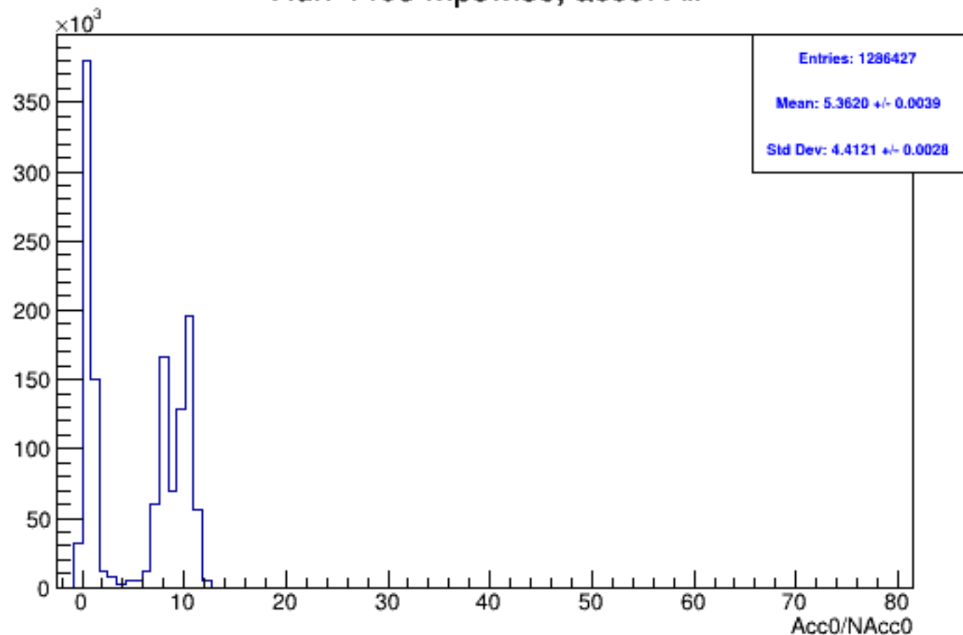
Run 4403 mpwise, acc0: All
