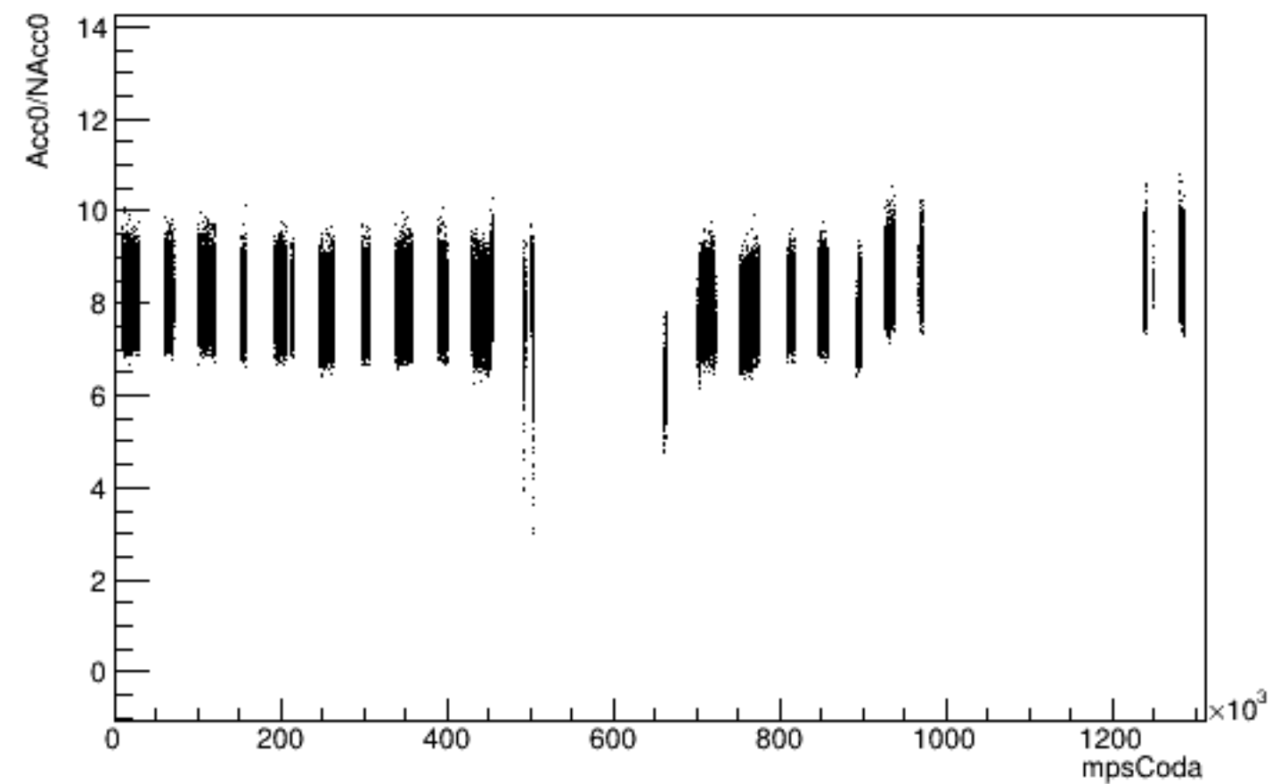
Run 4403 mpwise, Acc0/NAcc0:mpsCoda, beam ON, laser OFF
