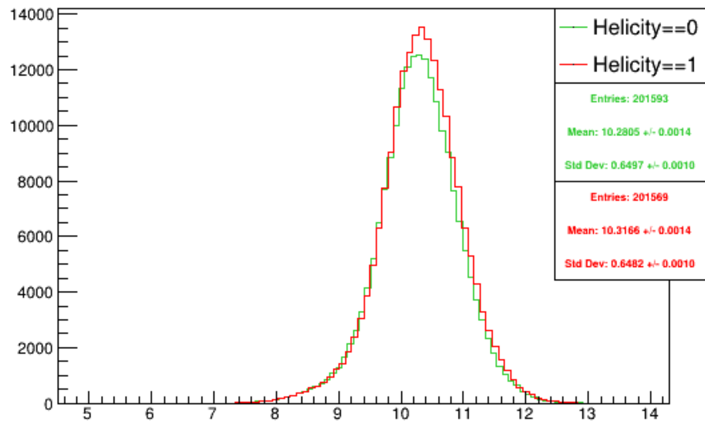
Run 4403 mpwise, acc0: Beam ON, Laser ON
