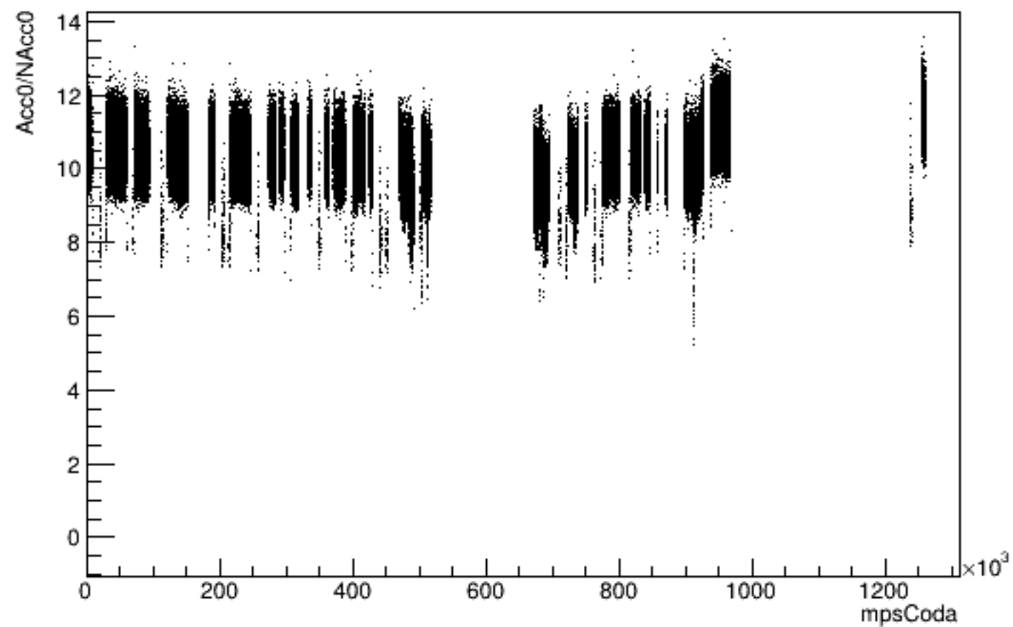
Run 4403 mpwise, Acc0/NAcc0:mpsCoda, beam ON, laser ON
