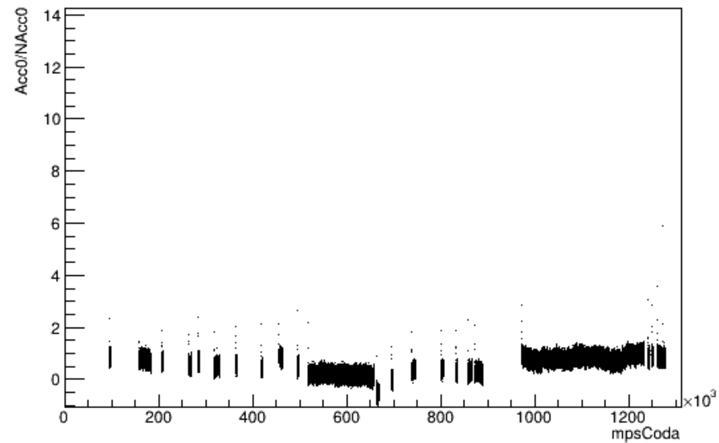
Run 4403 mpwise, Acc0/NAcc0:mpsCoda, beam OFF
