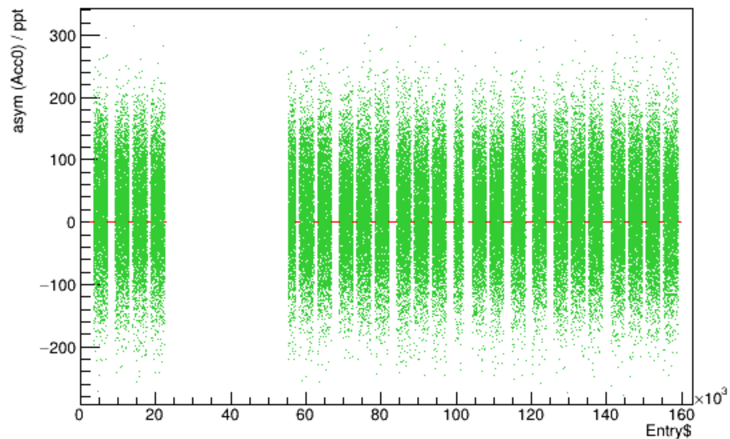
Run 4411 quartetwise, asym0sub vs time
