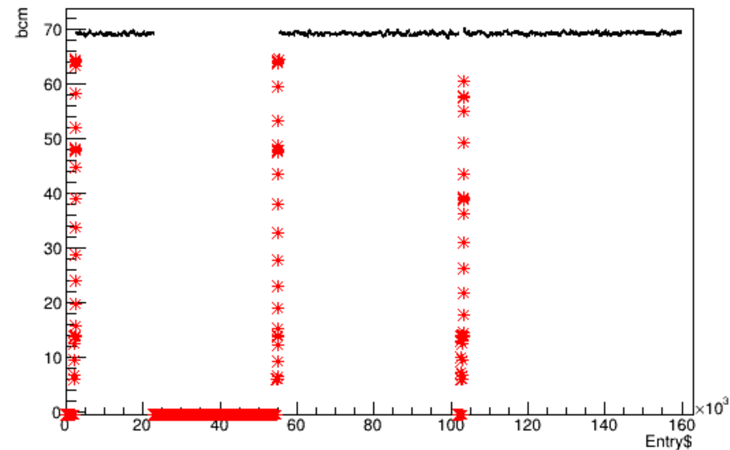
Run 4411 quartetwise, bcm vs time
