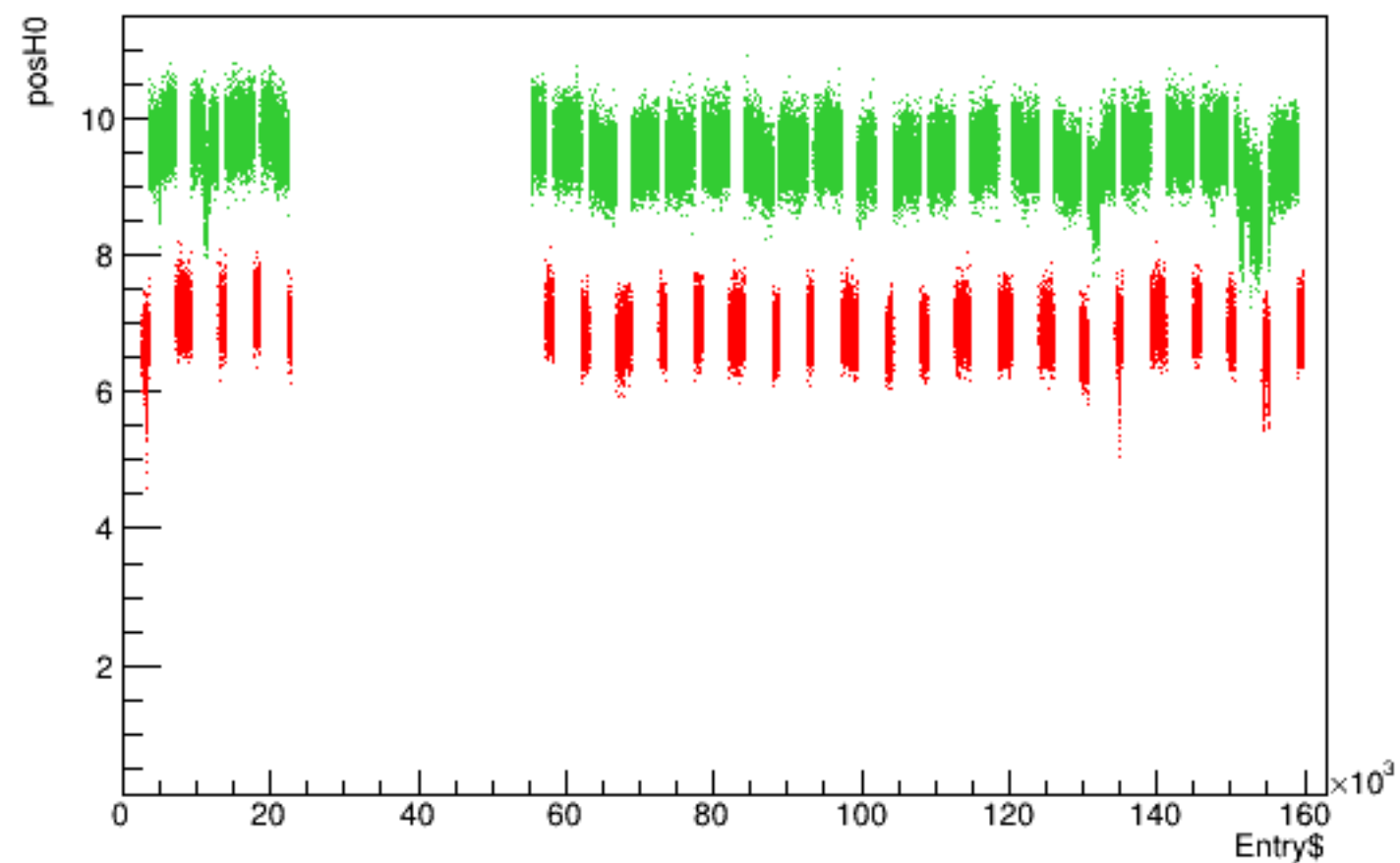
Run 4411 quartetwise, posH0 vs time
