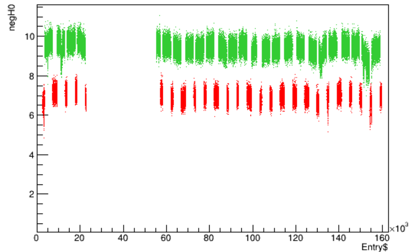
Run 4411 quartetwise, negH0 vs time
