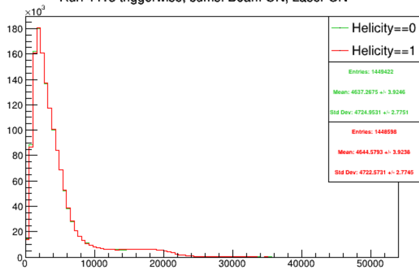
Run 4413 triggerwise, sums: Beam ON, Laser ON
