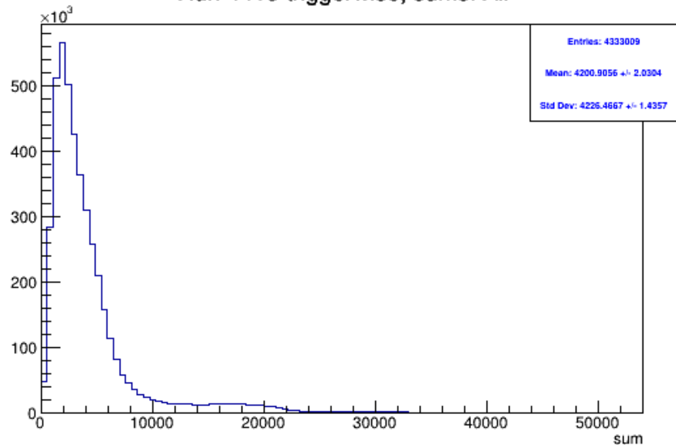
Run 4413 triggerwise, sums: All
