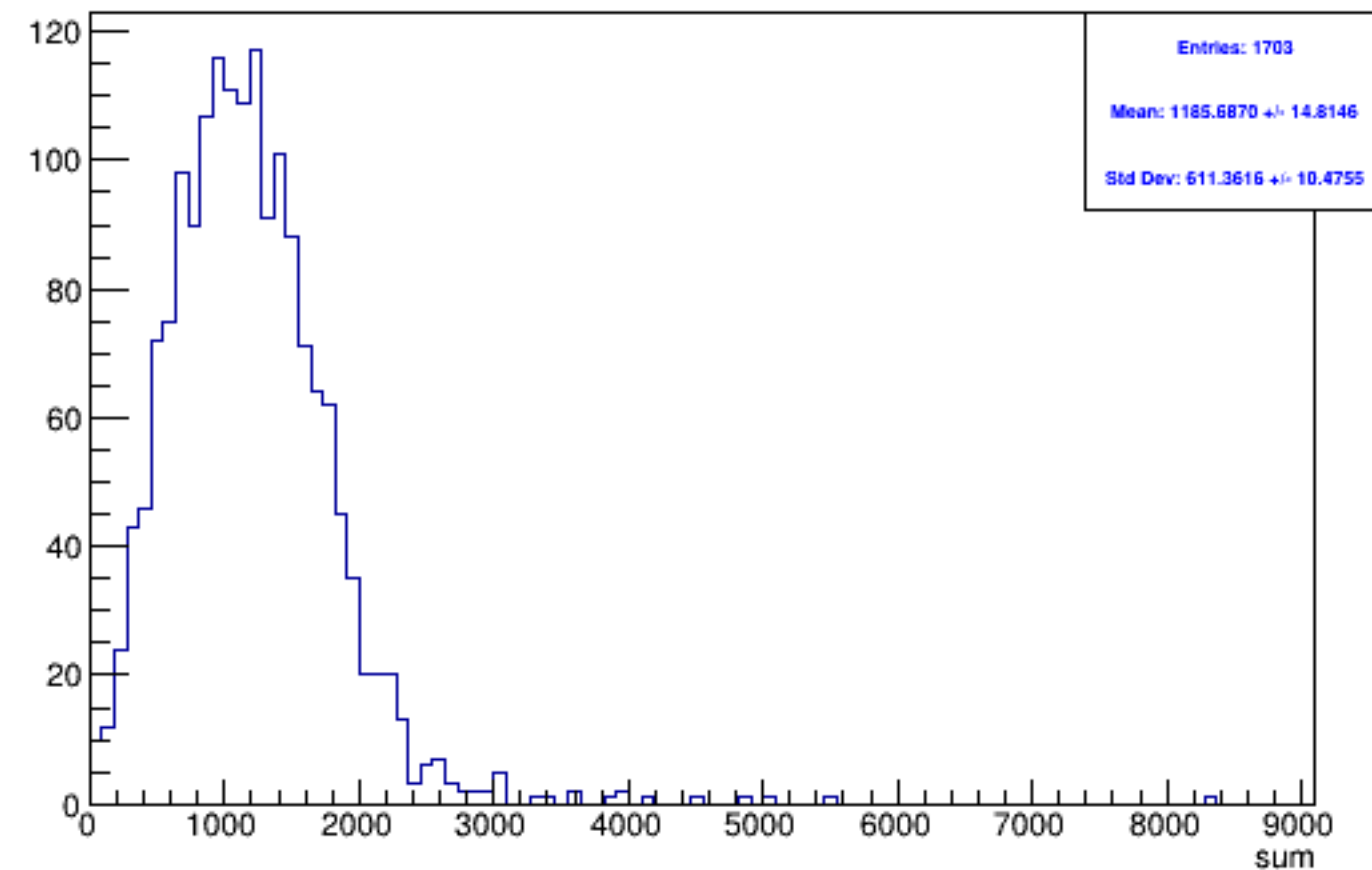
Run 4413 triggerwise, sums: Beam OFF
