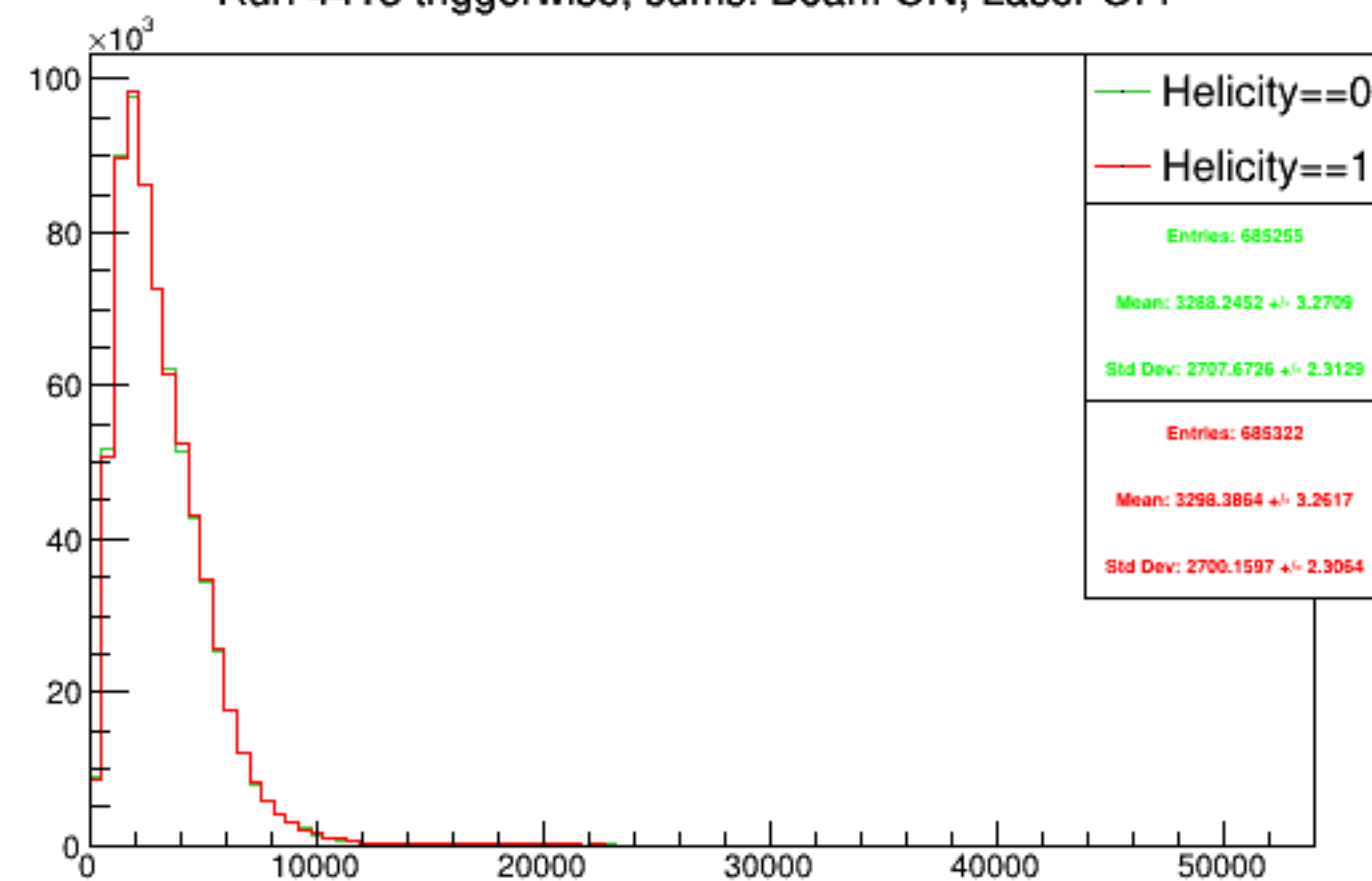
Run 4413 triggerwise, sums: Beam ON, Laser OFF
