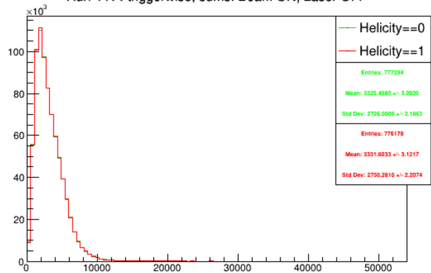
Run 4414 triggerwise, sums: Beam ON, Laser OFF
