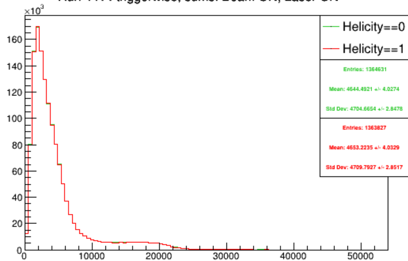
Run 4414 triggerwise, sums: Beam ON, Laser ON
