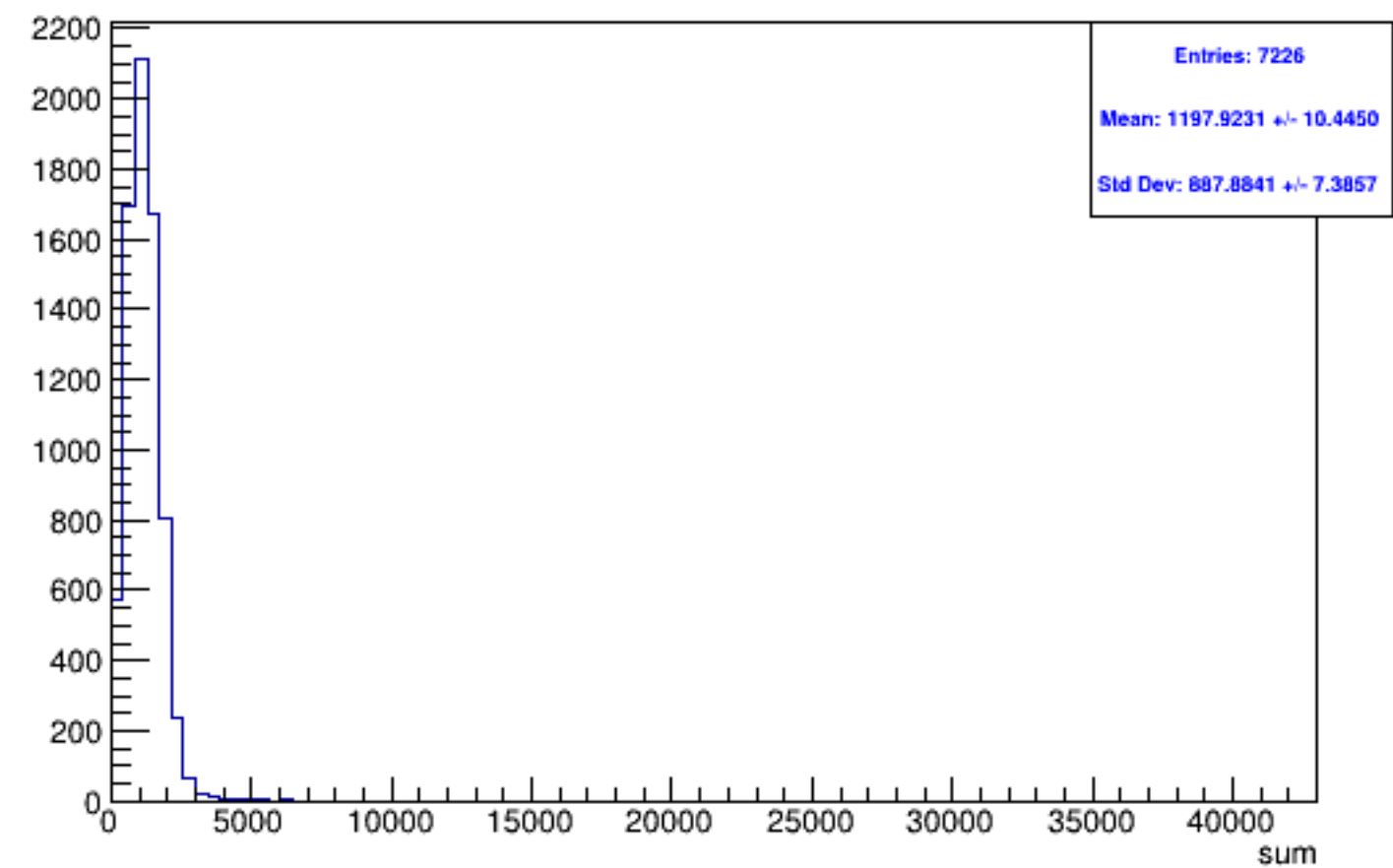
Run 4414 triggerwise, sums: Beam OFF
