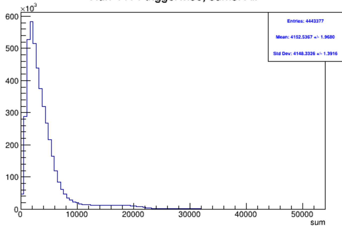
Run 4414 triggerwise, sums: All
