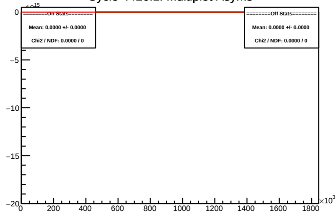
Cycle 4416.1: Multiplet Asyms
