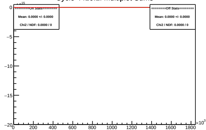
Cycle 4416.1: Multiplet Sums
