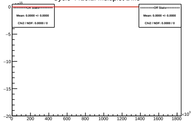
Cycle 4416.1: Multiplet Diffs
