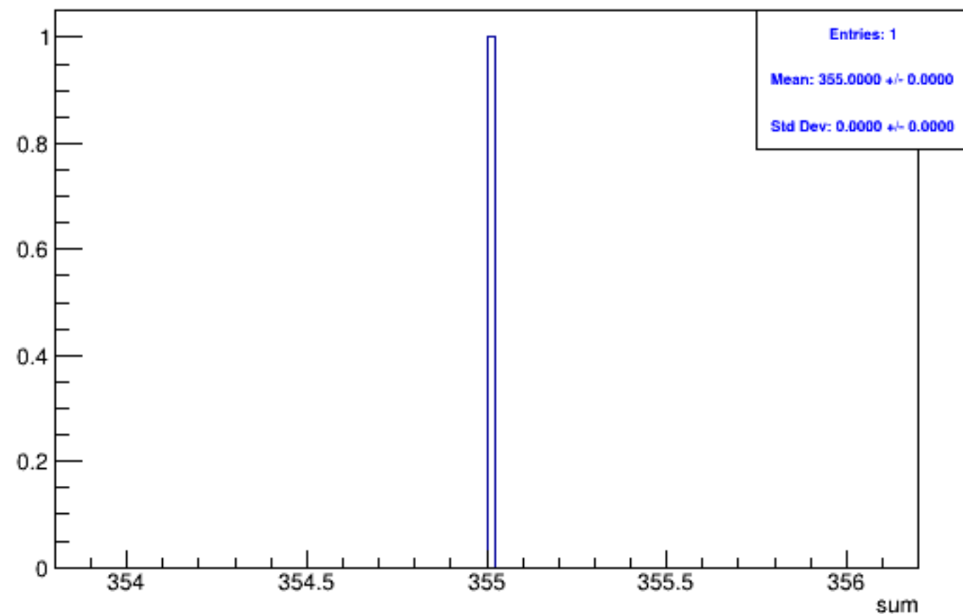
Run 4421 triggerwise, sums: Beam OFF
