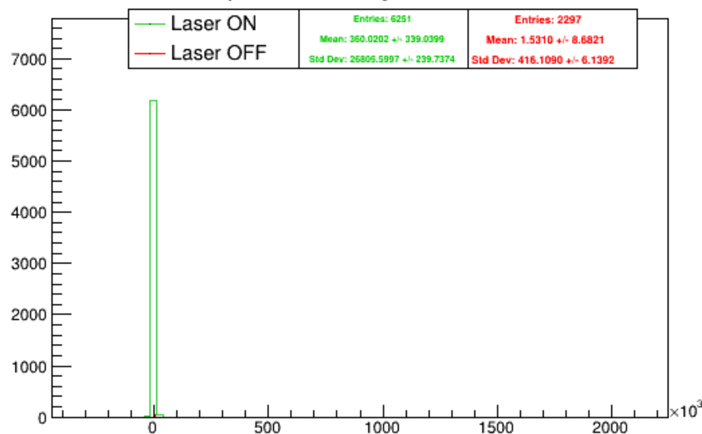
Run 4425 quartetwise, asym0sub: Beam ON
