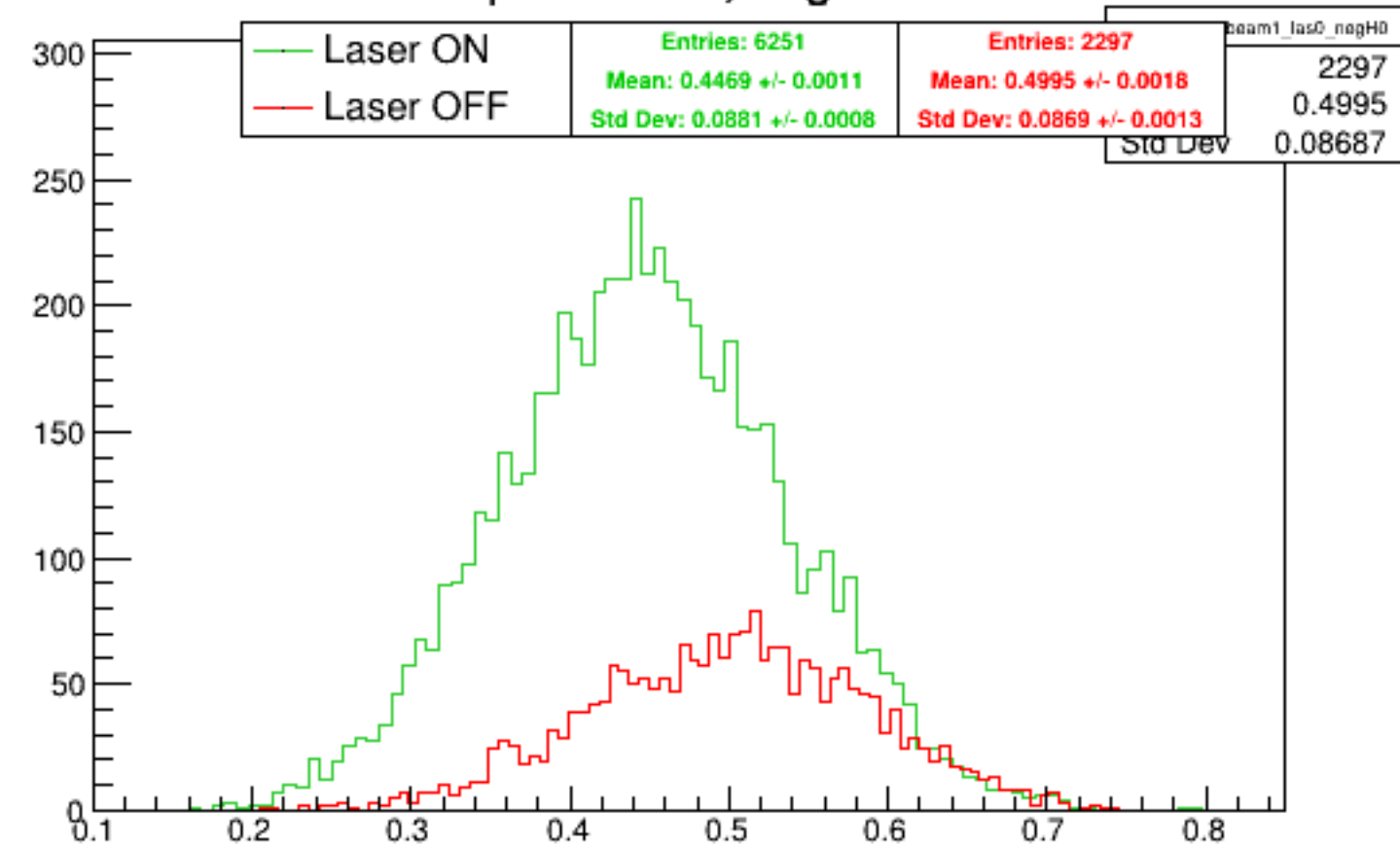
Run 4425 quartetwise, negH0: Beam ON
