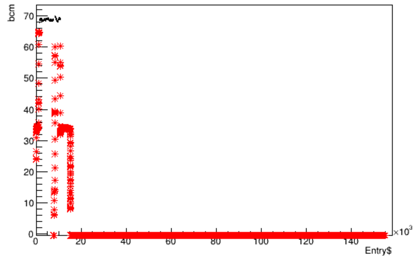
Run 4425 quartetwise, bcm vs time
