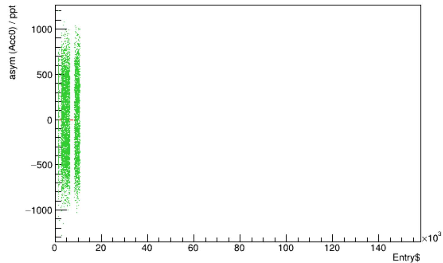
Run 4425 quartetwise, asym0sub vs time
