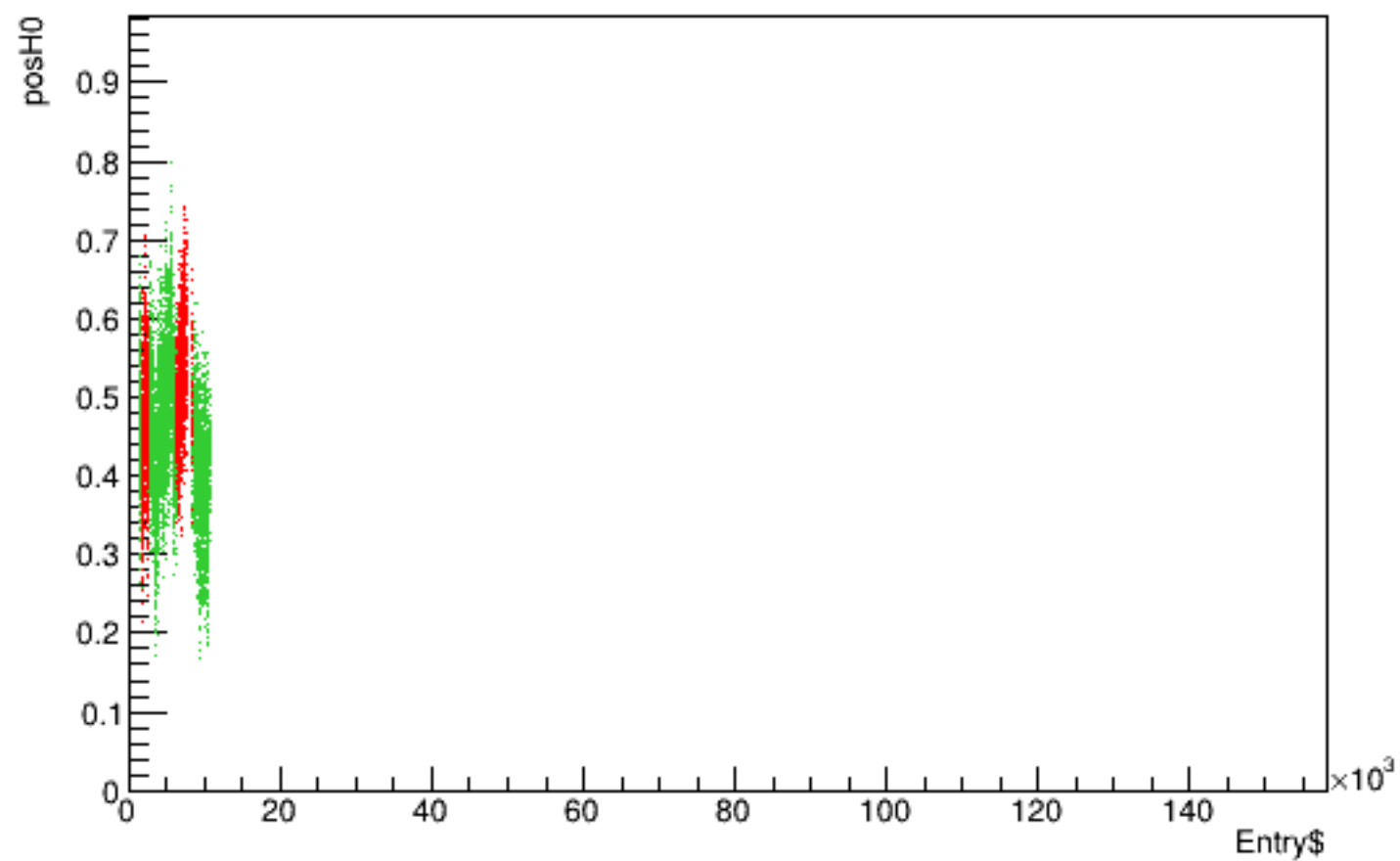
Run 4425 quartetwise, posH0 vs time
