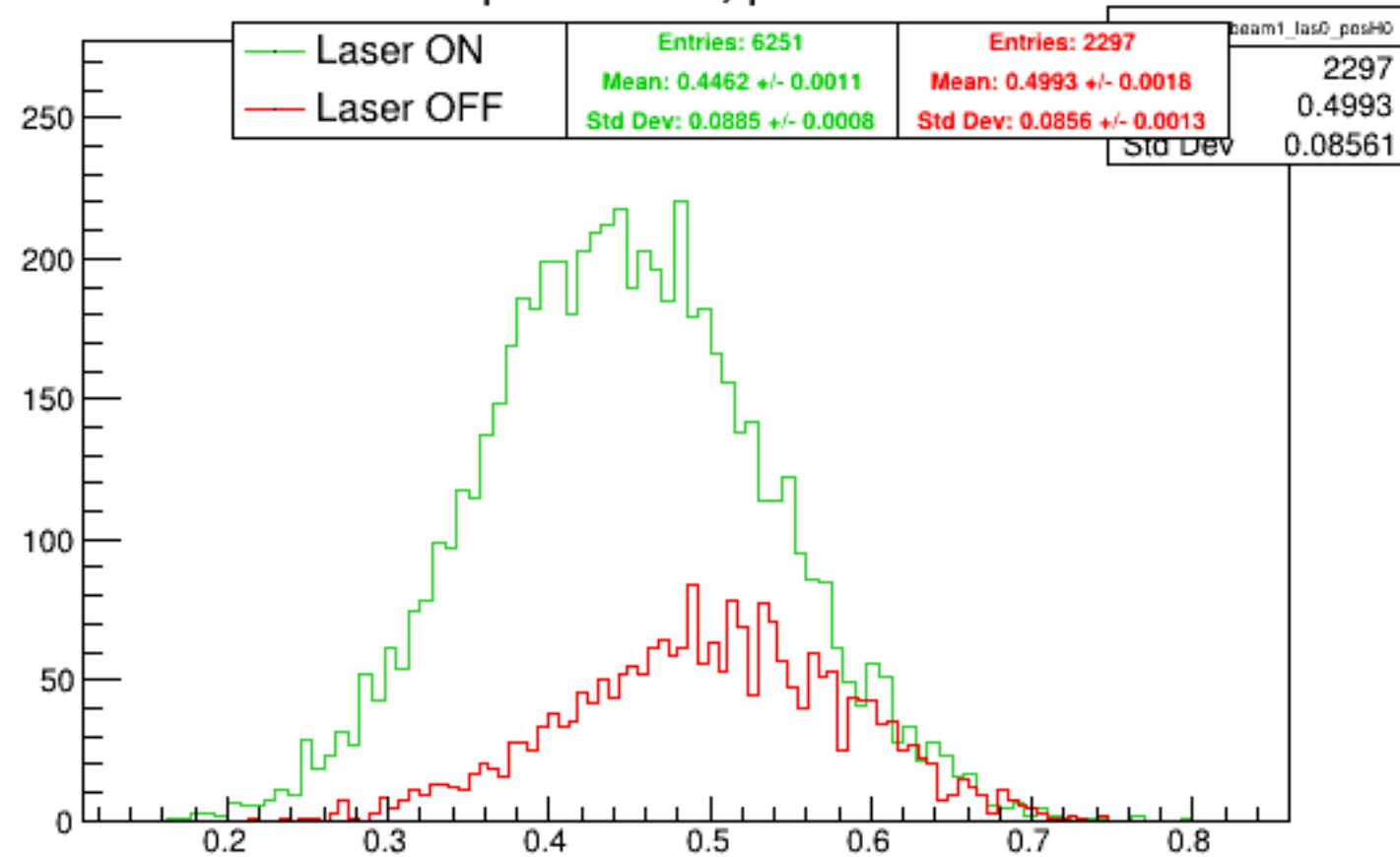
Run 4425 quartetwise, posH0: Beam ON
