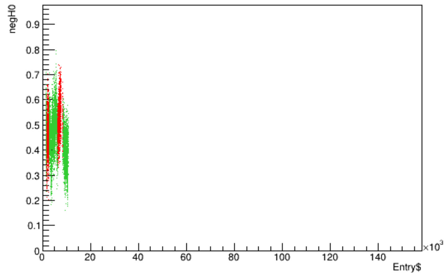
Run 4425 quartetwise, negH0 vs time
