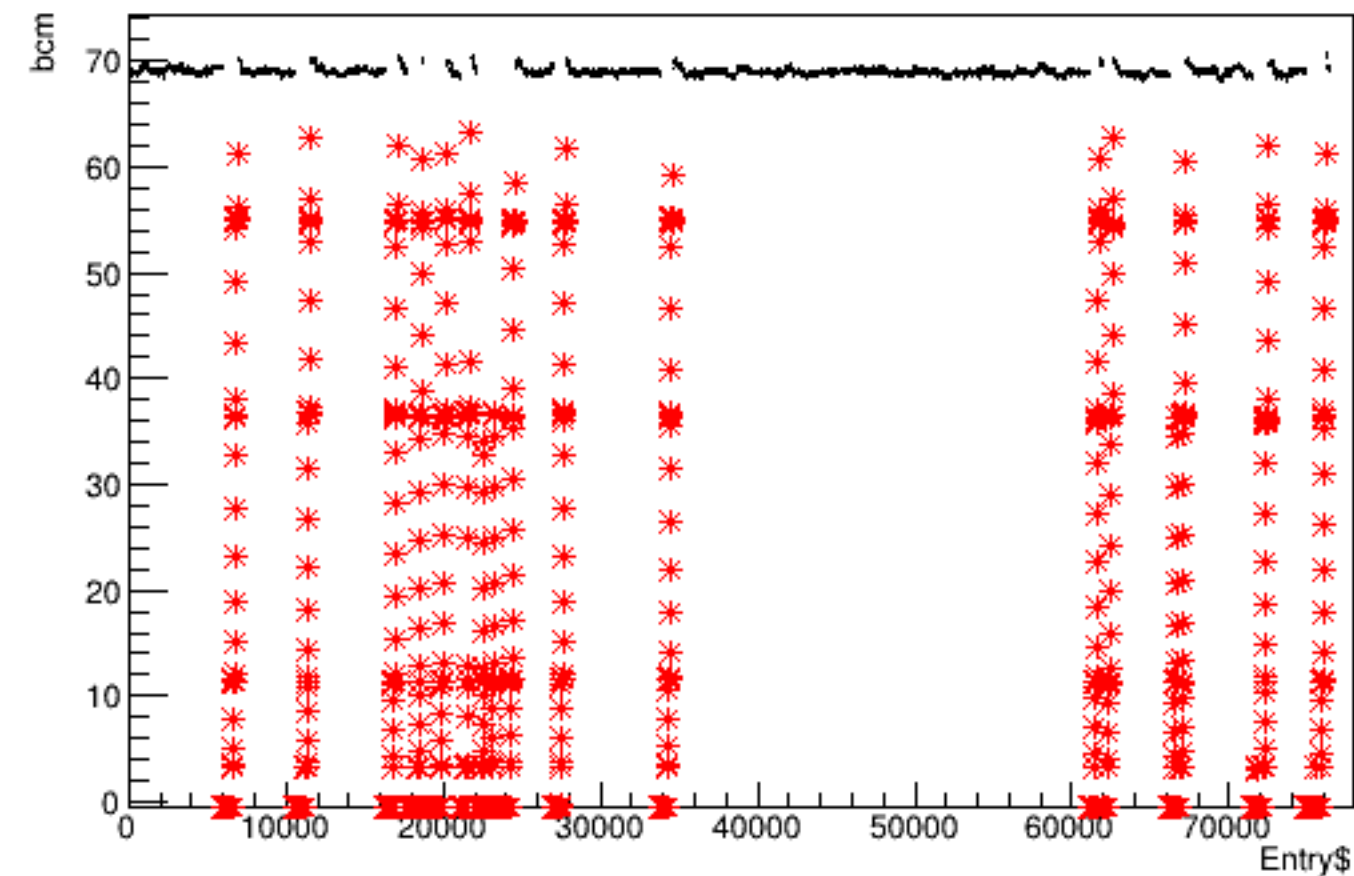
Run 4431 quartetwise, bcm vs time
