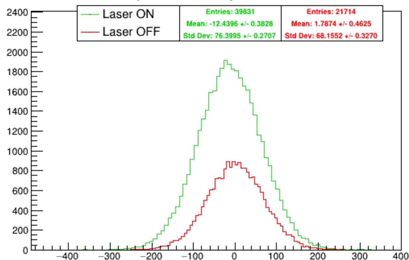
Run 4431 quartetwise, asym0sub: Beam ON
