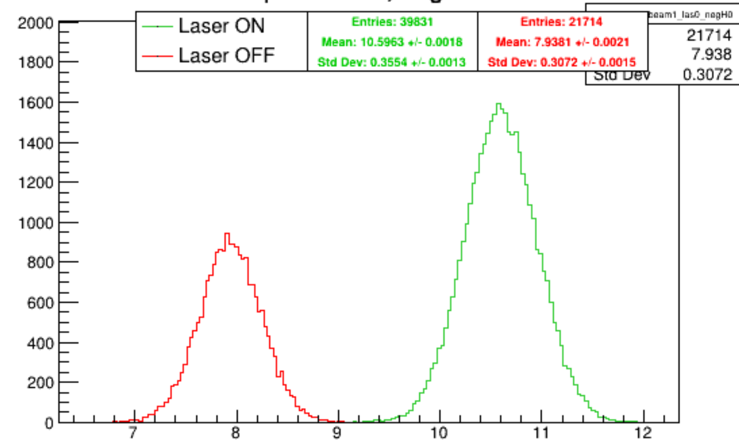
Run 4431 quartetwise, negH0: Beam ON
