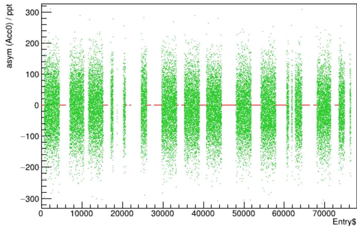
Run 4431 quartetwise, asym0sub vs time
