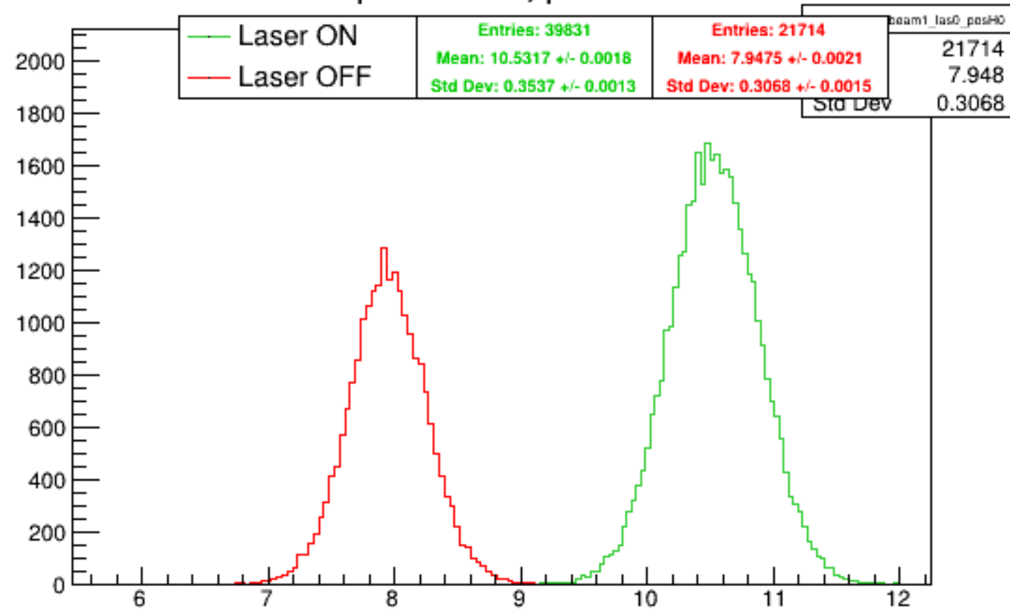
Run 4431 quartetwise, posH0: Beam ON
