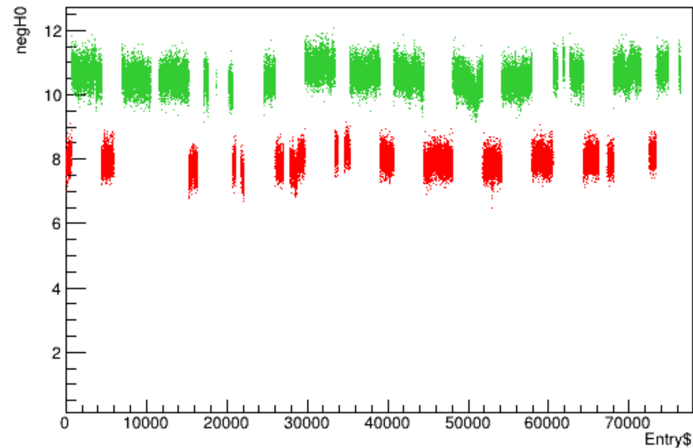
Run 4431 quartetwise, negH0 vs time
