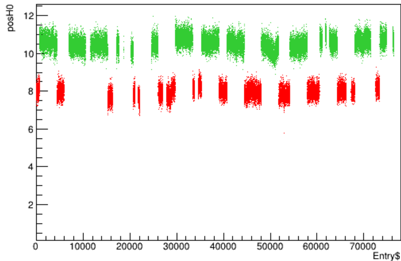
Run 4431 quartetwise, posH0 vs time
