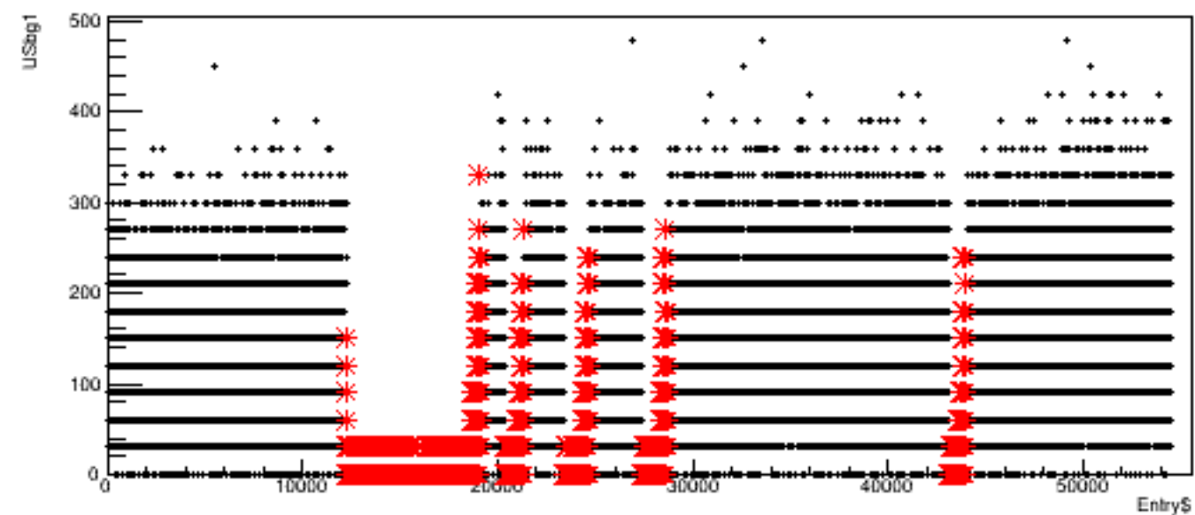
Run 4437, quartetwise: USbg1 vs time
