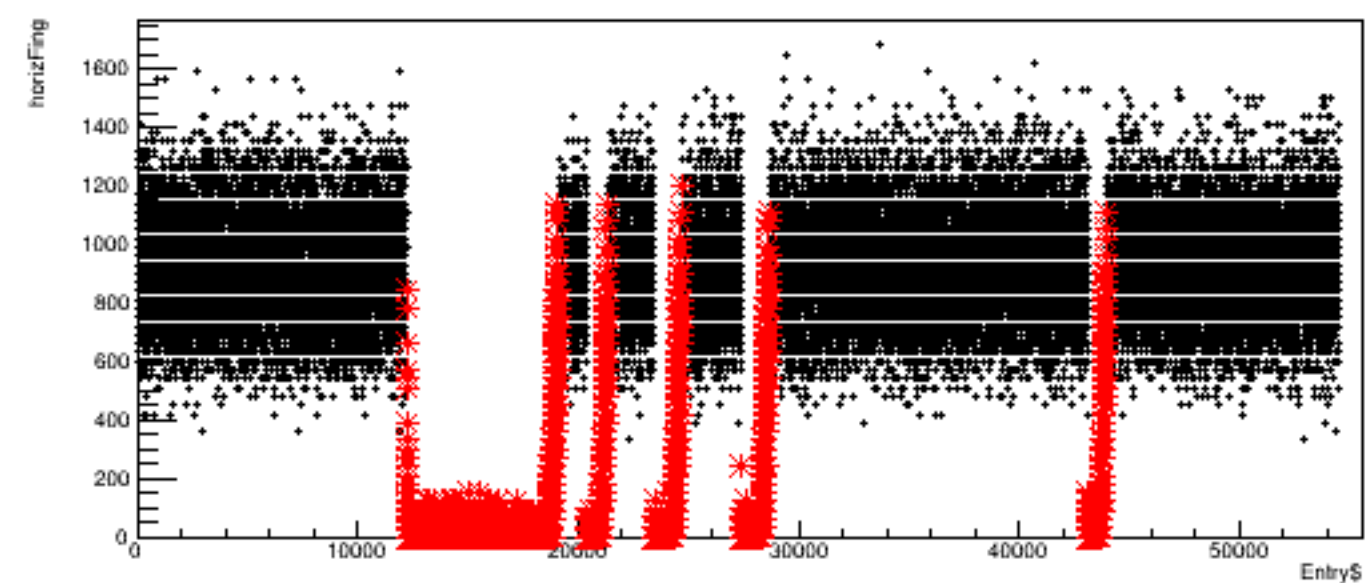
Run 4437, quartetwise: horizFing vs time
