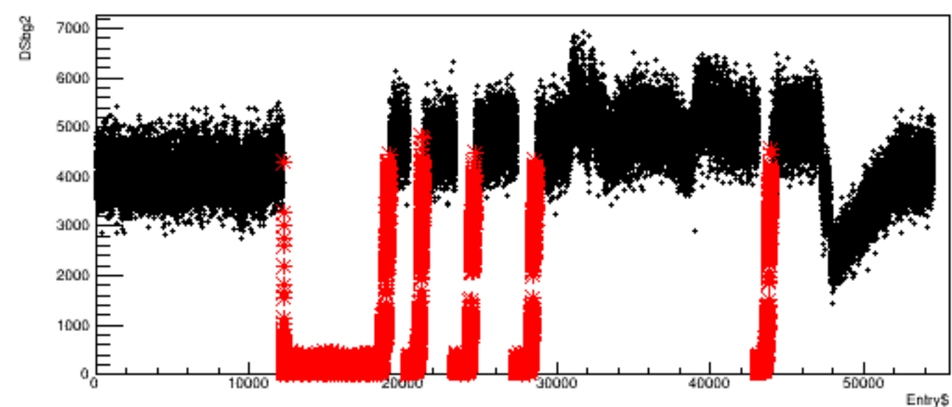
Run 4437, quartetwise: DSbg2 vs time
