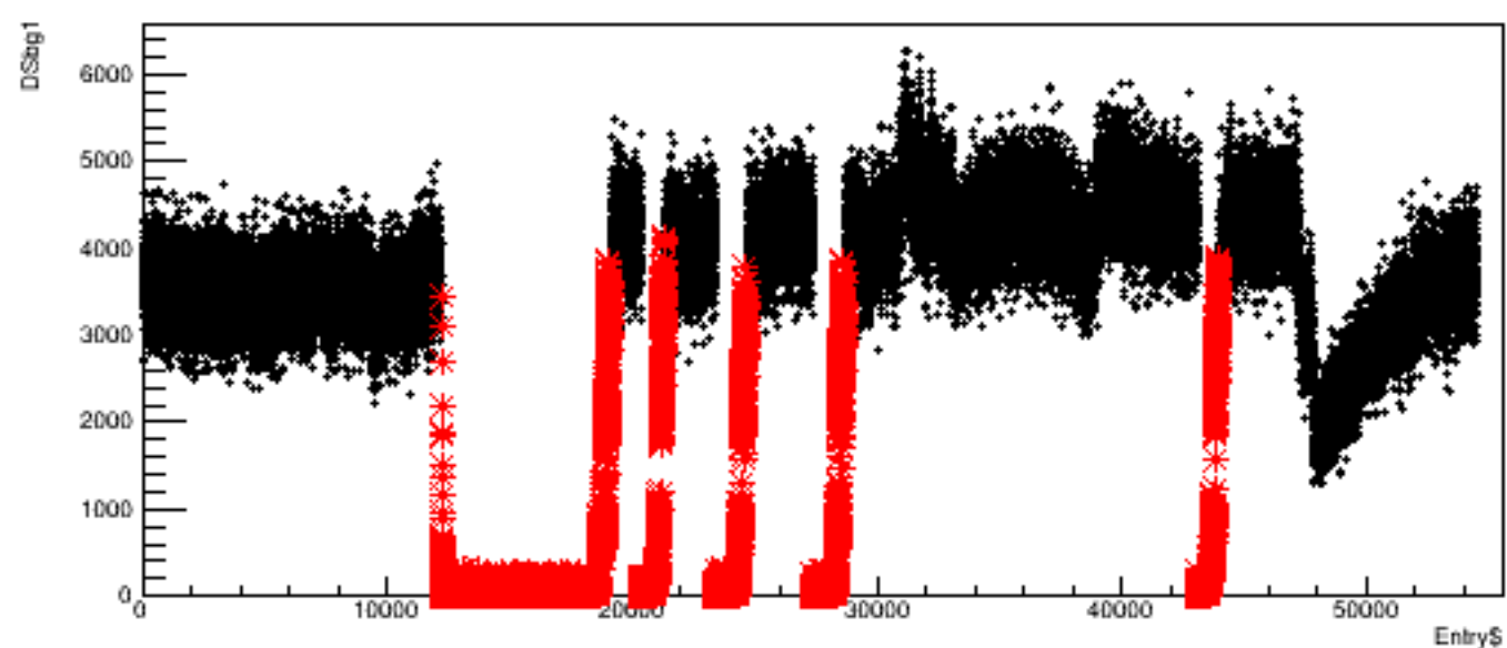
Run 4437, quartetwise: DSbg1 vs time
