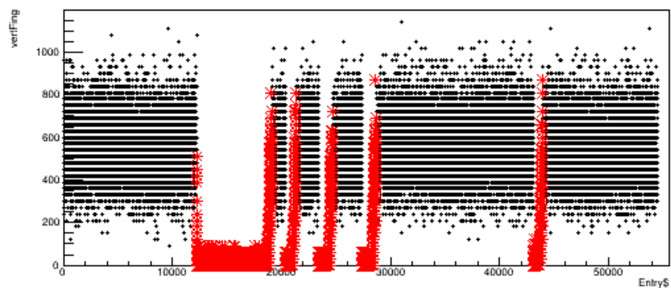
Run 4437, quartetwise: vertFing vs time
