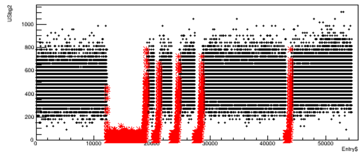
Run 4437, quartetwise: USbg2 vs time
